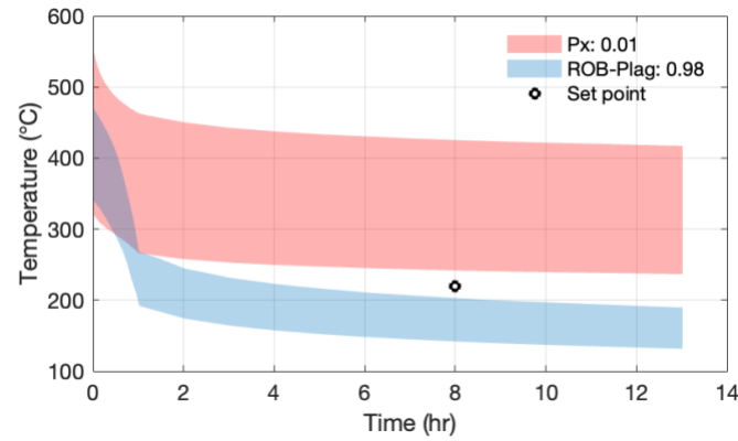
Figure 2 Area of temperature and time combination between the most and least retentive ^3\text{He} mineral phases within pyroxene (red) and plagioclase (blue) for a fractional gas loss of 0.01 and 0.98, respectively. For plagioclase, the temperature-time range is based on the diffusion kinetics determined from grains of the Ferrar Dolerite, ROB-plag (Bergelin et al., 2025). For pyroxene, the range includes diffusion kinetics obtained for grains of Ferrar dolerite pyroxene (LABCO-Px and ROB-Px) and gem-quality pyroxene (GEM-Px) grains (Bergelin et al., 2025). The grain size radius used to determine the diffusion kinetics range from 108-168 \mu\text{m} . Any temperature-time combinations above the blue shade are expected to degas >0.98 , and any combinations below the red shade are expected to degas <0.01 of the total ^3\text{He} in each mineral phase. The area below the red shade and above the blue shade represents the temperature and time field to separate ^3\text{He} released from plagioclase, without releasing ^3\text{He} from pyroxene. The black dot shows the temperature and time combination that we use in this experiment, and is suitable for a standard vacuum oven.
