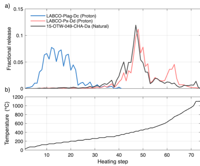
Figure 1 Step heating analysis of proton-irradiated, single grains of Ferrar dolerite plagioclase (blue), pyroxene (red), and naturally cosmic-ray irradiated, crushed Ferrar dolerite containing a mixture of plagioclase and pyroxene grains (black). Each of the three degassing experiments experienced the same heating schedule. (a) shows the fractional release of ^3\text{He} atoms, and (b) shows the temperature reached during each heating step. Note that the duration of each step varies, which is not shown in this figure (Table S1).
