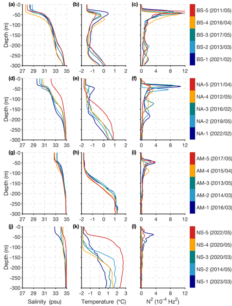
Figure R4. Observed salinity (left column), temperature (middle column) and buoyancy frequency (right column) from observational profiles between 2011 and 2023 in the Arctic Ocean, used as initial profiles in the model simulations. To capture representative characteristics of each region in the Arctic Ocean, these profiles were grouped geographically into four categories: (a)-(c): Beaufort Sea (BS); (d)-(f): North of the Amerasian Basin (NA); (g)-(i): Amundsen Basin (AM); (j)-(l): Nansen Basin (NS). The time of each profile is shown in the color scale at the right-hand side. In order to emphasize the regional differences of the upper stratification, we show only the upper 300m. In fact, in the model we used the upper 700 m of data as the initial field.
