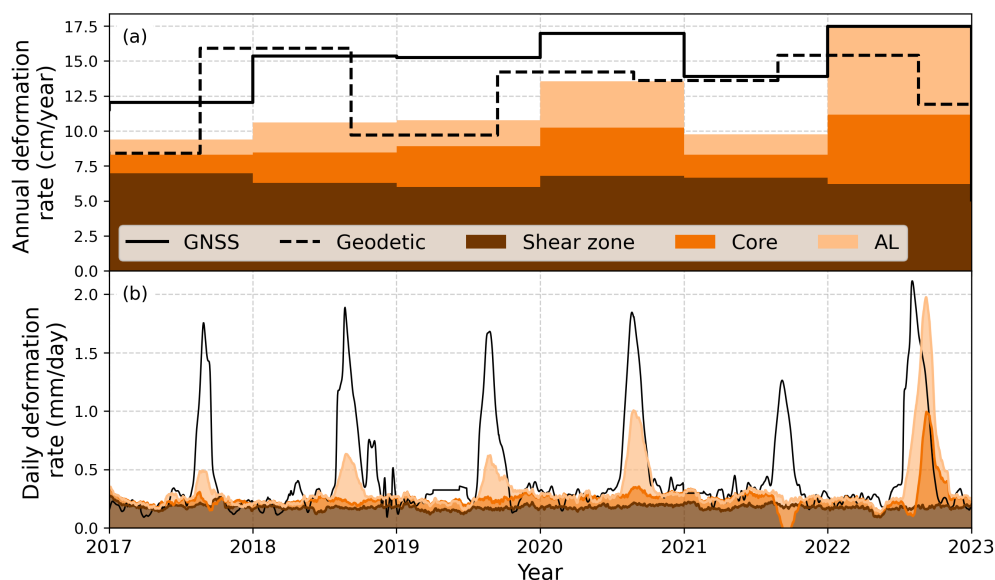
Figure 5. Layer-specific cumulative deformation rates over time: (a) at an annual resolution and (b) at a daily resolution. Measurements are from the borehole, the GNSS station and the geodetic marker (only with an annual resolution).
