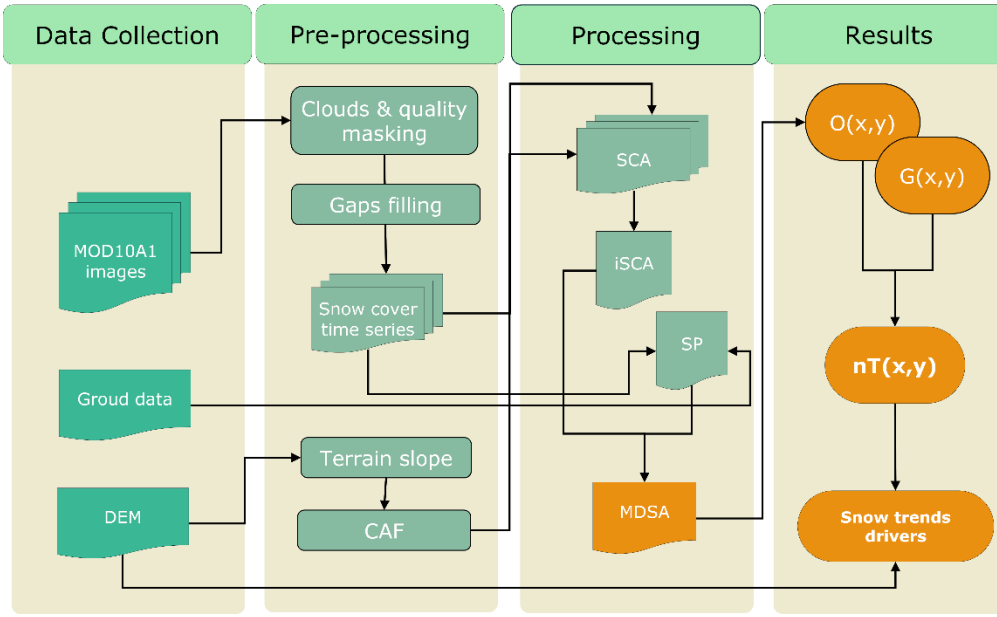
110 Figure 2: Workflow adopted. Arrows represent the data flow from input data (light green) through methodological steps (in dark green) to the obtained results (in orange).
