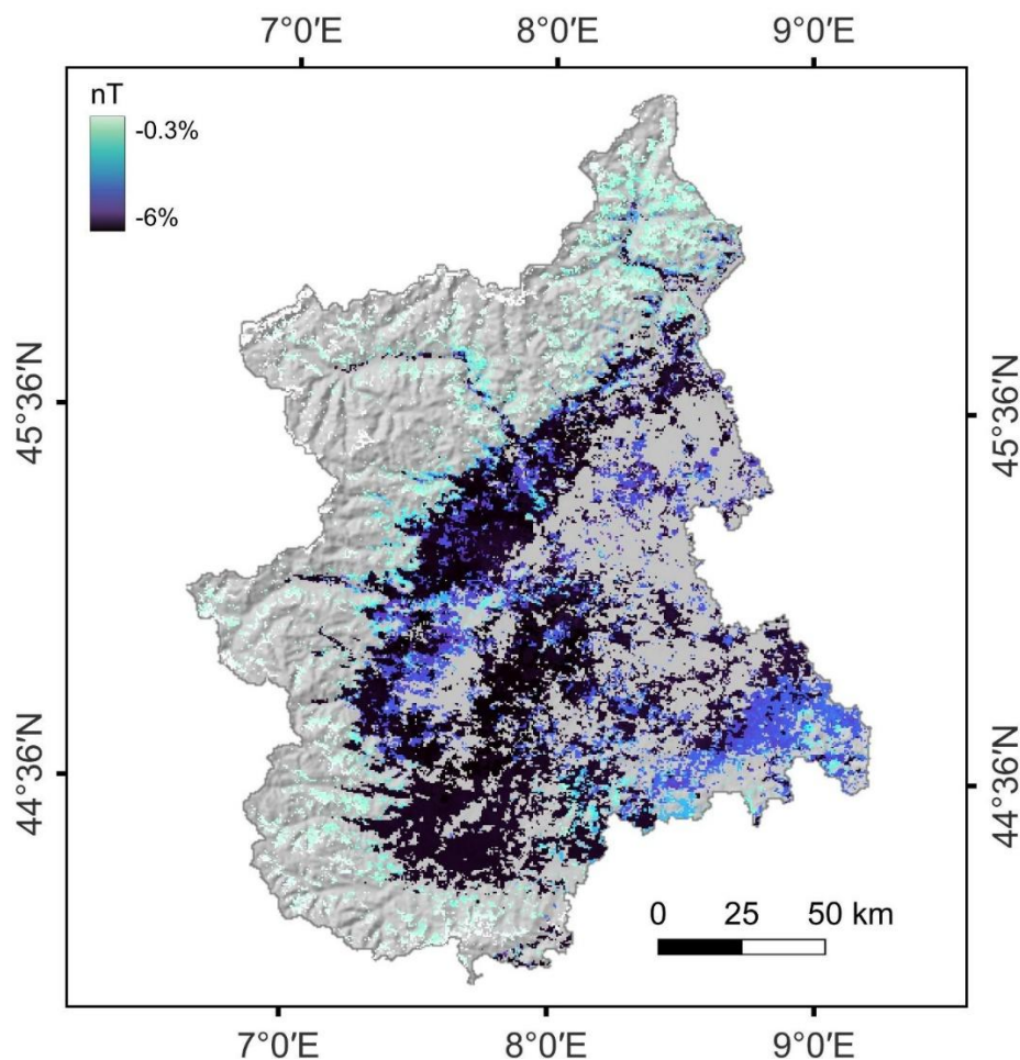
Figure 5: Spatial representation of nT , strongly-negative values are related to low altitude areas, instead of less negative values, related to high altitude areas.
