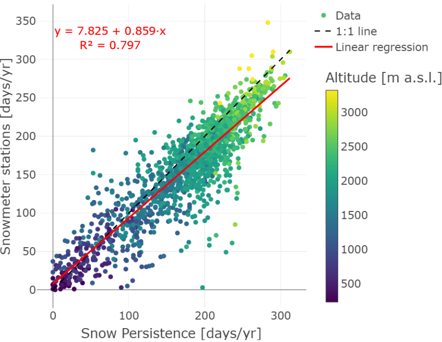
Figure 3: Days of snow persistence calculated by satellite product and ground stations represented in a scatter plot. Dots' colors represent the altitude of the investigated station/pixel. Red line represents the linear regression.
