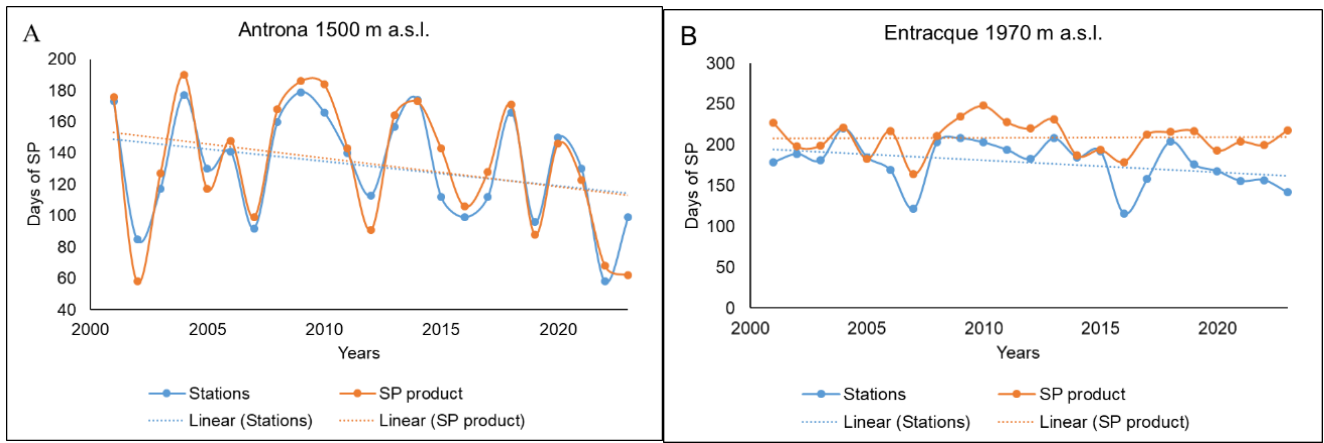
220 Figure 4: yearly snow persistence comparing SP measure calculated from MODIS (orange) and ground snowmeter station (blue). 225 A) Antrona station B) Entracque - Chiotas station. In B the satellite values (orange) are higher than the station ones (blue) 230 underlighting showing a typical case of overestimation of snow presence.
