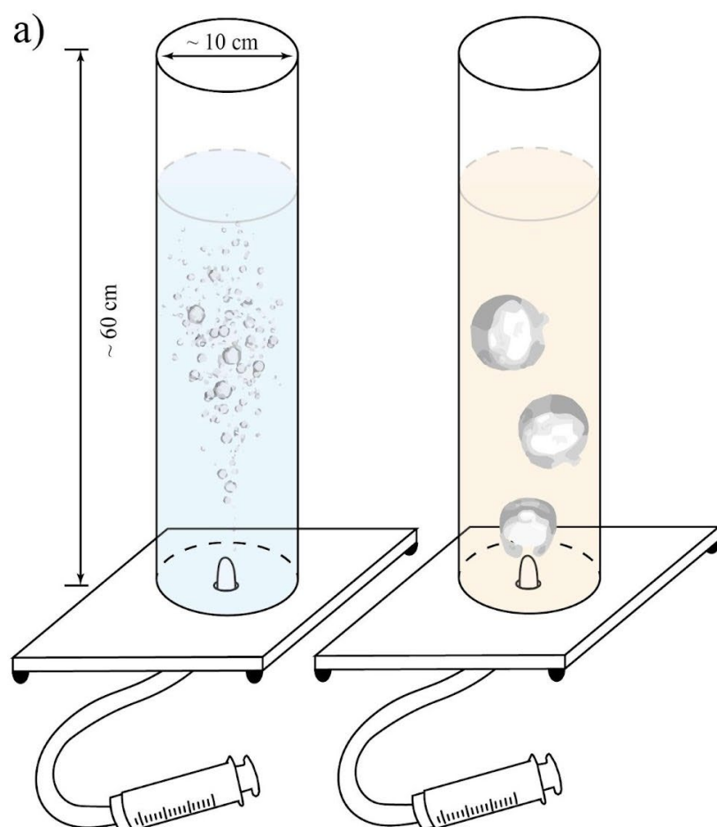
185 Figure 2: a) scheme of the bubble apparatus for both the water- and golden syrup-filled cylinders; b) a picture of the bubble experiment showing the bubble rise. Bubble size is not due to decompression, but rather to differences in the initially injected volume.
