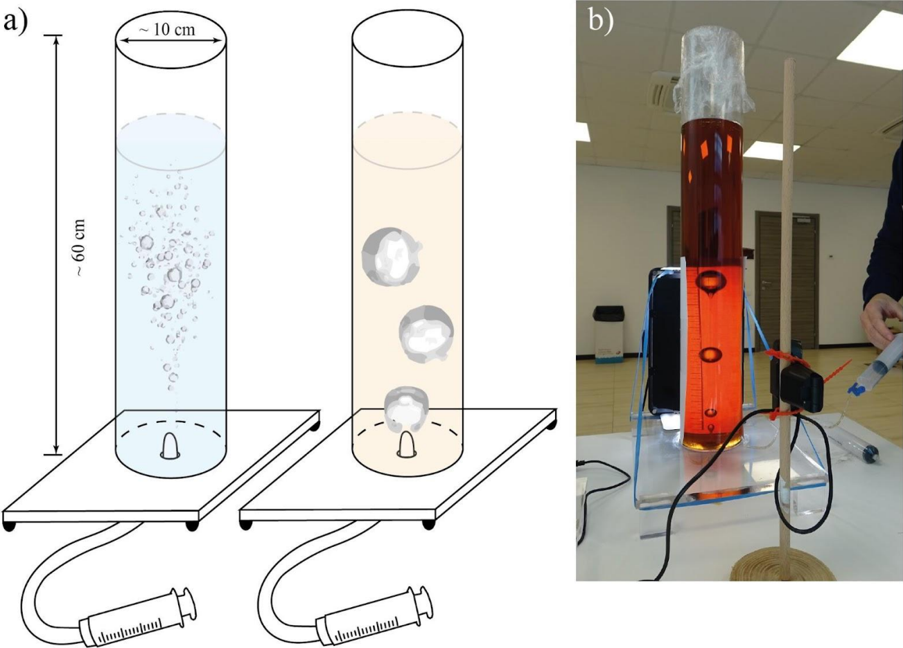
190 Figure 2: a) scheme of the bubble apparatus for both the water- and golden syrup-filled cylinders; b) a picture of the bubble experiment showing the bubble rise. Bubble size is not due to decompression, but rather to differences in the initially injected volume.
