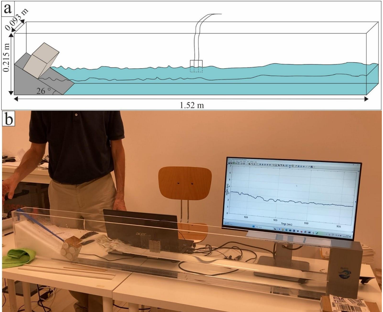
290 Figure 5: a) scheme of the tsunami apparatus showing the rectangular box filled by water, and the different components of the apparatus (inclined plane, rigid block and sensor); b) picture of tsunami experiment.
