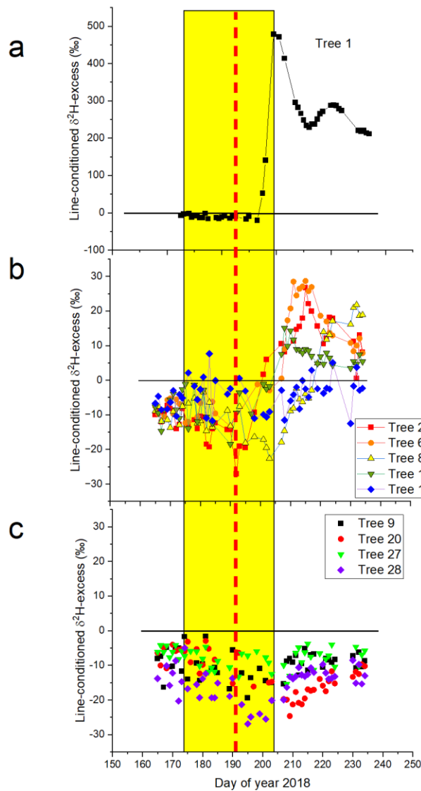
Fig. 5. Line-conditioned deuterium-excess (lc-excess) of xylem water in tree stems. Values above zero, denoted by the horizontal black line, show likely label uptake. Panel a—) Tree 1, near the soil-labelling plot; b—) Labeled trees with lc-excess at some point greater than zero; c—) Unlabeled trees, all more than 4 m from the center of the labelling plot. Note that the y-axes are on different scales and the zero-intercepts are at different locations on panel a vs panels b and c. In all panels, the drought period is shown by the yellow box and the labelling date is shown as a vertical, dashed red line at DOY 191.
