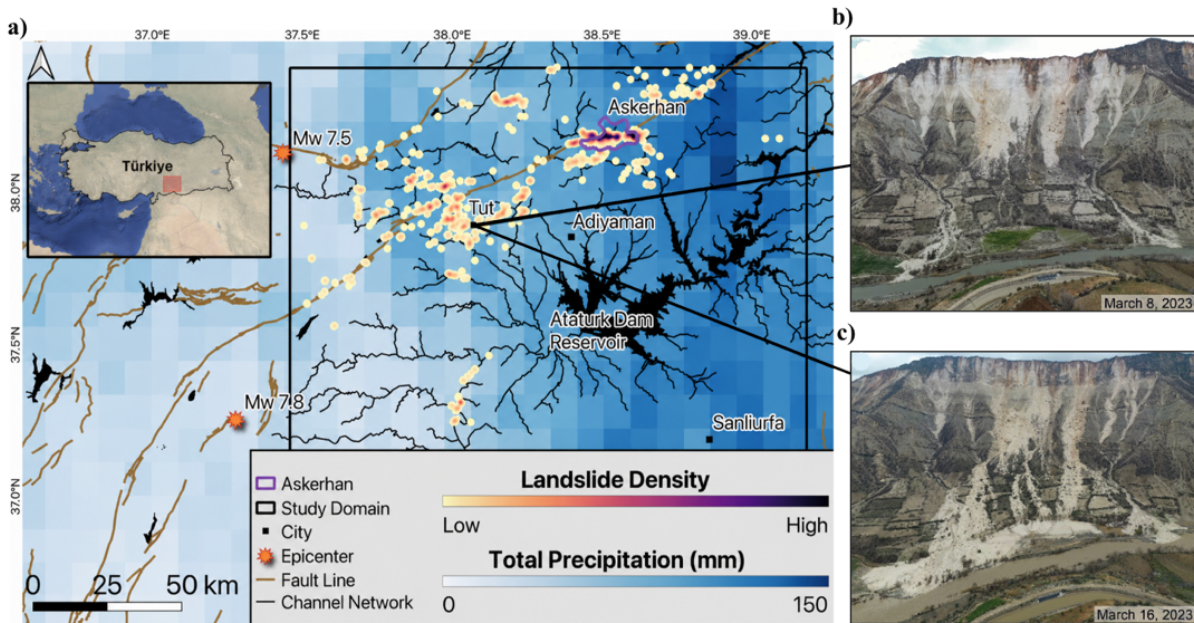
Figure 2: (a) NASA’s Integrated Multi-satellitE Retrievals for GPM (IMERG) precipitation estimates for March 10-16 2023. This atmospheric river swept through the central earthquake impacted area, delivering up to 146.4 mm of rainfall over a 7 day span. Photos captured within the town of Tut illustrate the landscape effects of (b) coseismic driven crown cracking and landsliding and (c) post-seismic storm-driven sedimentation and debris flow (Görüm et al., 2025). A 10 km 2 validation site within the Askerhan
