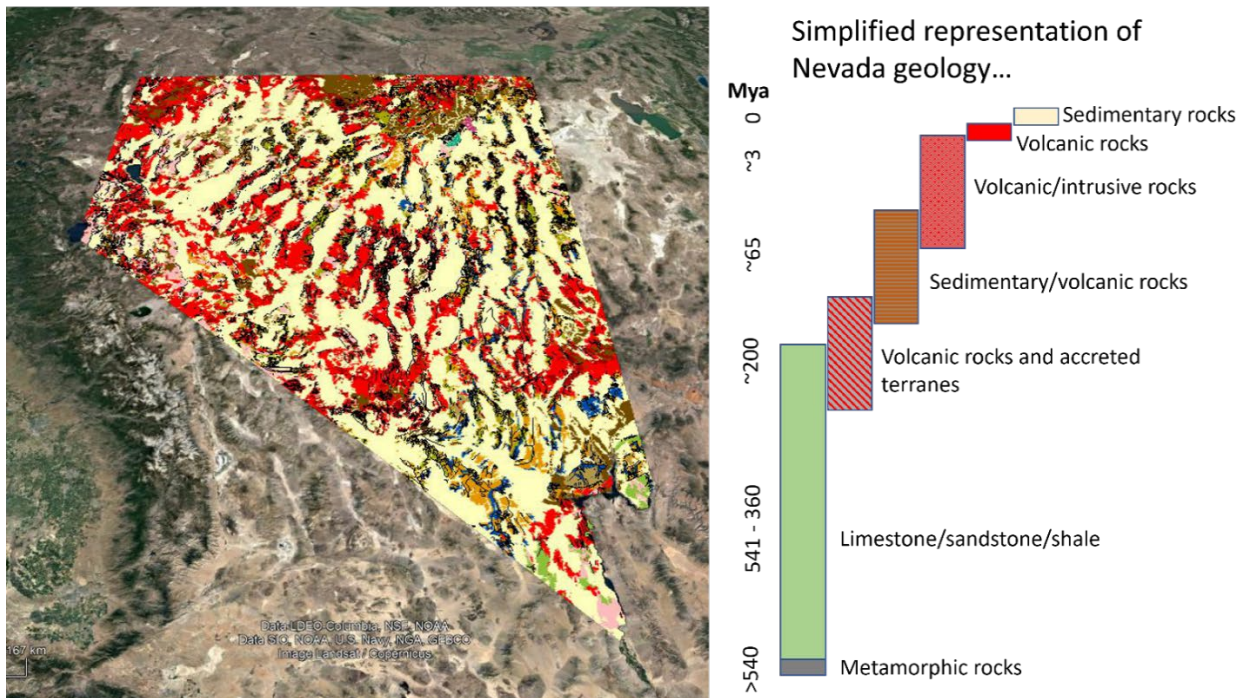
Figure 3. Nevada surficial geology map from Crafford (2007), scale 1:250,000 (left), and simplified representation of Nevada geology (right).
