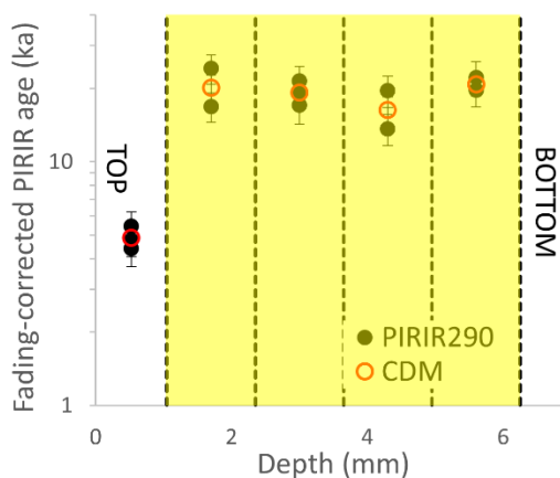
645 Figure 13. Uncorrected (left) and fading-corrected (right) luminescence-depth profiles for volcanic Rocks 11 and 13 from CA21P1. Dashed lines denote slice thickness. Aliquots contain ~125-165 grains each of the 125-250 \mu\text{m} fraction. Yellow shading highlights slices used for plateau age calculations. Black dots are pIRIR290 aliquot ages, X symbols are rejected aliquots, and red hollow circles are CDM weighted mean ages for each slice. The y-axes are plotted on a log scale.
