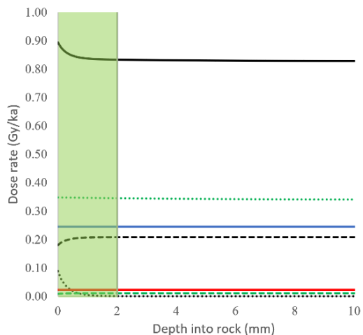
450 Figure 6. Modelled dose rates for limestone rocks from site CV21P1 following the method of Riedesel and Autzen (2020) and radionuclide concentration data obtained from ICP-MS/AES. The average dose rate for the outer ~2 mm of the rocks (green shading) was used for age calculation.
