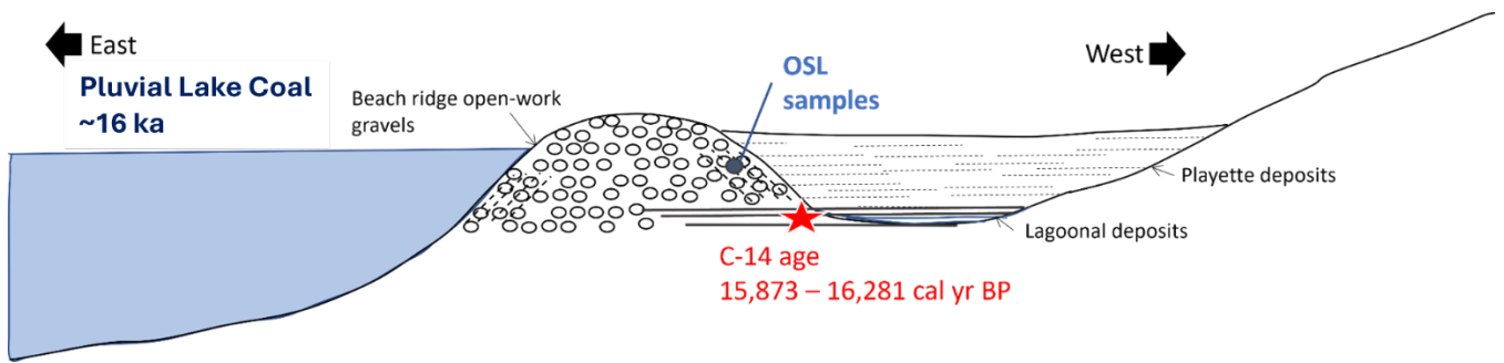
Figure 5. Illustration of sampled beach ridge shortly after formation ~16,000 years ago during the Pluvial Lake Coal highstand. Any backwater playette deposits or lagoonal deposits landward of the beach ridge have since eroded away, exposing the beach gravels on the west side of the ridge. Figure not to scale.
