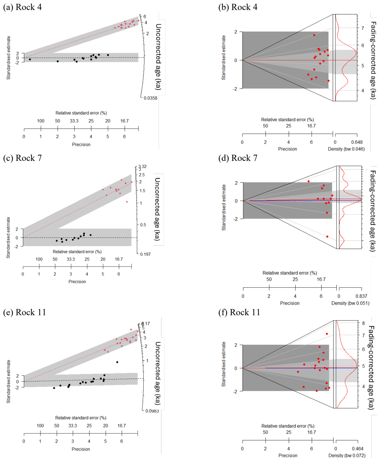
605 Figure 10. Uncorrected (left) and fading-corrected (right) age distributions from polycrystalline grains extracted from the outer ~1 mm layer of volcanic Rocks 4, 7 and 11 (~2500 grains per aliquot, 32-63 \mu\text{m} fraction) from CA21P1 in Cave Valley. Corrections apply the Kars et al. (2008) approach based on the model of Huntley (2006). Black dots are IR50 data (younger age group in each
