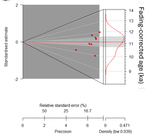
Figure 11. Uncorrected (left) and fading-corrected (right) age distributions from polymineral grains extracted from the outer 1 mm layer of volcanic Rocks 12, 13 and 18 (~2500 grains per aliquot, 32-63 \mu\text{m} fraction) from CA21P1 in Cave Valley. Corrections apply
