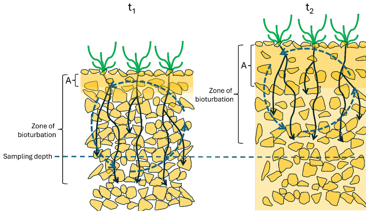
775 Figure 16. Schematic illustrating the accretionary-inflationary mode of soil profile development on the beach ridge at site CA21P1. Initial establishment of an A soil horizon after beach ridge abandonment in the late Pleistocene-early Holocene is shown as “t1”. Increases in dust influx ~8-4 ka (t2) cause accretion of the A horizon and translocation of fines to depth. As the soil surface rises, the zone of bioturbation rises preventing surface clasts reaching the depth of sampling after ~4 ka.
