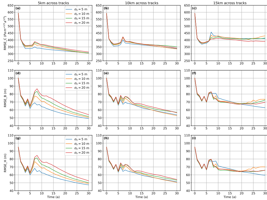
Figure 12. The evolution of ensemble mean RMSEs using different across-track spacing surface elevation with various uncertainties on observations for (a-c) friction coefficient and , (d-f) bed topography, and (g-i) ice thickness under different across-track spacings of surface elevation observations and varying levels of surface elevation uncertainty.
