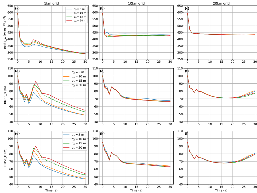
Figure 13. Same as Fig 13, but with using different grid resolution-resolutions for surface elevation observations.
