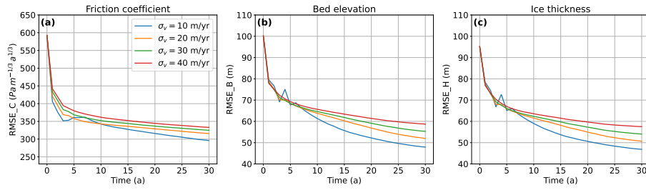
Figure A2. The evolution of mean analysis RMSE for (a) friction coefficient, (b) bed topography, and (c) ice thickness, using full spatial coverage of surface velocity and elevation data (as in the twin experiments), under different levels of uncertainty in surface velocity observations.
