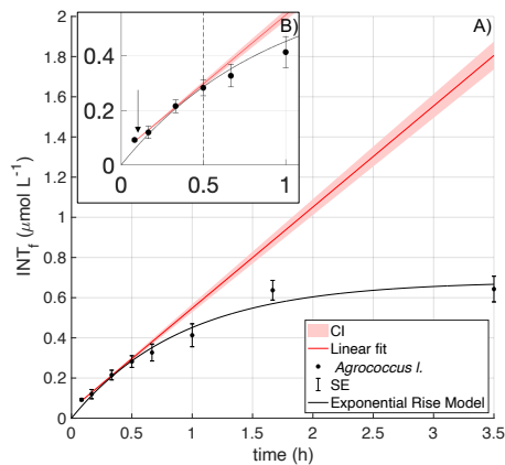
Figure 1. INT toxicity curve of Agrococcus lahaulensis during a time series experiment. A) Average INT_f ( \mu\text{mol L}^{-1} ) and standard error bars (SE; n = 3 ) are presented in black. The red line is the predicted linear fit, the red shading indicates the confidence interval, and the black line denotes the exponential rise model. B) The small top box represents a zoom-in showing toxicity after 30 minutes of incubation (vertical dashed line) and the downwards pointing arrow indicates the calculated experimental incubation time.
