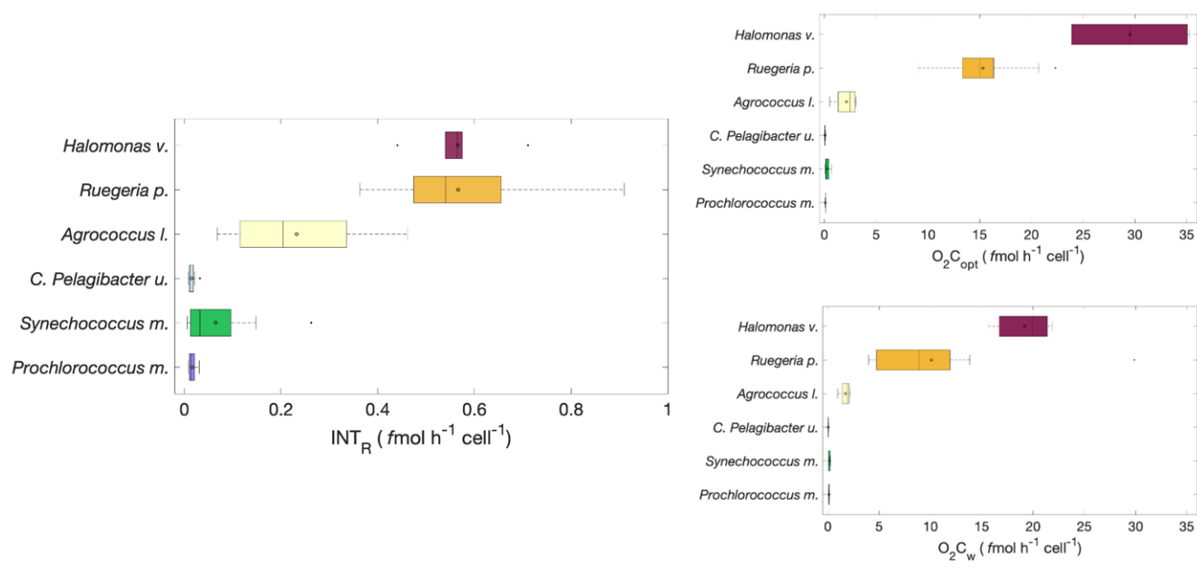
245 Figure 2. Cell specific rates of formazan production ( \text{INT}_R (fmol h -1 cell -1 ) and oxygen consumption ( \text{O}_2\text{C}_{\text{opt}} and \text{O}_2\text{C}_w (fmol h -1 cell -1 )) ; n = 12. of Prochlorococcus marinus , Synechococcus marinus , C. Pelagibacter ubique , Agrococcus lahaulensis , Ruegeria pomeroyi and Halomonas venusta . The boxplot central mark (—) indicates the median, the circle the mean (o), the side edges of the box indicate the 25th and 75th percentiles, respectively, the whiskers (T) extend to the most extreme data points, and the outliers are plotted using the (•) symbol. Copiotrophs are shown with warm colours (dark red, orange, yellow) and oligotrophs with cold colours oligotrophs (cyan, green, violet).
