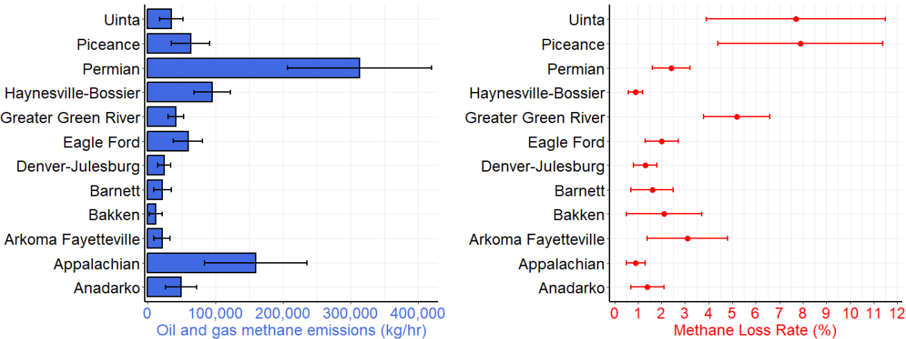
Figure 3: Basin-level oil and gas methane emissions (kg/hr) and gas normalized loss rates (%) estimated from MethaneAIR data. Gas-dominant basins (Appalachian and Haynesville-Bossier) have the lowest loss rates (<1%), whereas low-producing basins with aging infrastructure (Piceance and Uinta) have higher loss rates (>7%).
