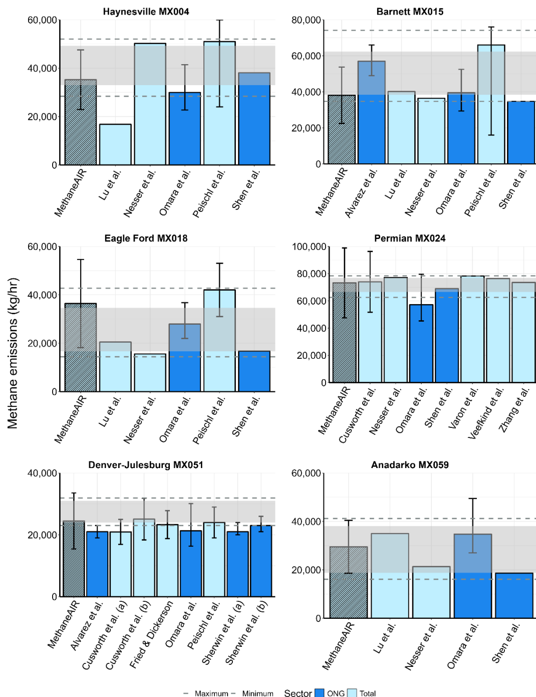
Figure 5: Total methane emissions for six MethaneAIR flights compared to other measurement-based estimates reported in the literature. The grey shaded area and dashed lines show the representative ranges of total methane emissions (95% CI, minimum/maximum) derived from previous literature. The MethaneAIR quantification across different measured basins shows good agreement compared to other measurement-based estimates.
