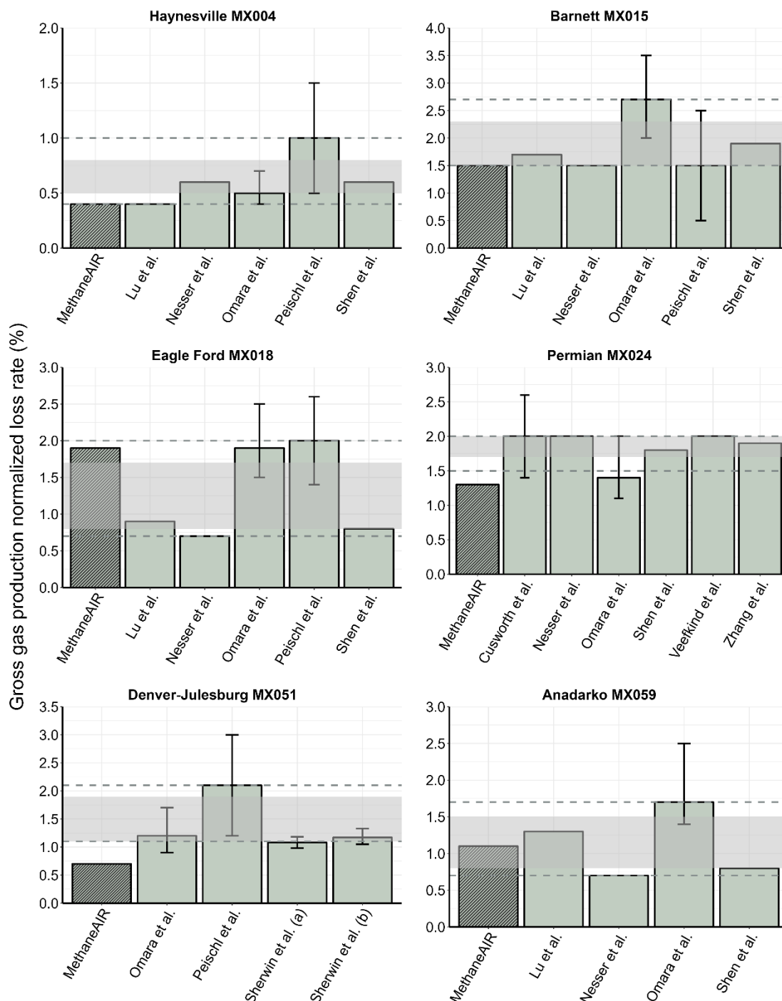
Figure 6: Gross-gas production normalized methane loss rates for six MethaneAIR flights compared to other measurement-based estimates reported in the literature. The grey shaded area and dashed lines show the representative ranges of loss rates (95% CI,
