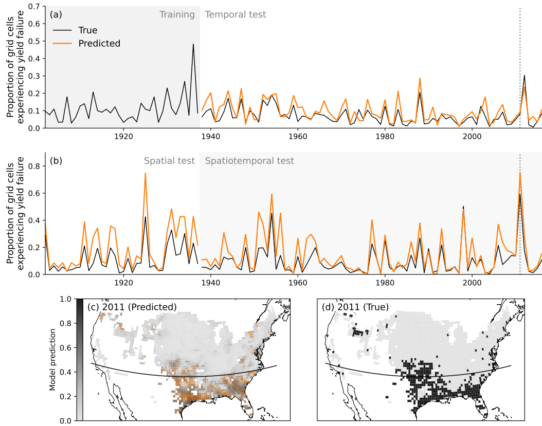
Figure 4. Predictions of a logistic regression model using ten identified pDSSAT drivers on held-out years and regions. (a) True (black) and predicted (orange) proportion of grid cells experiencing yield failure each year over the grid cells used for training (latitudes above 35 degrees), using a threshold of 0.235 to define a yield failure prediction (selected based on achieving the maximal f-score of 0.405 over the training years, which are marked by the grey shaded area). (b) True (black) and predicted (orange) proportion of grid cells experiencing yield failure each year in the held-out grid cells (latitude below 35 degrees). Unshaded years represent the spatial test set (held-out regions during years included in training data) and shaded years represent the spatiotemporal set (held-out regions and years). Model predictions for 2011 are illustrated in panel (c), with orange dots marking grid cells where the prediction exceeds the threshold and therefore yield failure is predicted. The corresponding ground truth is shown in panel (d), with black areas indicating locations experiencing yield failure. The curved line indicates the spatial split used to define the test sets. No data from locations below the line, from any year, is used for identifying drivers or training the model.
