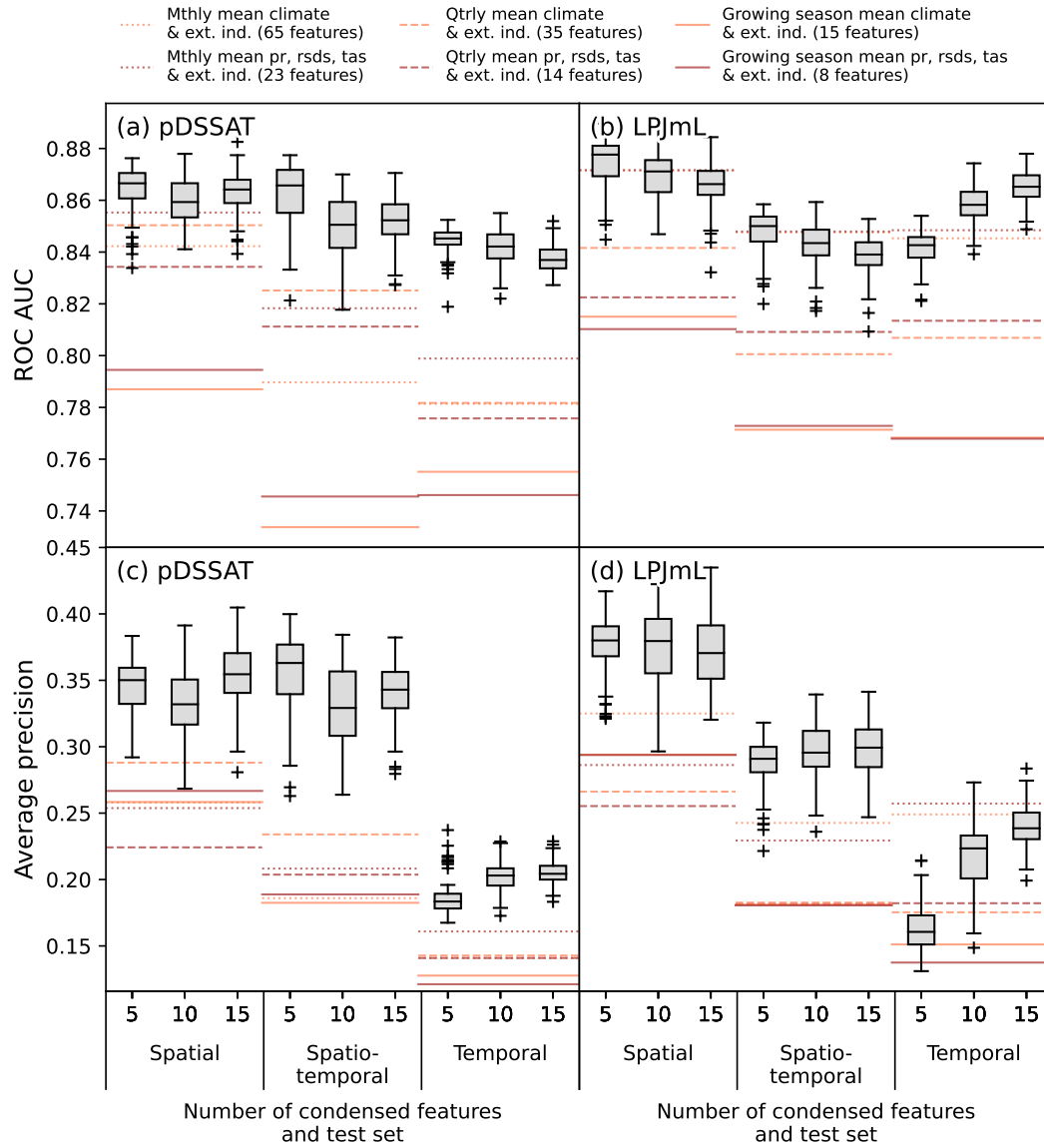
Figure C3. As Fig. 7, when yield failure is defined based on a 5th percentile threshold over the training years.
