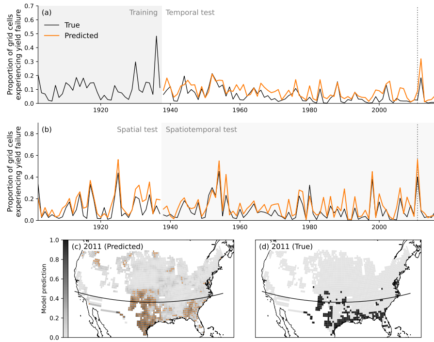
Figure A3. As Fig. 4 but for LPJmL. The threshold used for predicting yield failure years is 0.247, which achieves an f-score on the training set of 0.461.
