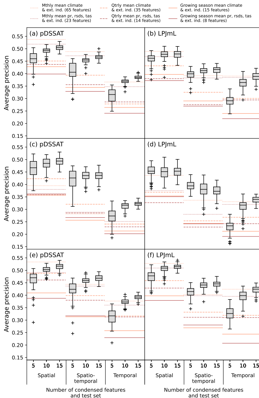
Figure A7. As in Fig. A6 but for average precision (higher is better).
