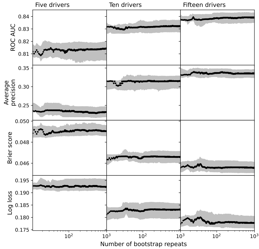
Figure A1. Stability of lasso logistic regression model performance estimates with increasing number of bootstrap repeats, using different numbers of identified climate drivers (columns) as predictive features, and using four different performance metrics (rows). Scores are calculated on the temporal test set, for non-detrended LPJmL. Black lines mark the median score across the repeats and the shaded region indicates the interquartile range.
