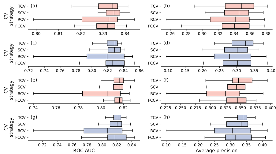
Figure D5. Performance on the test years of Lasso logistic regression models using identified driver sets as predictors, using different cross-validation strategies, based on the parameter sweeps described in Fig. D1. Panels (a) and (b) show results for non-detrended pDSSAT (red); panels (c) and (d) show non-detrended LPJmL (blue); panels (e) and (f) show detrended pDSSAT (red) and panels (g) and (h) show results for detrended LPJmL (blue).
