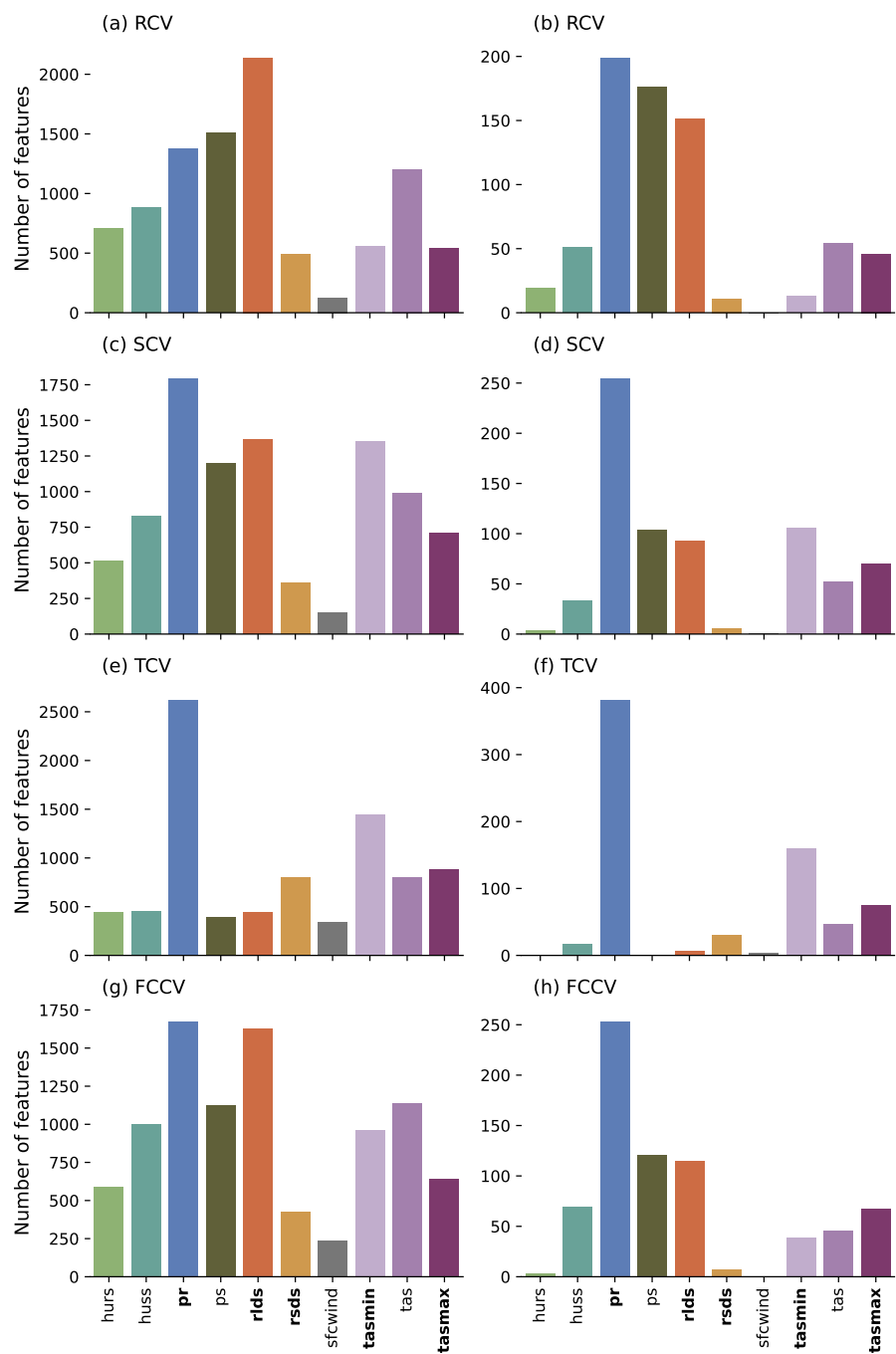
Figure D3. As in Fig. D1, but for pDSSAT with yields detrended.
