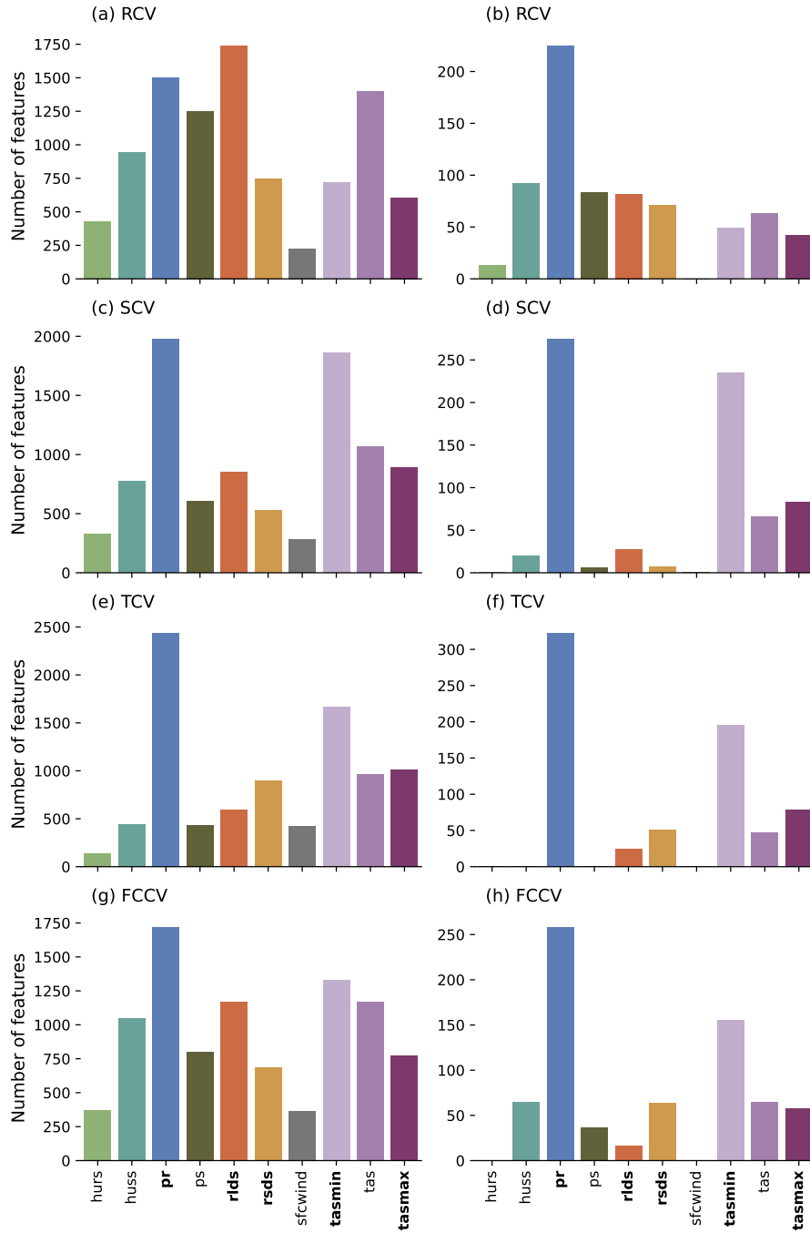
Figure D1. Climate variables used by features selected in Step 2 (a,c,e,g) and in drivers identified in Step 3 (b,d,f,h) for pDSSAT without detrending, depending on cross-validation strategy used to select features: random (RCV), spatial clusters (SCV), temporal (TCV) and feature-based clusters (FCCV). An exhaustive grid parameter sweep is performed (sampling 10, 20 or 30 time intervals in each pool; selecting 10, 20 or 30 features from each pool; and using 5, 10 or 15 cross-validation folds), using 20 pools per unique parameter combination, and sets of 5, 10 and 15 drivers are extracted. Features and drivers resulting from all parameter combinations are grouped by variable and counted.
