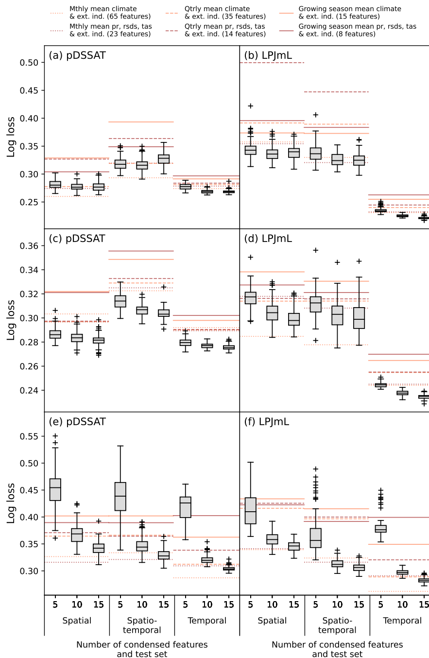
Figure B11. As Fig. A9, when yields are detrended.
