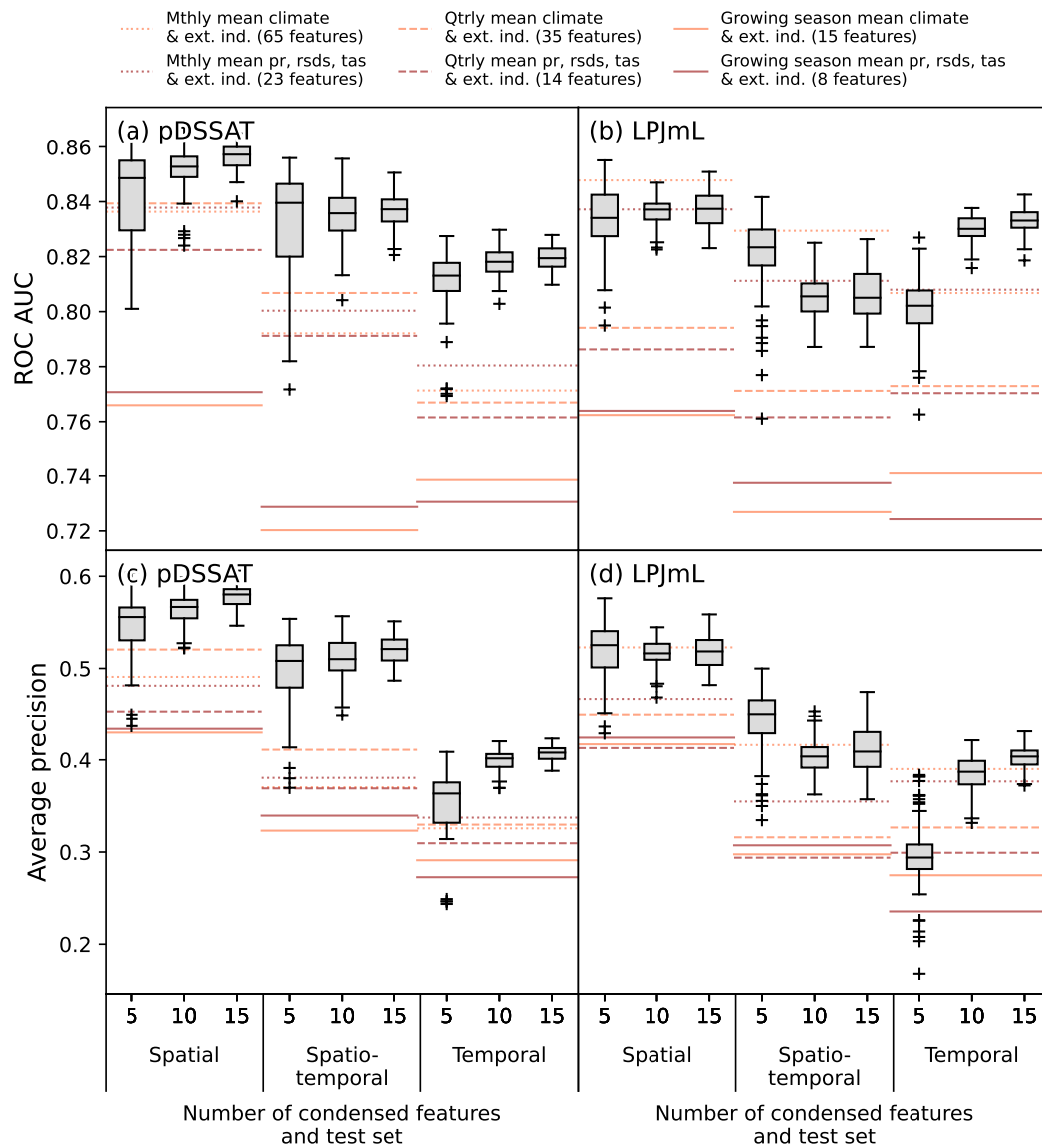
Figure C4. As Fig. 7, when yield failure is defined based on a 15th percentile threshold over the training years.
