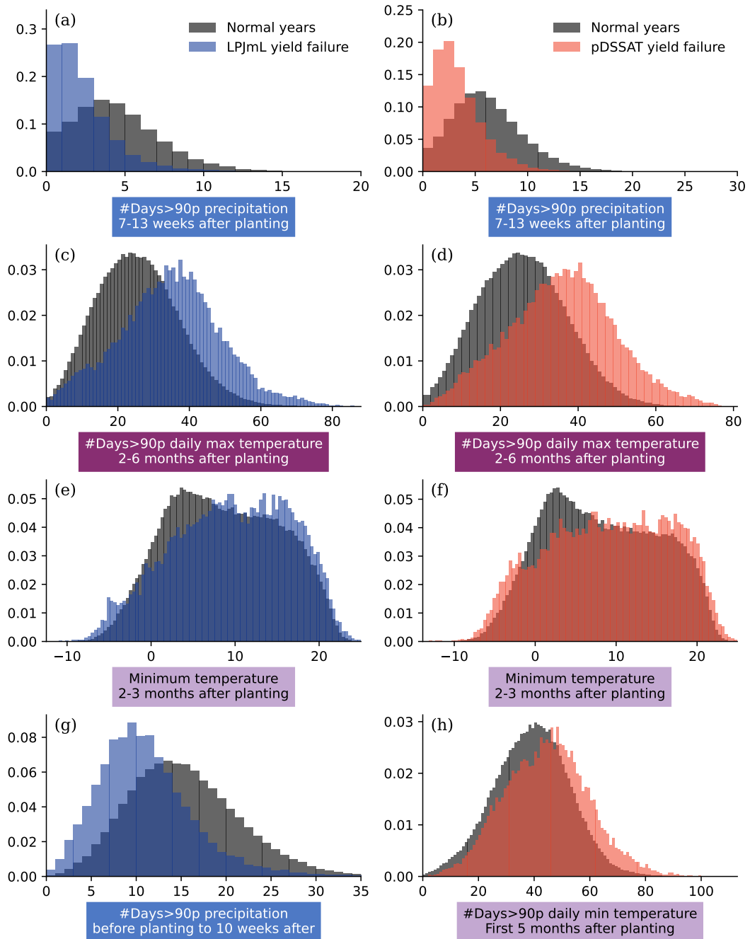
Figure 6. Distributions for normal and yield-failure years of some of the identified climate drivers of maize yield failure shown in Fig. 5, for LPJmL (panels (a), (c), (e) and (g)) and pDSSAT (panels (b), (d), (f) and (h)).
