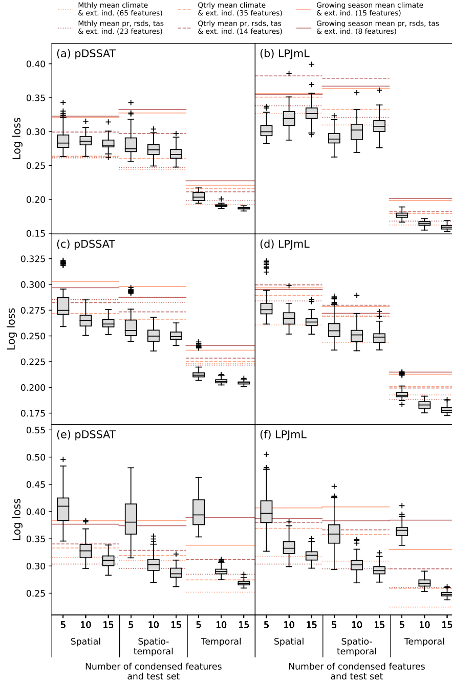
Figure A9. As in Fig. A6 but for log loss (lower is better).
