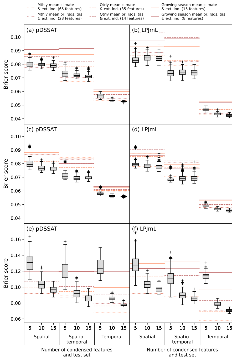
Figure A8. As in Fig. A6 but for Brier score (lower is better).
