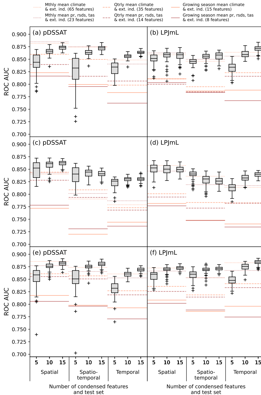
Figure A6. ROC AUC scores on test sets for models trained on training set, using feature sets derived from training set data (higher is better). (a), (c) and (e) show scores for pDSSAT and (b), (d) and (f) show LPJmL. (a) and (b) use LASSO logistic regression and include interaction terms; (c) and (d) use LASSO without interaction terms, (e) and (f) use extra trees.
