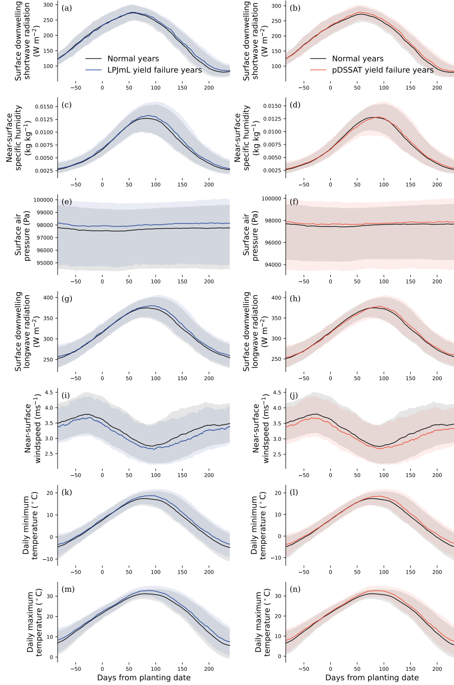
Figure A2. As in Fig. 3, composite plots of the seven-day rolling mean of surface downwelling shortwave radiation, near-surface specific humidity, surface air pressure, surface downwelling longwave radiation, near-surface wind speed, daily minimum temperature, and daily maximum temperature for LPJmL (panels (a), (c), (e), (g), (i), (k), (m)) and pDSSAT (panels (b), (d), (f), (h), (j), (l), (n)) for either normal years or yield failure years, without detrending.
