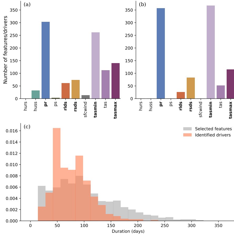
Figure A4. Climate variables used in features selected after Step 2 of our method (a) and in drivers identified from condensing those features in Step 3 (b), for pDSSAT without detrending. Bold text indicates variables used as input by the crop model: precipitation ( pr , mm), surface downwelling longwave radiation ( rlds , \text{Wm}^{-2} ) and shortwave radiation ( rsds , \text{Wm}^{-2} ), daily minimum ( tasmin , ^{\circ}\text{C} ) and maximum near-surface air temperature ( tasmax , ^{\circ}\text{C} ). Not used by the crop model are near-surface relative humidity ( hurs , %), near-surface specific humidity ( huss , \text{kgkg}^{-1} ), surface air pressure ( ps , Pa), near-surface windspeed ( sfcwind , \text{ms}^{-1} ) and mean daily near-surface air temperature ( tas , ^{\circ}\text{C} ). However, pDSSAT does use minimum and maximum daily temperatures which are then downscaled to hourly values. The density histogram in panel (c) shows the duration in days of the resulting features or drivers at each stage.
