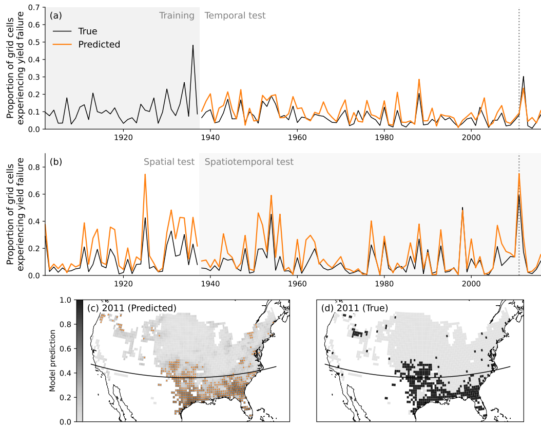
Figure 4. Temporal and spatial predictions Predictions of a logistic regression model using ten identified pDSSAT drivers on held-out years and regions . (a) True (black) and predicted (orange) proportion of grid cells experiencing yield failure each year over the grid cells used for training (latitudes above 35 degrees), using a threshold of 0.235 to define a yield failure prediction (selected based on achieving the maximal f-score of 0.405 over the training years, which are marked by the grey shaded area). (b) True (black) and predicted (orange) proportion of grid cells experiencing yield failure each year in the held-out grid cells (latitude below 35 degrees). Unshaded years represent the spatial test set (held-out regions during years included in training data) and shaded years represent the spatiotemporal set (held-out regions and years) . Model predictions for 2011 are illustrated in panel (c), with orange dots marking grid cells where the prediction exceeds the threshold and therefore yield failure is predicted. The corresponding ground truth is shown in panel (d), with black areas indicating locations experiencing yield failure. The curved line indicates the spatial split used to define the test sets. No data from locations below the line, from any year, is used for identifying drivers or training the model.
