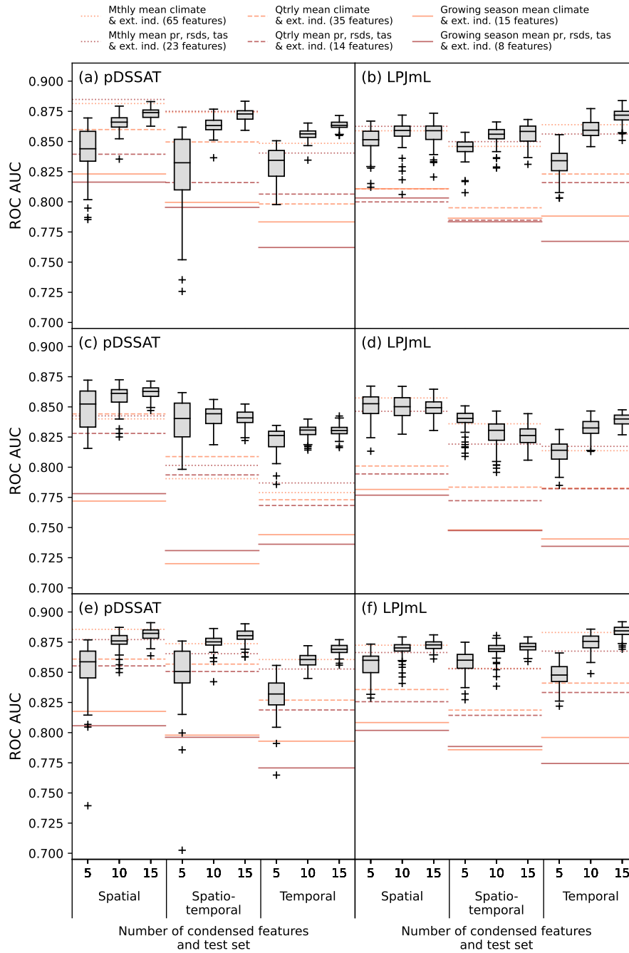
Figure A5. ROC AUC scores on test set-sets for models trained on training set, using feature sets derived from training set data (higher is better). (a), (c) and (e) show scores for pDSSAT and (b), (d) and (f) show LPJmL. (a) and (b) use LASSO logistic regression and include interaction terms; (c) and (d) use LASSO without interaction terms, (e) and (f) use extra trees.
