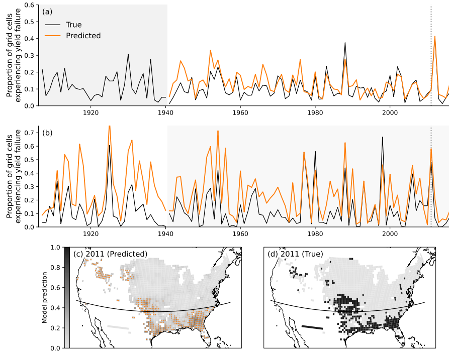
Figure B3. As Fig. 4, for pDSSAT after yields are detrended by removing the seven-year rolling average. The model achieves a ROC AUC of 0.82 0.80 , average precision of 0.35 0.32 , Brier score of 0.08 and log loss of 0.28 over-on the temporal test periodset , a ROC AUC of 0.85 , average precision of 0.43 , Brier score of 0.08 and log loss of 0.28 on the spatial test set, and a ROC AUC of 0.83 , average precision of 0.42 , Brier score of 0.09 and log loss of 0.31 on the spatiotemporal test set. The threshold used for predicting yield failure years is 0.19 0.194 , which results in an f-score on the training years-set of 0.40 0.382 . The Pearson correlation of predicted and true annual proportions of grid cells experiencing yield failure is 0.85 0.79 on the temporal test set and also 0.79 on the spatiotemporal test set.
