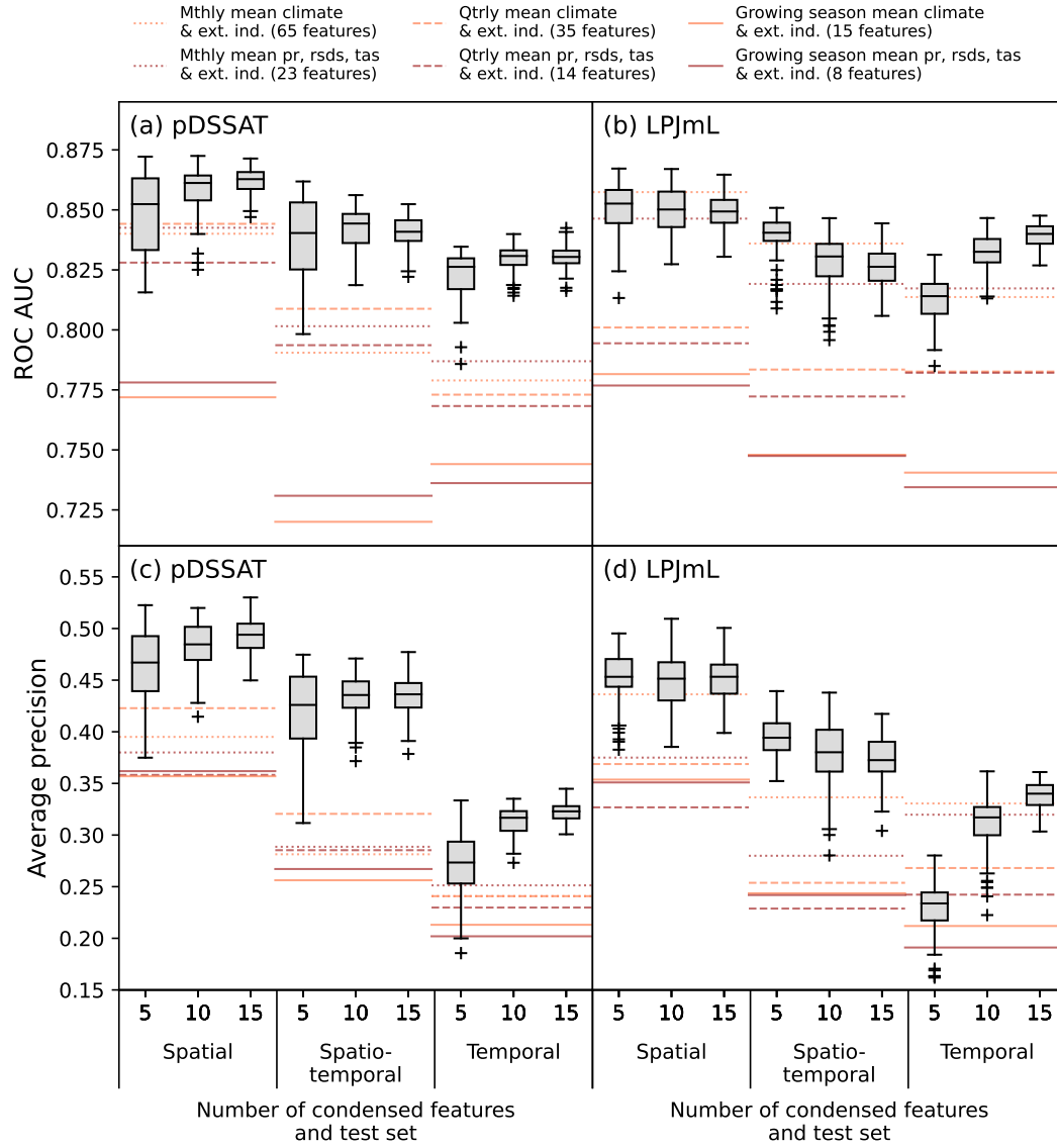
Figure 7. Comparison of the spatial, spatiotemporal and temporal test-set performance of Lasso models for pDSSAT ((a) and (c)) and LPJmL ((b) and (d)). Box plots show the scores for models using sets of five, ten or fifteen drivers using our proposed method, and horizontal lines denote the scores for the same models using baseline feature sets as predictors (made up of mean aggregate climate variables over the growing season or in monthly/quarterly intervals as well as five extreme indicators).
