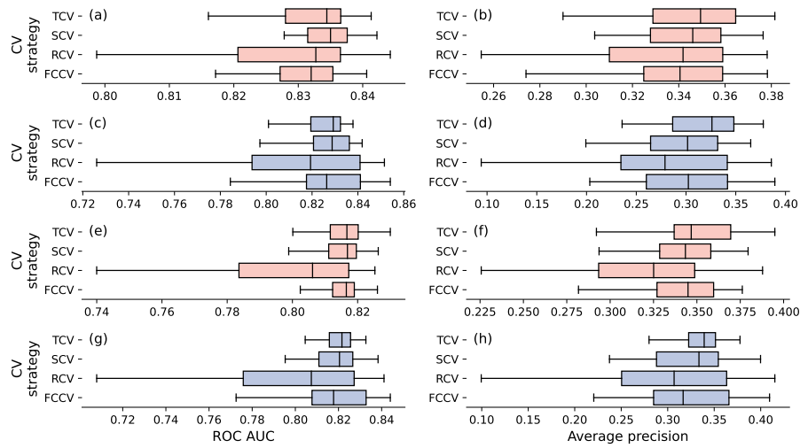
Figure C5. Performance on the test years of Lasso logistic regression models using identified driver sets as predictors, using different cross-validation strategies, based on the parameter sweeps described in Fig. C1. Panels (a) and (b) show results for non-detrended pDSSAT (red); panels (c) and (d) show non-detrended LPJmL (blue); panels (e) and (f) show detrended pDSSAT (red) and panels (g) and (h) show results for detrended LPJmL (blue).
