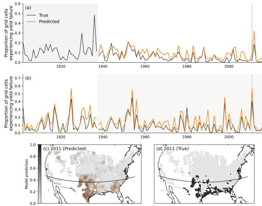
Figure A2. As Fig. 4 but for LPJmL. The threshold used for predicting yield failure years is 0.2250.247 , which achieves an f-score on the training years-set of 0.4710.461 .
