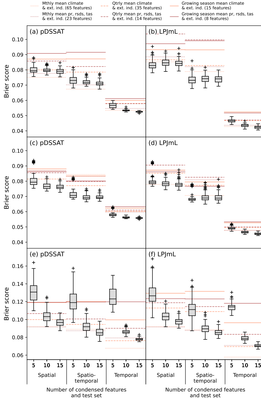
Figure A7. As in Fig. A5 but for Brier score (lower is better).
