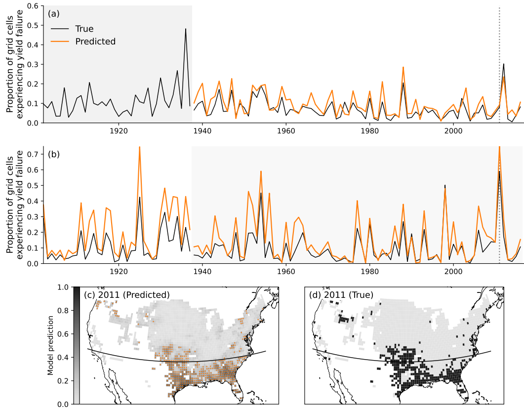
Figure 4. Temporal and spatial predictions of a logistic regression model using ten identified pDSSAT drivers. (a) True (black) and predicted (orange) proportion of grid cells experiencing yield failure each year over the grid cells used for training (latitudes above 35 degrees) , using a threshold of 0.243-0.235 to define a yield failure prediction (selected based on achieving the maximal f-score of 0.438-0.405 over the training years, which are marked by the grey shaded area). The dashed vertical line denotes the (b) True (black) and predicted (orange) proportion of grid cells experiencing yield failure each year in which the highest average precision is achieved, 2011, held-out grid cells (latitude below 35 degrees) . Model predictions for this year 2011 are illustrated in panel (bc), with orange dots marking grid cells where the prediction exceeds the threshold and therefore yield failure is predicted. The corresponding ground truth is shown in panel (ed), with black areas indicating locations experiencing yield failure. Similarly, the dotted vertical line in panel (a) marks the year in which the lowest average precision is achieved (1992), and the corresponding model predictions and ground truth for this year are shown in panels (d) and (c) respectively.
