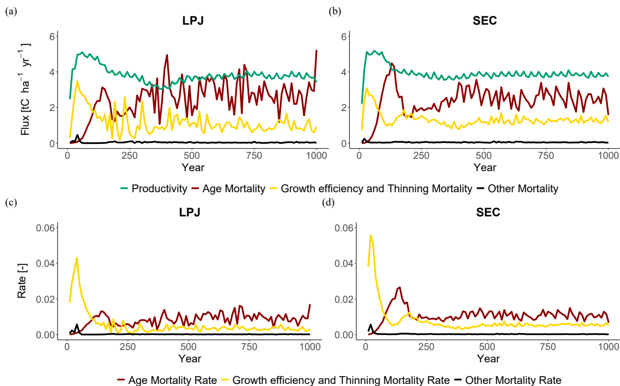
Figure 5. Mortality fluxes (top) and rates (bottom) at BCI. Productivity refers to woody biomass growth, while mortality fluxes indicate the loss of woody biomass from the stand to the litter pool.
