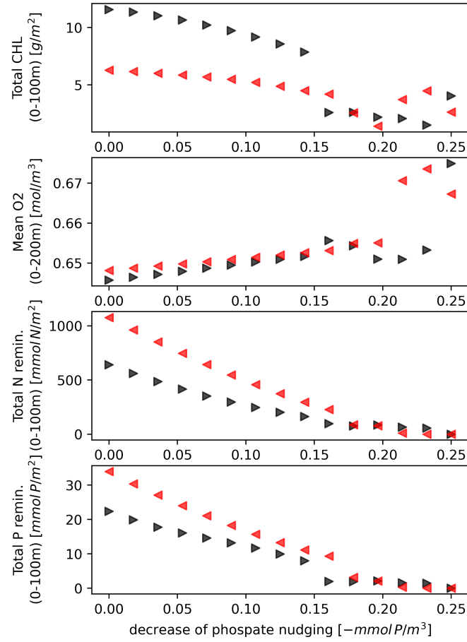
Fig. S6. Bifurcation diagrams under the variation of phosphate nudging forcing in the EXP-SEQ experimental setup for the dynamic regimes associate with annual production and recycling: total chlorophyll produced each year in the first 100m, the total dissolved oxygen present in the first 200m produced each year, the total ammonium (N) remineralized in the first 100m each year and the total phosphate (P) remineralized in the first 100m each year. The black triangles stand for the simulation which follows the x-axis values with time, the red triangles the simulation which goes backwards.
