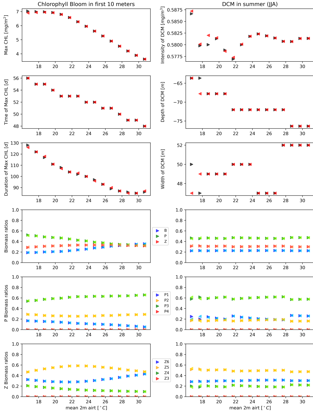
Fig. S3. Bifurcation diagrams for the dynamic regimes associated to Chlorophyll bloom (left panels) and DCM (right panels) under the variation of the air temperature forcing in the EXP-SEQ experimental setup. For each column, in the first three panels from the top the black triangles stand for the simulations which follow the x-axis values with time (forward), the red triangle the simulations which go backwards. For each column, in the first three panels from the bottom the darker coloured triangles stand for the simulations which follow the x-axis values with time, the lighted coloured triangles the simulations which go backwards, e.g. blue goes forward and light blue goes backward.
