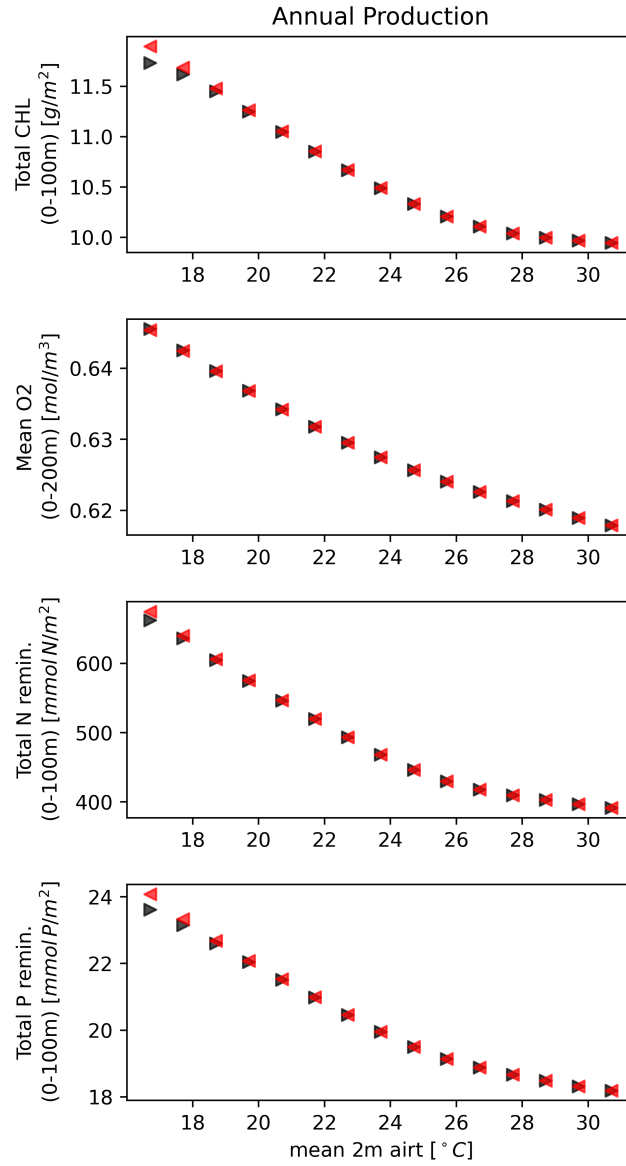
Fig. S4. Bifurcation diagrams under the variation of air temperature forcing in the EXP-SEQ experimental setup for the dynamic regimes associate with annual production and recycling: total chlorophyll produced each year in the first 100m, the total dissolved oxygen present in the first 200m produced each year, the total ammonium (N) remineralized in the first 100m each year and the total phosphate (P) remineralized in the first 100m each year. The black triangles stand for the simulation which follows the x-axis values with time, the red triangles the simulation which goes backwards.
