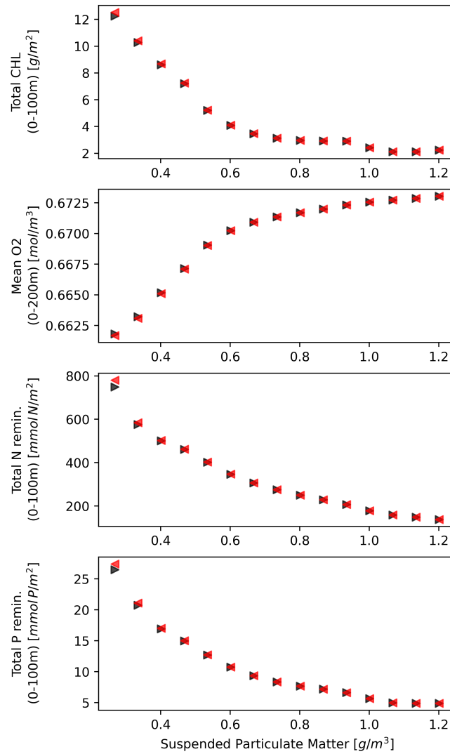
Fig. S8. Bifurcation diagrams under the variation of suspended particulate matter (SPM) forcing in the EXP-SEQ experimental setup for the dynamic regimes associate with annual production and recycling: total chlorophyll produced each year in the first 100m, the total dissolved oxygen present in the first 200m produced each year, the total ammonium (N) remineralized in the first 100m each year and the total phosphate (P) remineralized in the first 100m each year. The black triangles stand for the simulation which follows the x-axis values with time, the red triangles the simulation which goes backwards.
