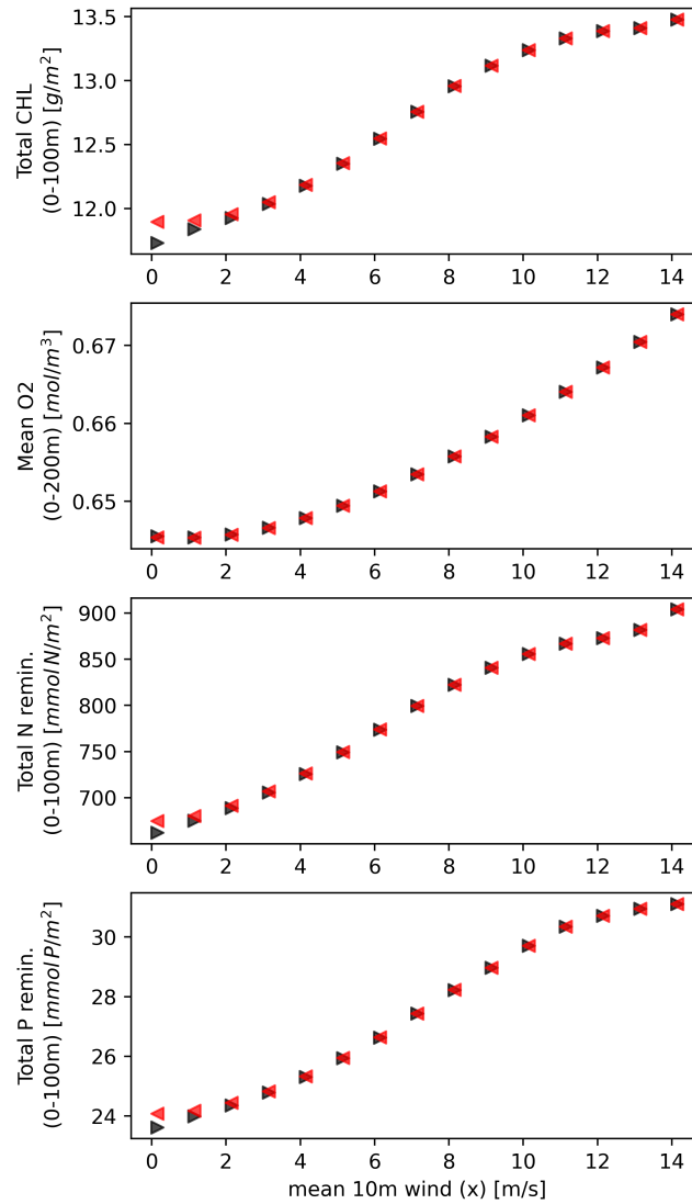
Fig. S2. Bifurcation diagrams under the variation of wind forcing in the EXP-SEQ experimental setup for the dynamic regimes associate with annual production and recycling: total chlorophyll produced each year in the first 100m, the total dissolved oxygen present in the first 200m produced each year, the total ammonium (N) remineralized in the first 100m each year and the total phosphate (P) remineralized in the first 100m each year. The black triangles stand for the simulation which follows the x-axis values with time, the red triangles the simulation which goes backwards.
