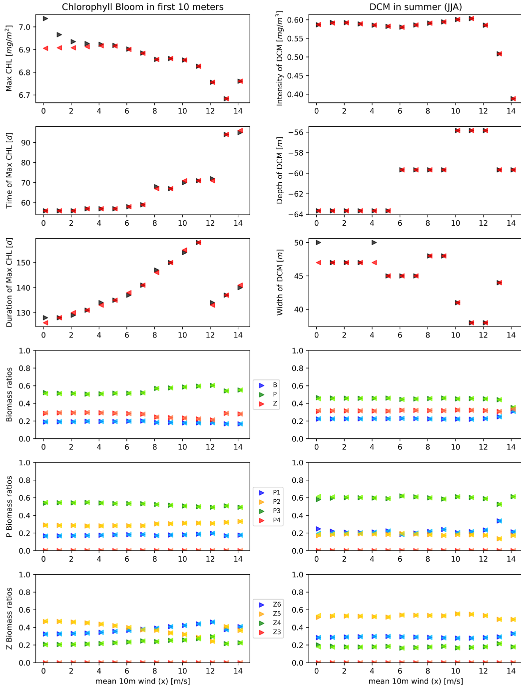
Fig. S1. Bifurcation diagrams for the dynamic regimes associated to Chlorophyll bloom (left panels) and DCM (right panels) under the variation of the wind forcing in the EXP-SEQ experimental setup. For each column, in the first three panels from the top the black triangles stand for the simulations which follow the x-axis values with time (forward), the red triangle the simulations which go backwards. For each column, in the first three panels from the bottom the darker coloured triangles stand for the simulations which follow the x-axis values with time, the lighted coloured triangles the simulations which go backwards, e.g. blue goes forward and light blue goes backward.
