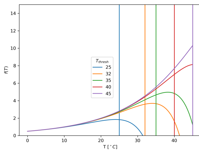
Fig. S11. Plot of the regulation function of temperature on metabolic rates (Eq. (4)). The value of the threshold temperature T_{thresh} set the flex of the function.
