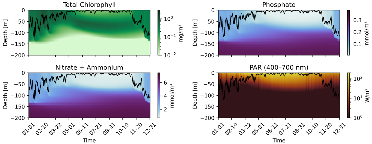
Figure 1. Hovmöller plots of oceanographic variables at the BOUSSOLE site for a climatological year, obtained from model outputs. Each panel shows the temporal evolution along the top 200 m of the water column: (a) Total Chlorophyll [ mg\,m^{-3} ], (b) Phosphate [ mmol\,m^{-3} ], (c) Nitrate + Ammonium [ mmol\,m^{-3} ], and (d) Photosynthetically Active Radiation (PAR, 400–700 nm) [ W\,m^{-2} ]. The black line in each panel represents the mixed layer depth (MLD).
