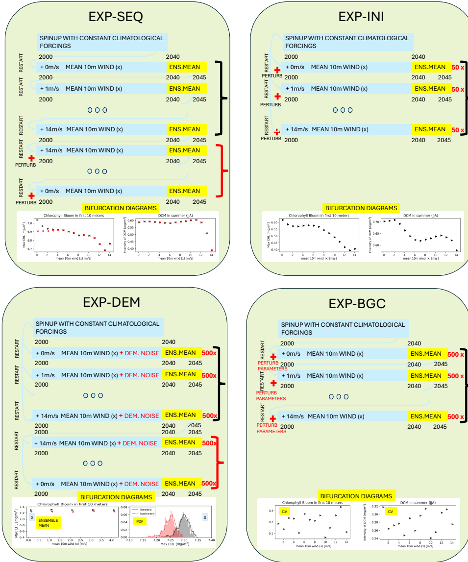
Figure 3. Protocols of the simulation experiments EXP-SEQ, EXP-INI, EXP-DEM, and EXP-BGC. The experiments methodology is described in Sect.2.4. For each EXP we considered the effects of the perturbation of the 6 environmental forcings, listed in Tab.1, over all the target indicators, listed in Tab.2. Here the forcing 10m wind (x) is taken as an example.
