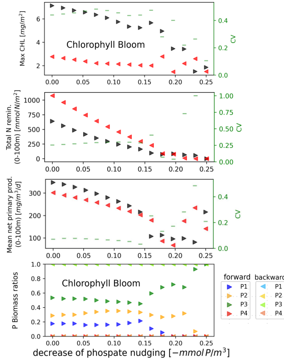
Figure 5. EXP-SEQ setup: Bifurcation diagrams showing the hysteretical response of the model's dynamic regimes associated to seasonal properties (top row), cycling (second row), annual production (third row) and community composition (bottom row) to phosphate nudging. The mean magnitude of the environmental forcings (x-axis) goes from its original value (left) to extreme values (right). The panels show the hysteresis, the forward path (black), from original to extreme environmental condition, and the backward path (red), from extreme to original environmental condition, follow different trajectories. The forward path, from original values to extreme values, is showed in darker colours. For community composition (bottom row) the forward path, from original values to extreme values, is showed in darker colours and the backward path, from extreme values to original values, is showed in lighter colours. Different colours indicates different phytoplankton functional types. The hysteresis has been quantified with CV > 0.1 , shown in green. The methodology is presented in Sect.2.4.1.
