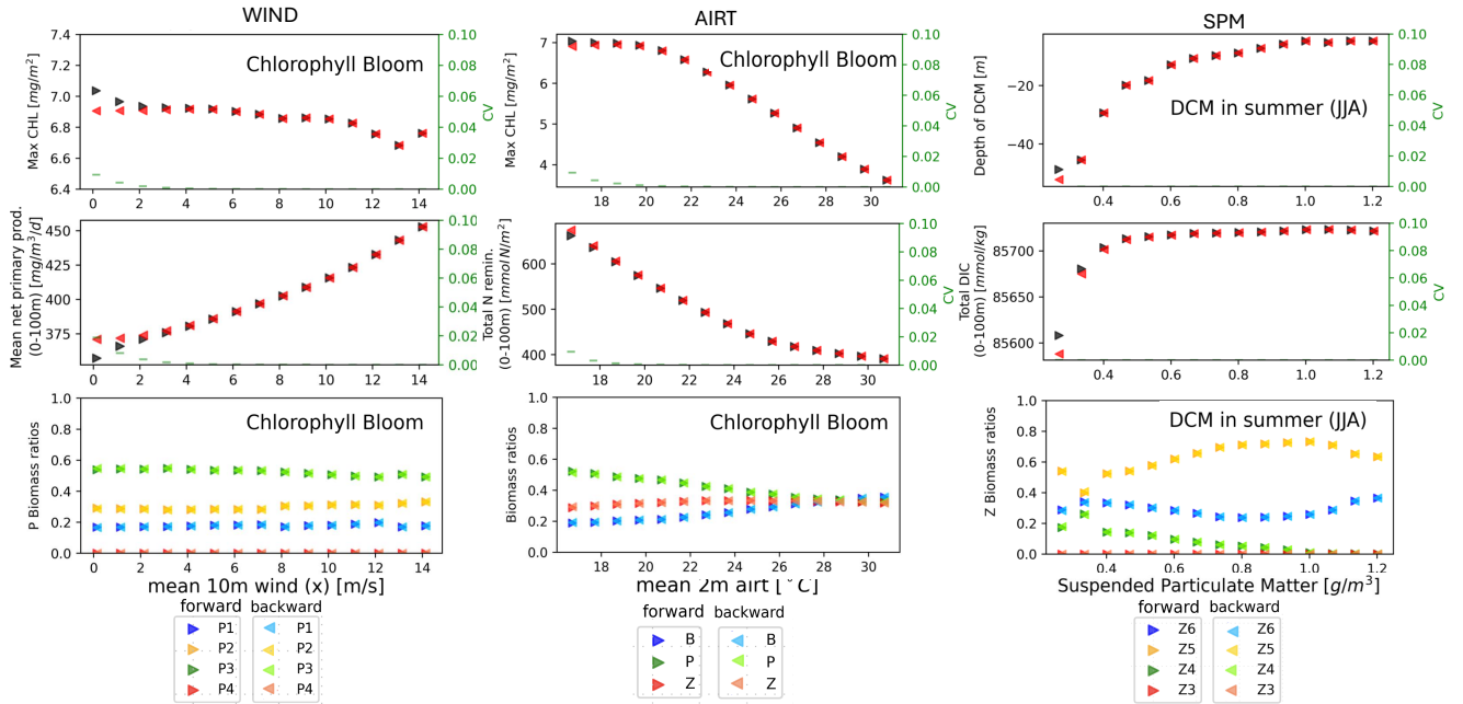
Figure 4. EXP-SEQ setup: Bifurcation diagrams showing the reversible response of the model's dynamic regimes associated to seasonal properties (top row), annual production and cycling (mid row) and community composition (bottom row) to wind (left column), air temperature (mid column) and SPM (right column). The mean magnitude of the environmental forcings (x-axis) goes from its original value (left) to extreme values (right). The panels show a reversible response: the forward path (black), from original to extreme environmental condition, and the backward path (red), from extreme to original environmental condition, follow the same trajectory. For community composition (bottom row) the forward path, from original values to extreme values, is showed in darker colours and the backward path, from extreme values to original values, is showed in lighter colours. Different colours indicates different plankton groups (mid panel) or plankton functional types (left and right panels). The reversibility has been quantified with CV < 0.1 , shown in green. The methodology is presented in Sect.2.4.1.
