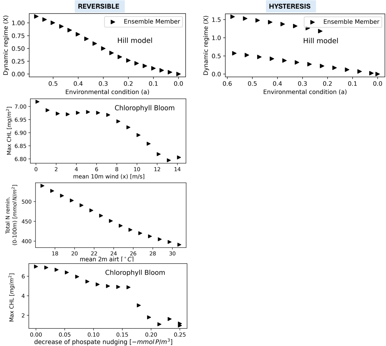
Figure 6. EXP-INI setup: Bifurcation diagrams showing the response of the model's dynamic regimes to environmental forcings. The mean magnitude of the environmental forcings (x-axis) goes from its original value (left) to extreme values (right). The left panels show a reversible response: for each value of the environmental forcings all the ensemble members with different initial conditions visit the same dynamic regime (only one triangle). The right panels show the hysteresis, for some values of the environmental forcings different ensemble members visit different dynamic regimes (two triangles in column). The first row is a simplified representation of the response to environmental forcing using the Hill model (Scheffer et al., 2001), where a is a parameter of the model. The methodology is presented in Sect.2.4.2. The other rows show the response of the dynamic regimes to the variation of 3 environmental forcings (wind, air temperature and phosphate nudging). Hysteresis never occurs for the studied forcings. CV is not shown because always smaller than 0.1.
