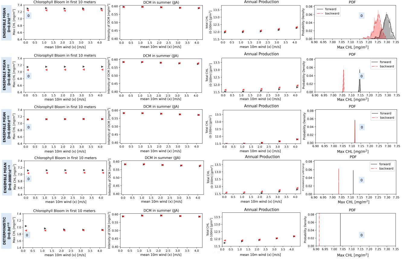
Figure 7. Bifurcation diagrams showing the response of the model's dynamic regimes to the increase of wind forcing in the EXP-DEM experimental setup. Each row shows the dynamic regimes for a different noise intensity decreasing from the top row ( D = 0.01 d^{-1/2} ) to the bottom row (deterministic solution). Along a row the first three panels show the ensemble mean of a dynamic regime for the forward (black) and backward (red) simulations. The last panel, along a row, shows the probability density function of a dynamic regime (Chlorophyll bloom Max CHL) computed over the ensemble of simulations for the first value of wind forcing (unperturbed), indicated by the "0" in the first and last panels. The methodology is presented in Sect.2.4.3.
