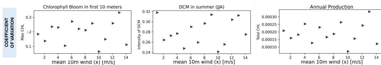
Figure 8. Bifurcation diagrams showing the response of the model’s dynamic regimes to the perturbation of the model parameters under the increase in wind forcing (EXP-BGC, presented in Sect.2.4.4). The y-axis shows the coefficient of variation (CV) of the dynamic regimes over the ensemble of simulations with different parameters. The CV of the annual production dynamics regimes (rightmost panel) is 3 orders of magnitude lower than that of the seasonal dynamic regimes (first two panels).
