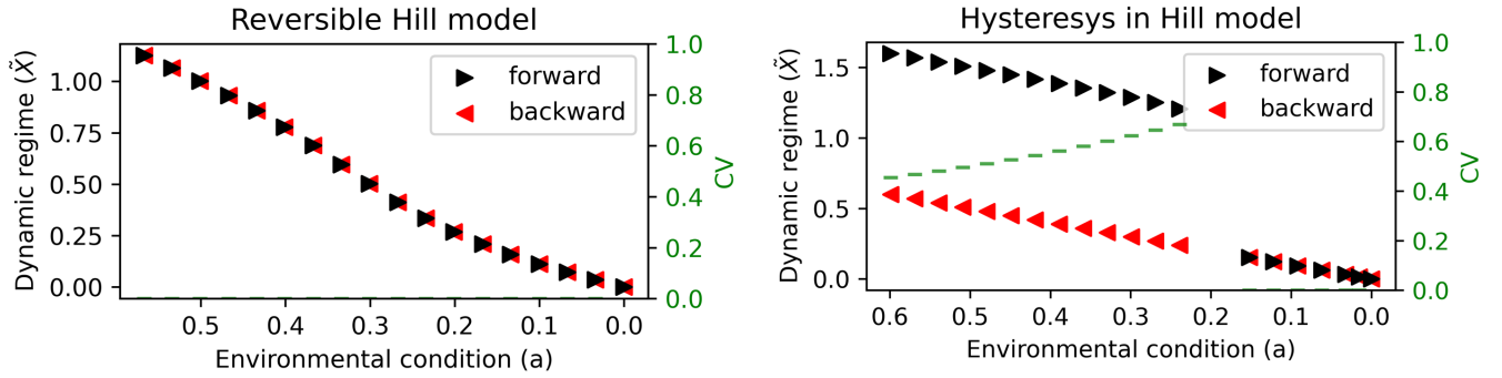
Figure 2. Bifurcation diagrams showing the response of the Hill model’s dynamic regimes to the environmental condition a . The left panel show a reversible response of the Hill model with parameters p = 2 and b = r = h = 1 , the forward path (black), from original to extreme environmental condition, and the backward path (red), from extreme to original environmental condition, follow the same trajectory satisfying CV < 0.1 . The right panel show the hysteresis in the Hill model with parameters p = 18 (chosen to obtain a figure similar to the BFM outputs shown in the following) and b = r = h = 1 , the forward path (black), from original to extreme environmental condition, and the backward path (red), from extreme to original environmental condition, follow different trajectories satisfying CV > 0.1 .
