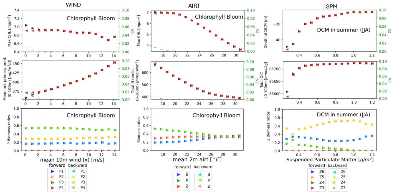
Figure 4. EXP-SEQ setup: Bifurcation diagrams showing the reversible response of the model's dynamic regimes associated to seasonal properties (top row), annual production and cycling (mid row) and community composition (bottom row) to wind (left column), air temperature (mid column) and SPM (right column). The mean magnitude of the environmental forcings (x-axis) goes from its original value (left) to extreme values (right). The panels show a reversible response: the forward path (black), from original to extreme environmental condition, and the backward path (red), from extreme to original environmental condition, follow the same trajectory. For community composition (bottom row) the forward path, from original values to extreme values, is showed in darker colours and the backward path, from extreme values to original values, is showed in lighter colours. Different colours indicates different plankton groups (mid panel) or plankton functional types (left and right panels). The reversibility has been quantified with CV < 0.1 , shown in green. The methodology is presented in Sect.2.4.1.
