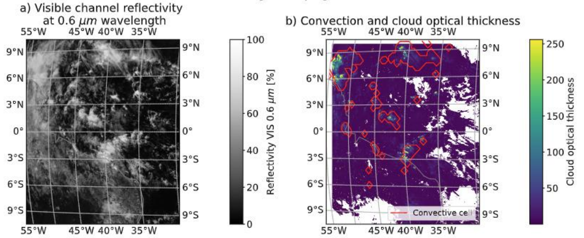
Figure 13. Satellite scene for the HAIC-HIWC II campaign case study. We considered flight 23, flying from French Guyana the 26 th May 2015. Panel a) shows the SEVIRI visible channel at 0.6 \mu\text{m} wavelength reflectivity. Panel b) depicts the cloud optical depth from Optimal Cloud Analysis (EUMETSAT, 2022) and deep convective cells from the TOOCAN database (Fiolleau and Roca, 2019).
