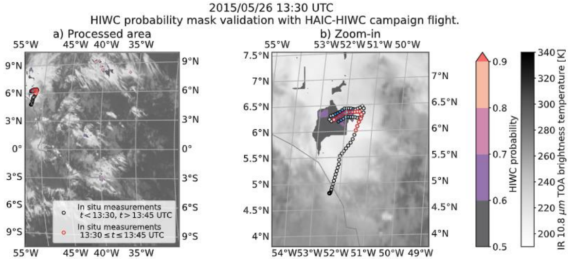
Figure 14. HIWC mask validation with flight 23 of the HAIC-HIWC II flight campaign. The flight crossed a HIWC region ( \text{IWC} \geq 0.5 \text{ g} \cdot \text{m}^{-3} ) from 13:37 to 13:45 peaking at 13:41 with \text{IWC} = 3.3 \text{ g} \cdot \text{m}^{-3} . HIWC measurements are depicted in blue shades, while no-HIWC are shown in grey shades. Markers with red borders depict the flight position within the satellite scanning times. Flight waypoints are corrected for parallax effect, shifted to the corresponding satellite grid coordinates.
