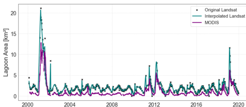
Figure B5. Time series of the shallow, salty lagoon area from Landsat, Interpolated Landsat and MODIS images.
