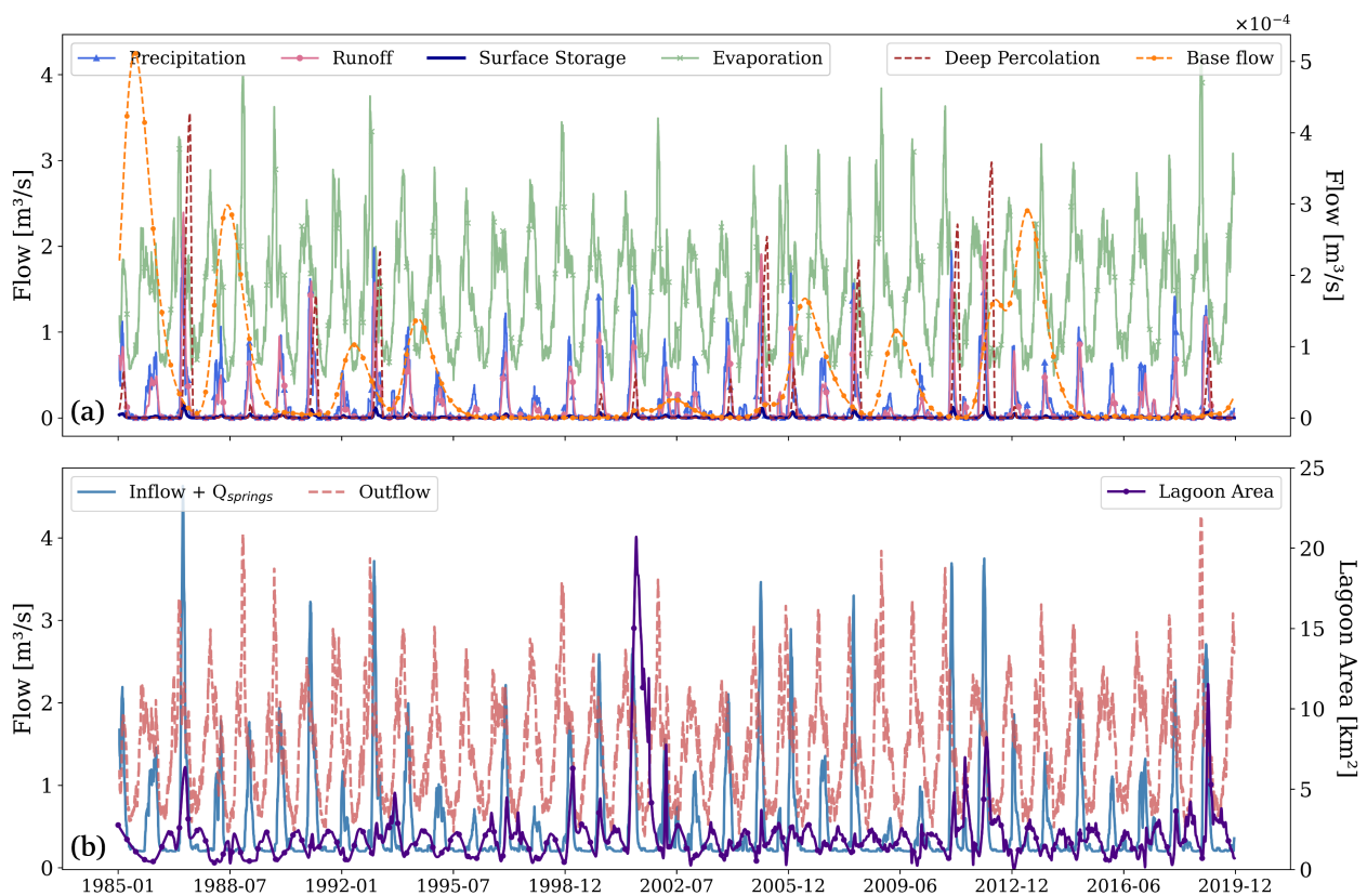
Figure 6. (a) Water balance components for the salt flat nucleus sub-basin, showing daily timeseries in \text{m}^3\text{s}^{-1} of (left axis) precipitation, runoff, surface storage, total evaporation, and (right axis) deep percolation and base flow, all derived from the rainfall-runoff model. (b) Total inflow (sum of precipitation, runoff and base flow) and total outflow (sum of total evaporation and deep percolation) in \text{m}^3\text{s}^{-1} . Springs discharge ( Q_{\text{springs}} ) is added to the inflow and assumed constant at 0.2 \text{ m}^3\text{s}^{-1} according to DGA hydrogeological reports. Lagoon area from Landsat imagery is displayed in the right y-axis [ \text{km}^2 ]. A 30-days running average is applied to the timeseries.
