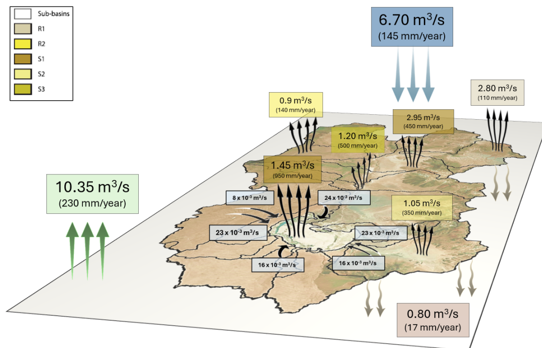
Figure 7. Schematic representation of long-term mean annual flows from the Salar del Huasco, Chile, in \text{m}^3 \text{ s}^{-1} and in parenthesis \text{mm year}^{-1} . Total evaporation is presented in green, total precipitation in blue and total groundwater recharge in brown. Springs are displayed in light blue. The rest represent evaporative losses from each Hydrological Response Unit (see Fig. 2b). Evaporation from the salt flat nucleus basin is separated from the rest S1-type, as it is the main discharge point per unit area of the basin ( 950 \text{ mm year}^{-1} ).
