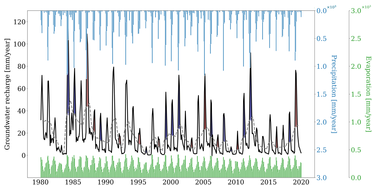
Figure 3. Groundwater recharge estimated for the Salar del Huasco basin using Uribe et al. (2015) modified rainfall-runoff model. Values are presented for the 1980 - 2019 period as monthly averages in \text{mm year}^{-1} . Groundwater recharge 12-month running average is displayed in grey dashed line. Blue shades correspond to La Niña years, while red shades correspond to El Niño years. Monthly averaged precipitation (blue bars) and evaporation (green bars) in \text{mm year}^{-1} from gridded CR2MET and EEFLUX datasets, respectively, are also presented.
