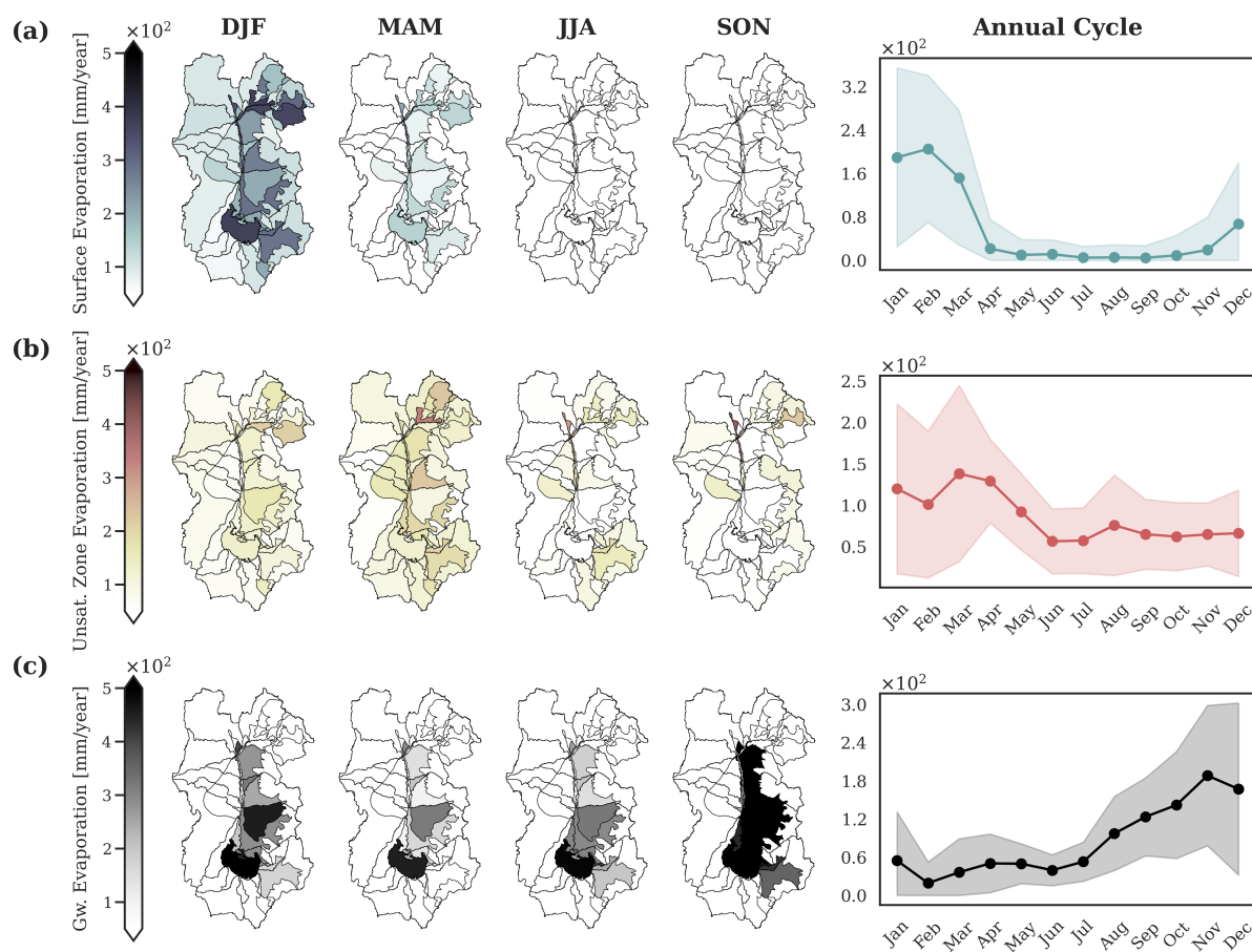
Figure 5. Left panels: Spatial distribution of seasonal means across sub-basins in \text{mm year}^{-1} for (from left to right) DJF, MAM, JJA and SON for (a) Surface evaporation, (b) Unsaturated zone evaporation and (c) Groundwater evaporation. Right panels: Monthly mean variability of each variable [ \text{mm year}^{-1} ]. Shades indicate the standard deviation.
