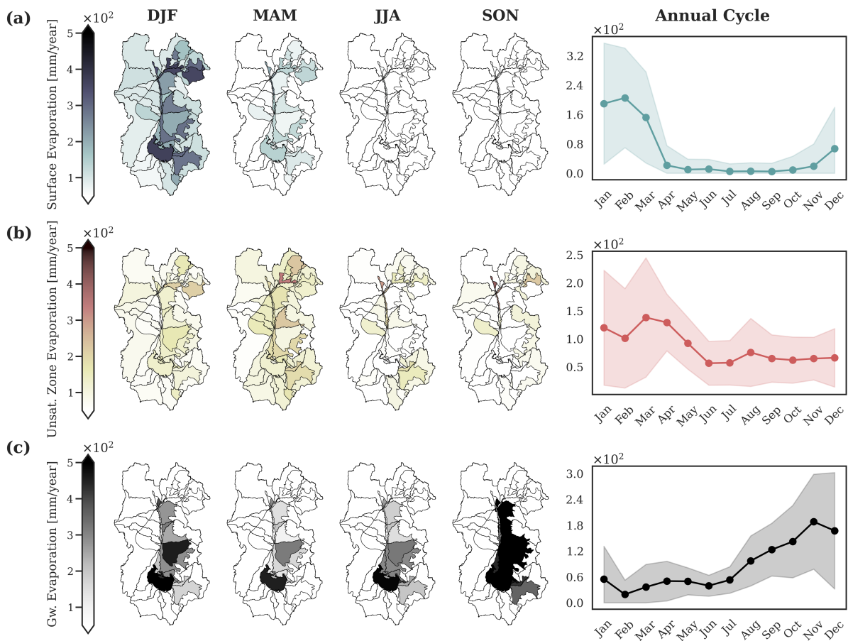
Figure 5. Left panels: Spatial distribution of seasonal means across sub-basins in \text{mm year}^{-1} for (from left to right) DJF, MAM, JJA and SON for (a) Surface evaporation, (b) Unsaturated zone evaporation and (c) Groundwater evaporation. Right panels: Monthly mean variability of each variable. Values represent monthly means, scaled to annual equivalents ( \text{mm year}^{-1} ) for consistency across all water balance components. Shades indicate the standard deviation.
