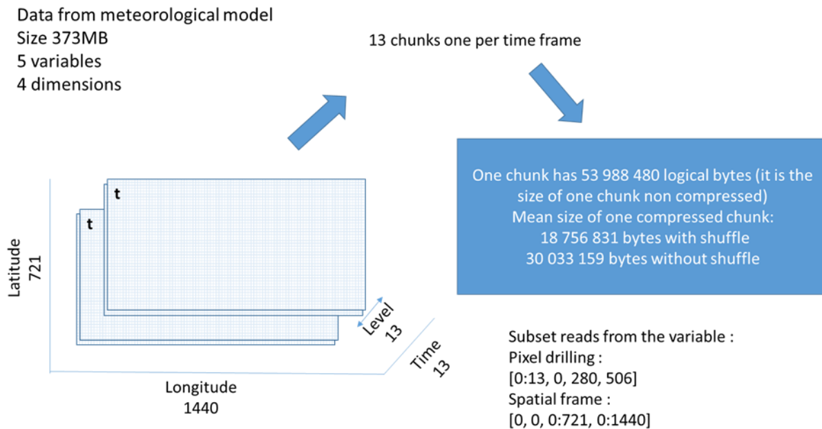
385 Figure 87: GFS meteorological model temperature dataset and variable read in the experiments
