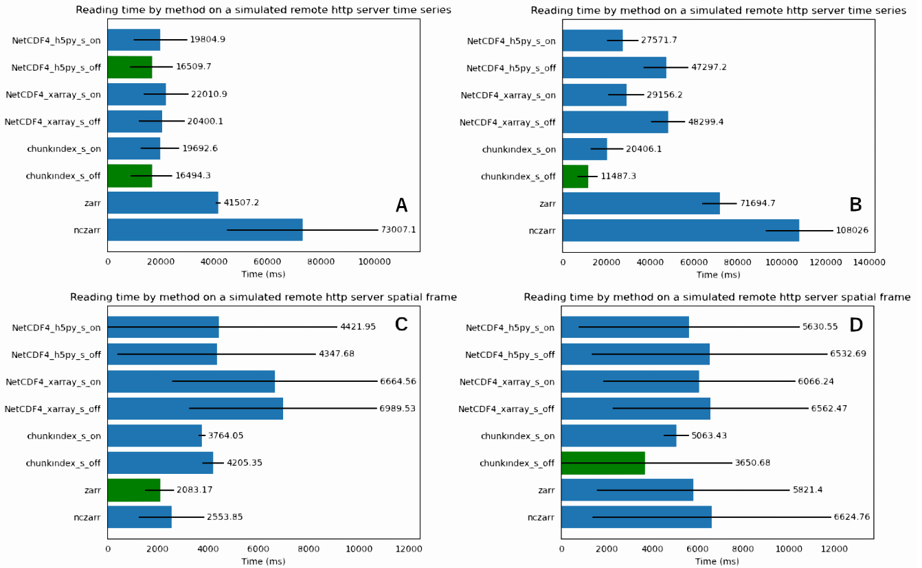
Figure 109: Results of simulated remote file system with poor network connection: (A) the Remote_CMEMS_time_series experiment mean time for reading a time series in the CMEMS oceanic model (B) the Remote_GFS_time_series experiment mean time for reading a time series in the GFS temperature dataset (C) the Remote_CMEMS_spatial_frame experiment mean time for reading a spatial frame in the CMEMS oceanic model output (D) the Remote_GFS_spatial_frame experiment mean time for reading a spatial frame in the GFS temperature dataset
