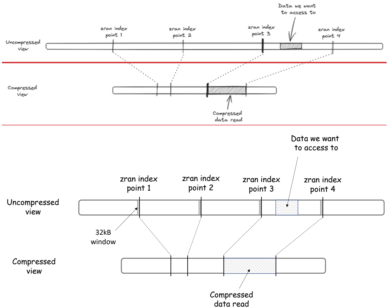
Figure 32: Principle of the zran index points on one chunk.
