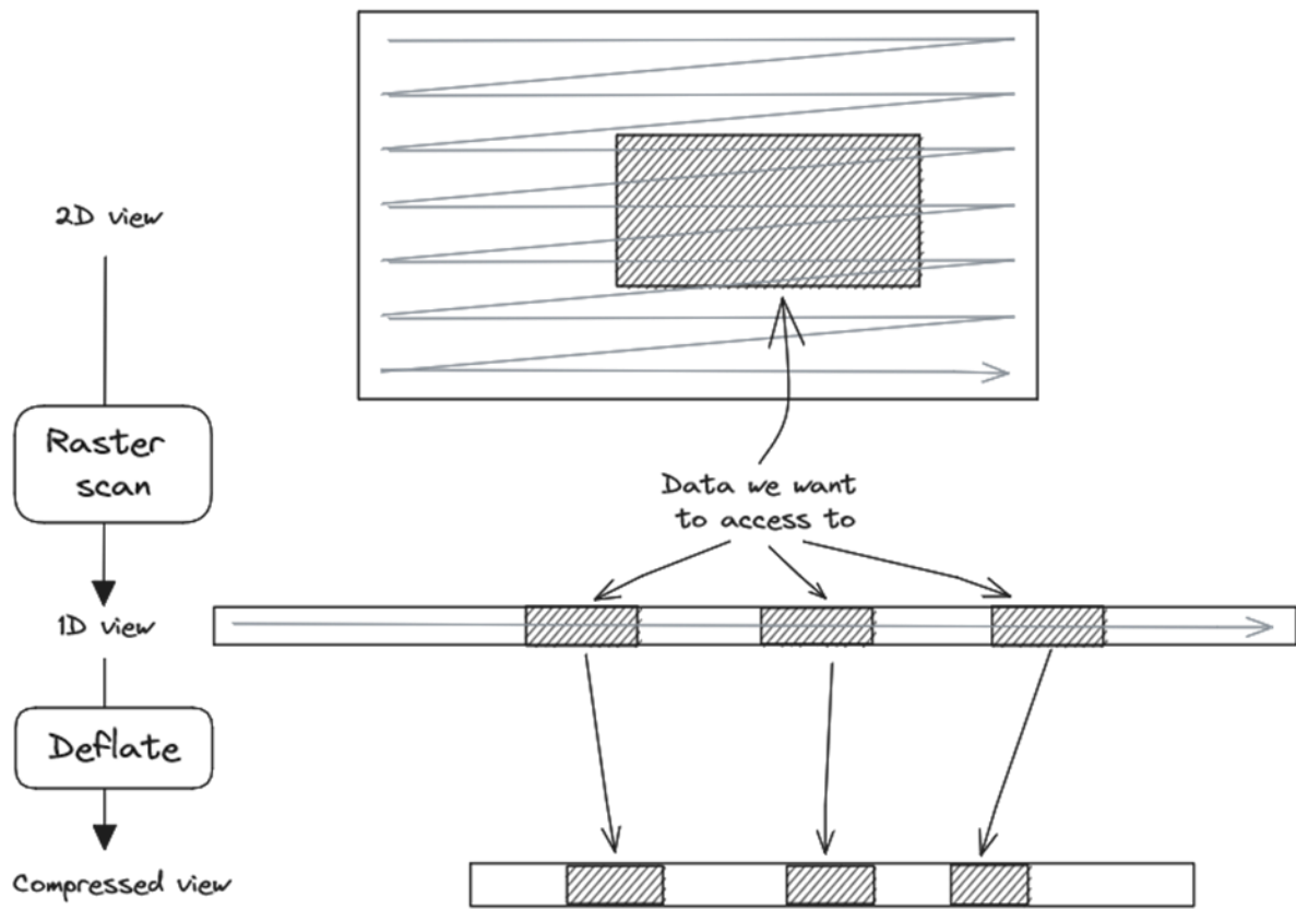
Figure 65: Raster scan scatters the connected data in the compressed chunk
