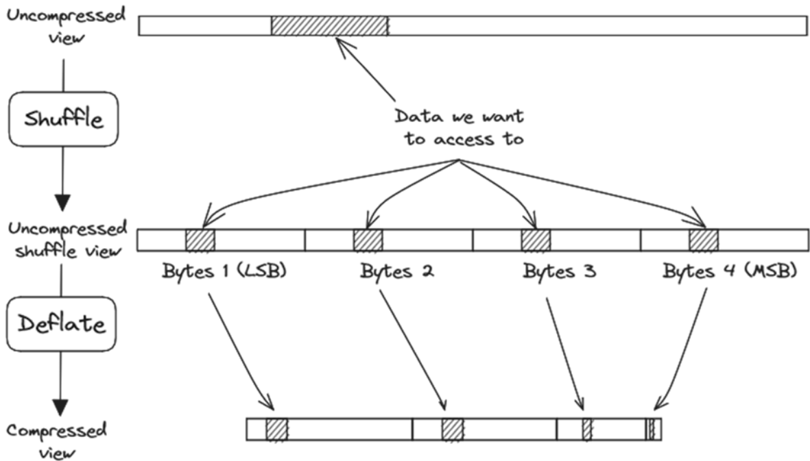
Figure 54: Shuffling scatters the data in the compressed chunk. In this example, bytes 1 are the Least Significant Bytes (LSB) and bytes 4 are the Most Significant Bytes (MSB).
