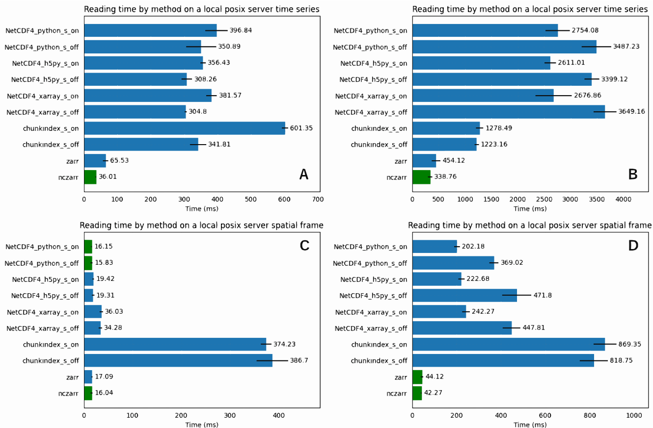
Figure 98: Results of the local file system experiment: (A) the Local_CMEMS_time_series mean time for reading a time series in the CMEMS oceanic model output (B) the Local_GFS_time_series mean time for reading a time series in the GFS temperature dataset (C) the Local_CMEMS_spatial_frame mean time for reading a spatial frame in the CMEMS oceanic model output (D) the Local_GFS_spatial_frame mean time for reading a spatial frame in the GFS temperature dataset.
