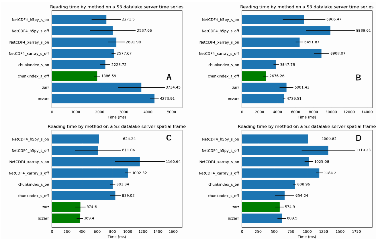
Figure 1140: Results of the S3 storage service experiment: (A) S3_CMEMS_time_series mean time for reading a time series in the CMEMS oceanic model output (B) S3_GFS_time_serie mean time for reading a time series in the GFS temperature dataset (C) S3_CMEMS_spatial_frame mean time for reading a spatial frame in the CMEMS oceanic model output (D) S3_GFS_spatial_frame mean time for reading a spatial frame in the GFS temperature dataset.
