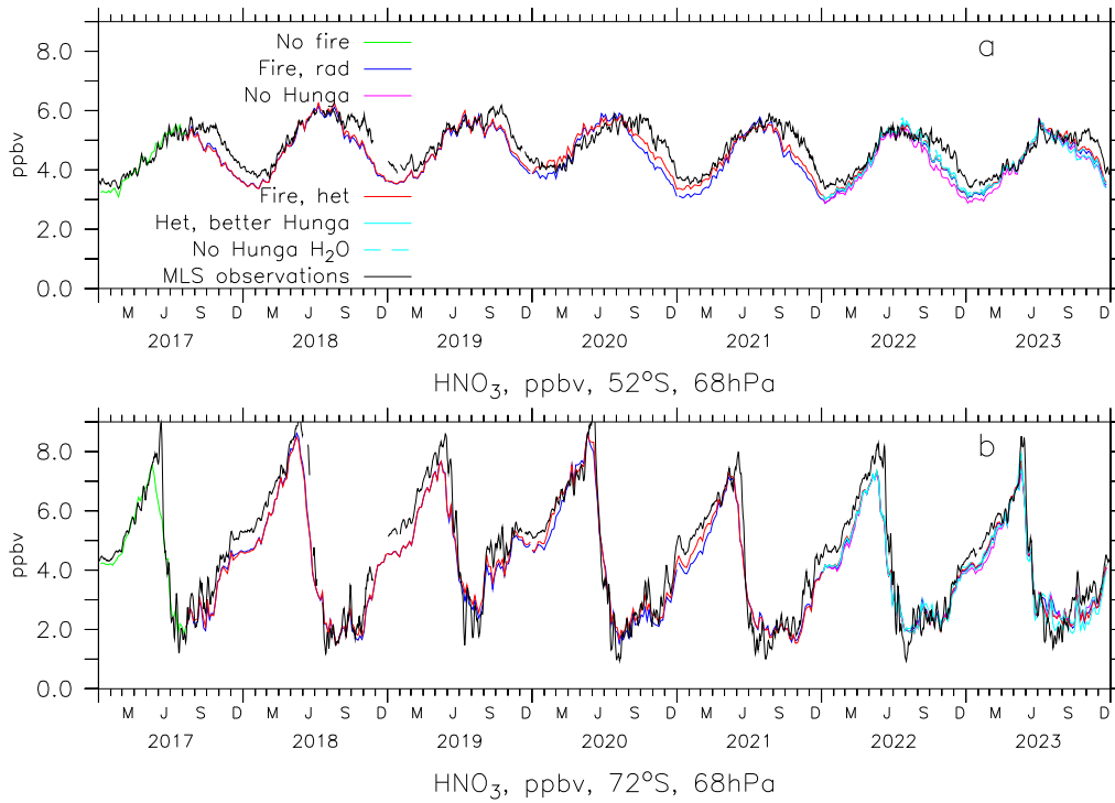
Figure 6. Simulated and observed \text{HNO}_3 at 68 hPa at 52°S (a) and 72°S (b). EMAC scenarios of Table 2 see legend.
