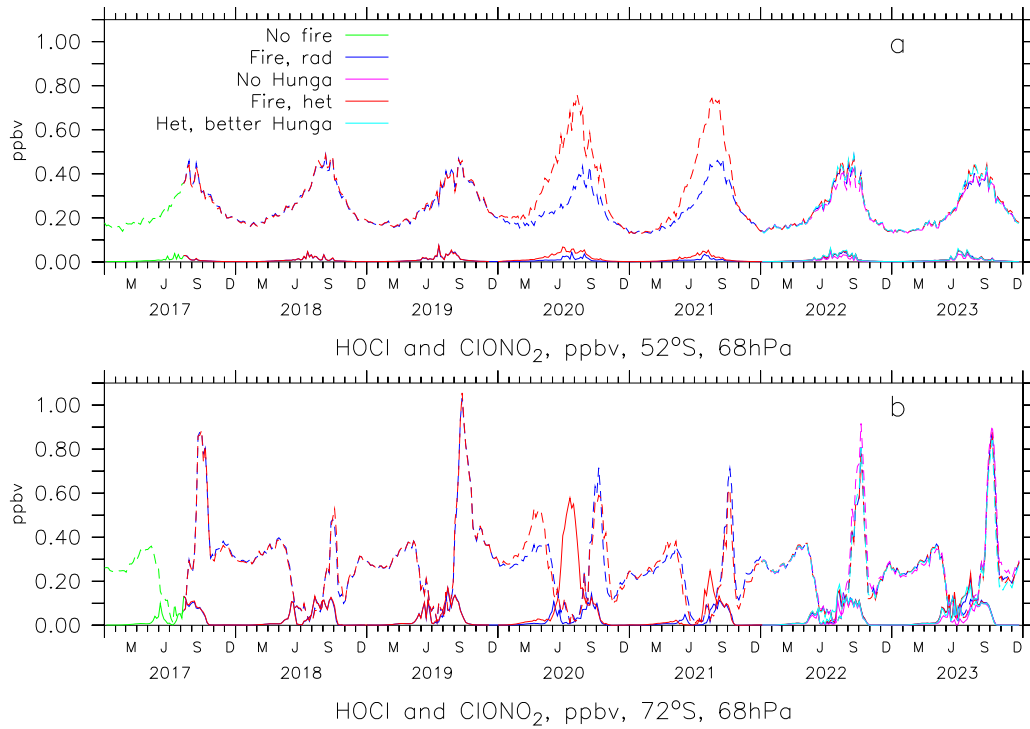
Figure 5. Simulated HOCl at 68 hPa at 52°S (a) and 72°S (b). Full curves, shown EMAC scenarios of Table 2 in legend. Dashed curves show calculated ClONO 2 .
