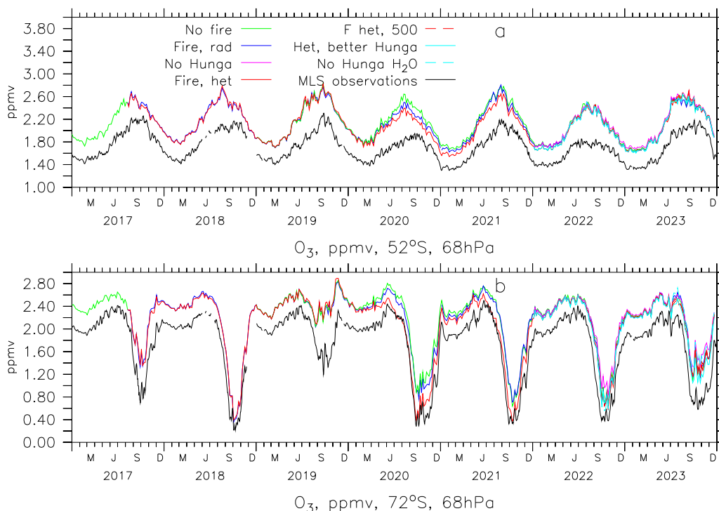
Figure 7. Simulated and observed O 3 at 68 hPa at 52°S (a) and 72°S (b). EMAC scenarios of Table 2 see legend.
