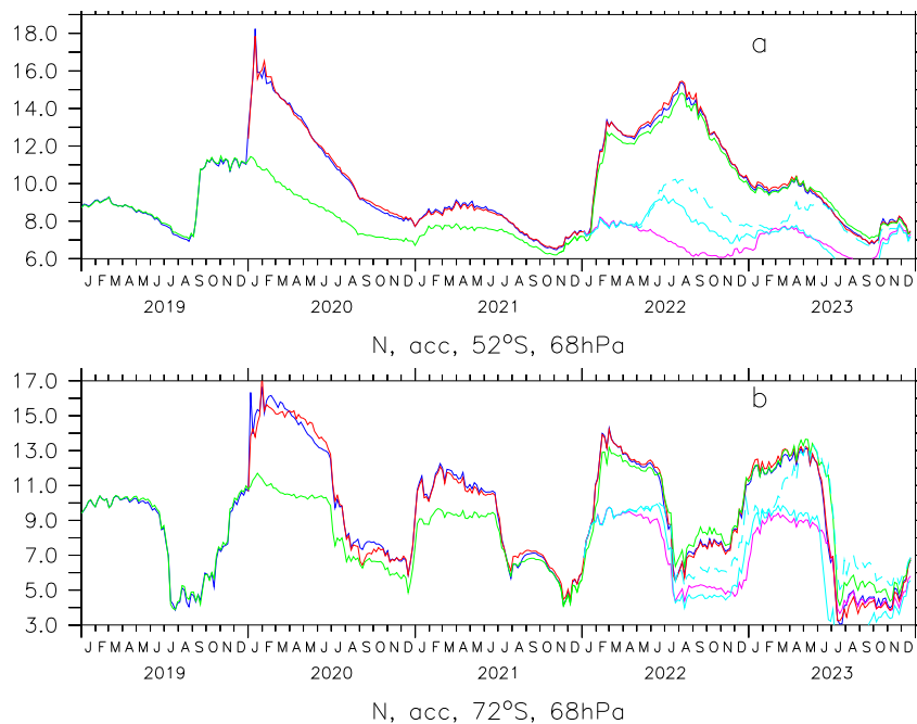
Figure A4. Calculated particle number density (accumulation mode, 1/\text{cm}^3 ), colors as in Table 2.
