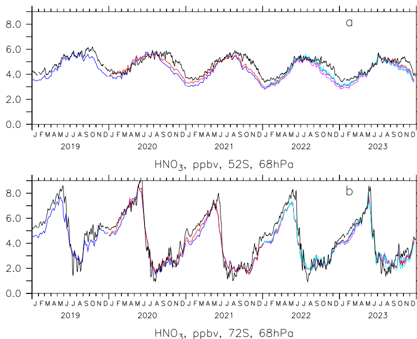
Figure 6. As Fig. 4 but for HNO 3 . Scenario 6 and 7 of Table 2 shown
