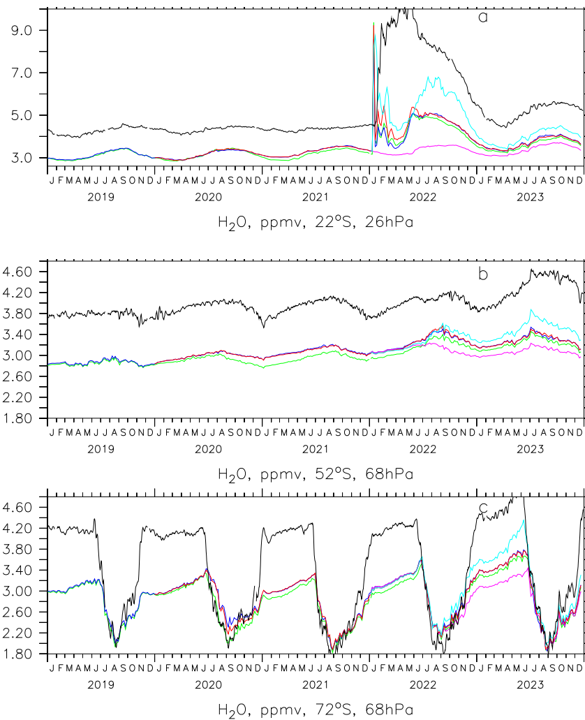
Figure A1. Calculated and observed water vapor, colors as in Fig. 7. Panel a is for the subtropical middle stratosphere. Lightblue is the sensitivity study with almost co-injected SO_2 and H_2O .
