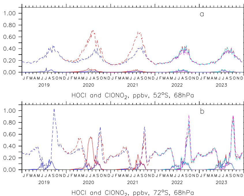
Figure 5. Simulated HOCl at 68 hPa at 52°S (a) and 72°S (b). Blue: EMAC with Hunga including water and dynamical effects of fires, Purple: EMAC without Hunga, Red: EMAC with Hunga and enhanced heterogeneous chlorine activation on organic particles. Lightblue: as red but with better Hunga SO 2 and water vapor injections. Curves for EMAC scenario 1 and 5 not shown since close to 2 and 4. Dashed curves show calculated ClONO 2 .
