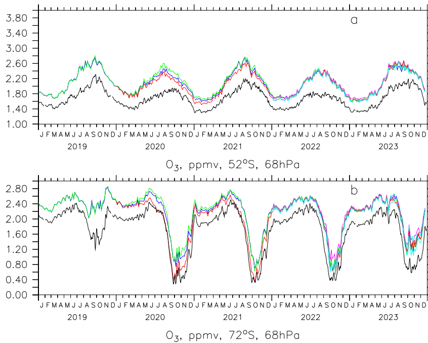
Figure 7. As Fig.4 but for ozone, green without fires.
