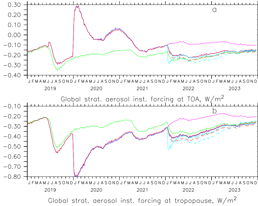
Figure 2. Calculated instantaneous radiative forcing by aerosol at the Top of the Atmosphere (TOA, a) and tropopause altitude (b). Green: EMAC without fires, blue: EMAC with fires, purple: no Hunga, red: EMAC with heterogeneous chemistry on smoke particles, red dashed: as red but 500kt SO 2 , lightblue: same but SO 2 almost co-injected with H 2 O (see Table 2, scenario 6), lightblue dashed: same without H 2 O injection.
