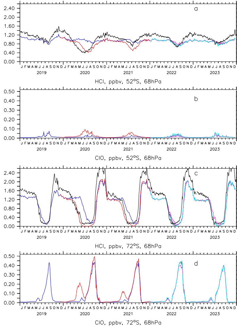
Figure 4. Simulated and observed HCl at 68 hPa at 52°S (a) and 72°S (c). Blue: EMAC with Hunga including water and dynamical effects of fires, Purple: EMAC without Hunga, Red: EMAC with Hunga and enhanced heterogeneous chlorine activation on organic particles, Lightblue: as red but more realistic Hunga SO 2 and H 2 O injections, Lightblue dashed: same without H 2 O injection (see Table 2). Black: MLS observations. Scenario 1 and 5 not shown since close to scenario 2 and 4. Calculated ClO in panels b and d (MLS not shown). 5-day averages for EMAC, daily averages with 5-day boxcar smoothing for MLS.
