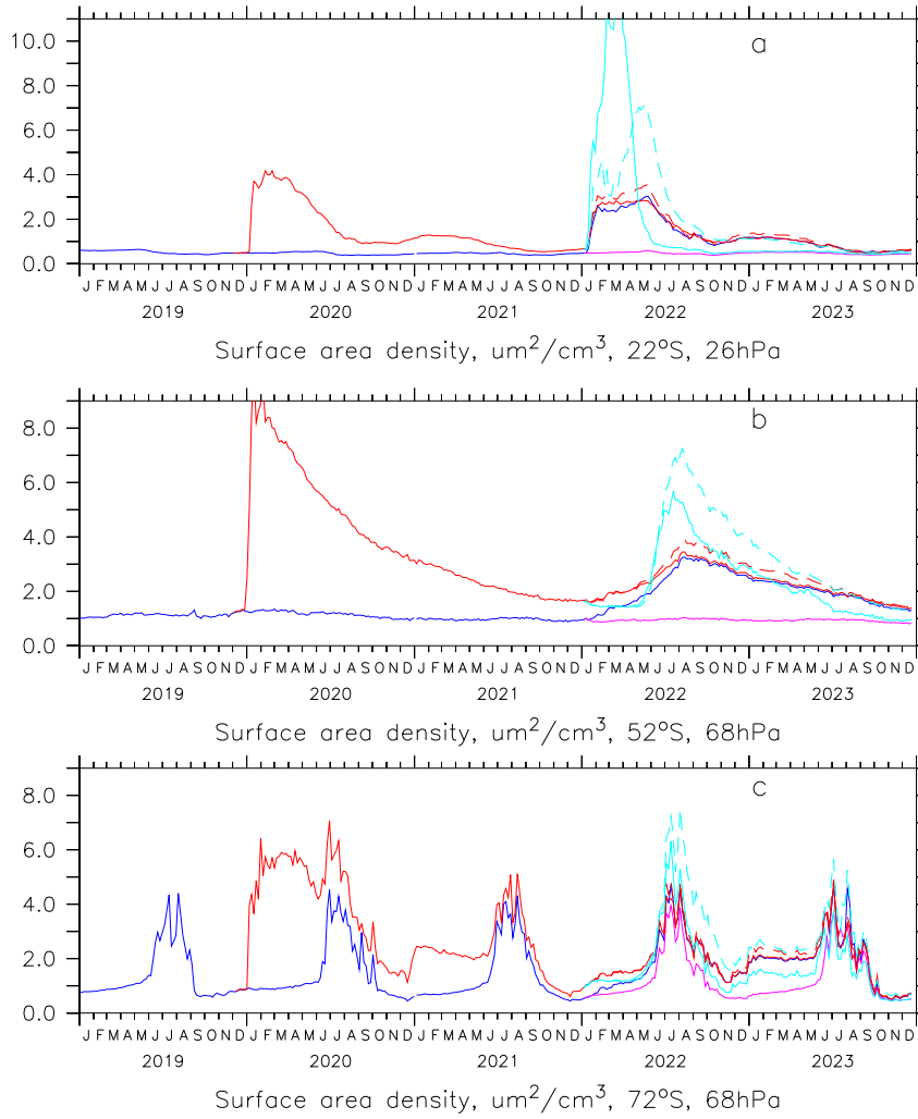
Figure 3. Calculated surface area density [ \mu\text{m}^2/\text{cm}^3 ] for heterogeneous chemistry in the middle stratosphere in southern subtropics (a) and the lower stratosphere in southern middle (b) and high (c) latitudes. Blue: sulfate and PSCs only with radiative effect of smoke (scen 2 of Table 2); Purple: without Hunga; Red: Including smoke particles; Lightblue: better \text{SO}_2 and \text{H}_2\text{O} (scen 6); Lightblue dashed: same without \text{H}_2\text{O} injection.
