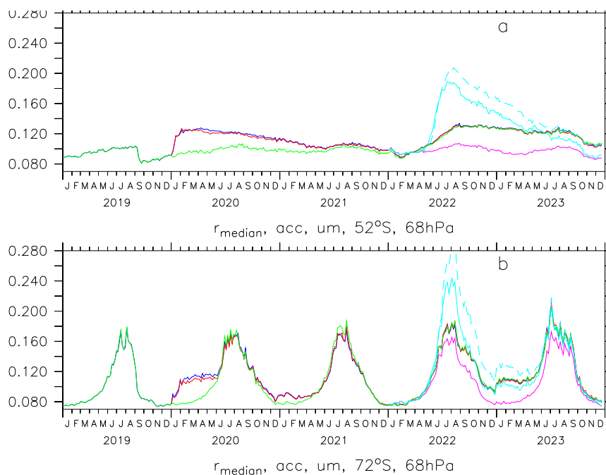
Figure A5. Calculated median particle radius (accumulation mode, \mu\text{m} ), colors as in Table 2.
