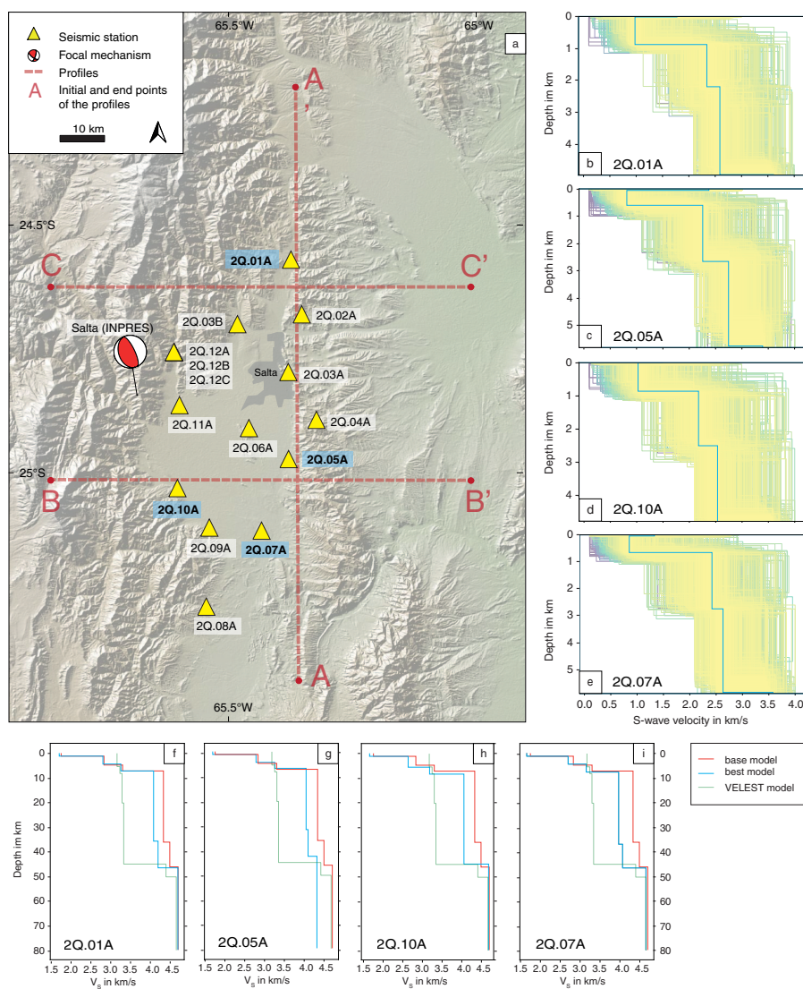
Figure 8. Base model (Zeckra (2020))(in red), VELEST model (in green) and best model inversion (in blue) for four representative stations; 01A, 05A, 07A and 10A namely.
