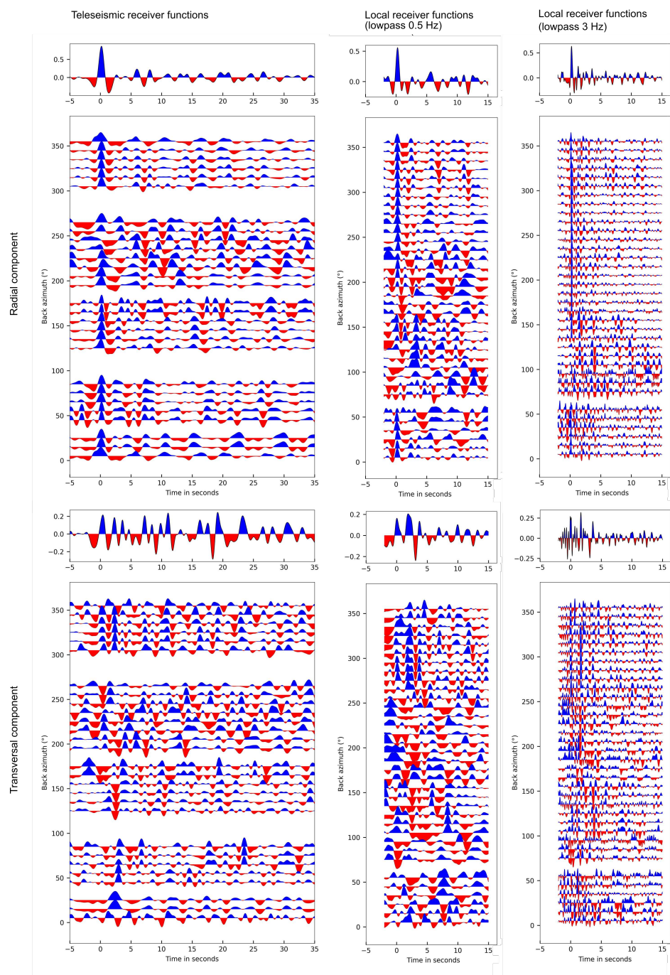
Figure 4. Teleseismic and local receiver functions computed for station 01A. The individual receiver functions are binned in 10^\circ intervals, with an overlap of 5^\circ . The linear stack is represented on top of each panel. The first row shows the radial component, while the bottom row shows the transverse component.
