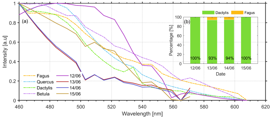
Figure 10. (a) Pollen fluorescence spectra of Fagus , Quercus , Dactylis and Betula obtained in vivo by lidar excitation at 355 nm (dashed lines) and pollen spectra (continuous lines) obtained by the lidar multichannel spectrometer, along with (b) the percentages of each pollen type for various clustering algorithms and metrics (from 12-15 June) from ground up to 1.2 km a.s.l.
