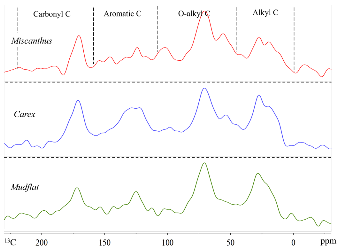
Fig. S1 spectra of soil organic carbon acquired using ^{13}\text{C} nuclear magnetic resonance of different community.
