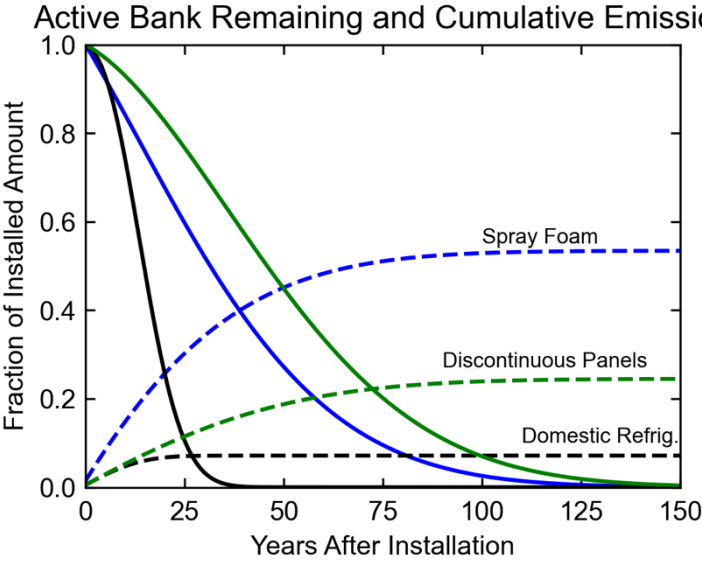
Figure 4. Weibull decommissioning functions assumed for three product types: (1) spray foam, (2) discontinuous panels, and (3) domestic refrigeration foam. These three markets were chosen because their rates of emission from foam and service lifetimes provide a wide range of responses. Solid lines represent the amount of HCFC-141b remaining in the equipment as a fraction of what was installed in year 0. Dashed lines represent the cumulative amount emitted while the product is in use. The domestic refrigeration curve peaks slightly higher here than in Fig. 1 because in this figure, the fractional emission is relative to the amount of HCFC-141b installed, not produced.
