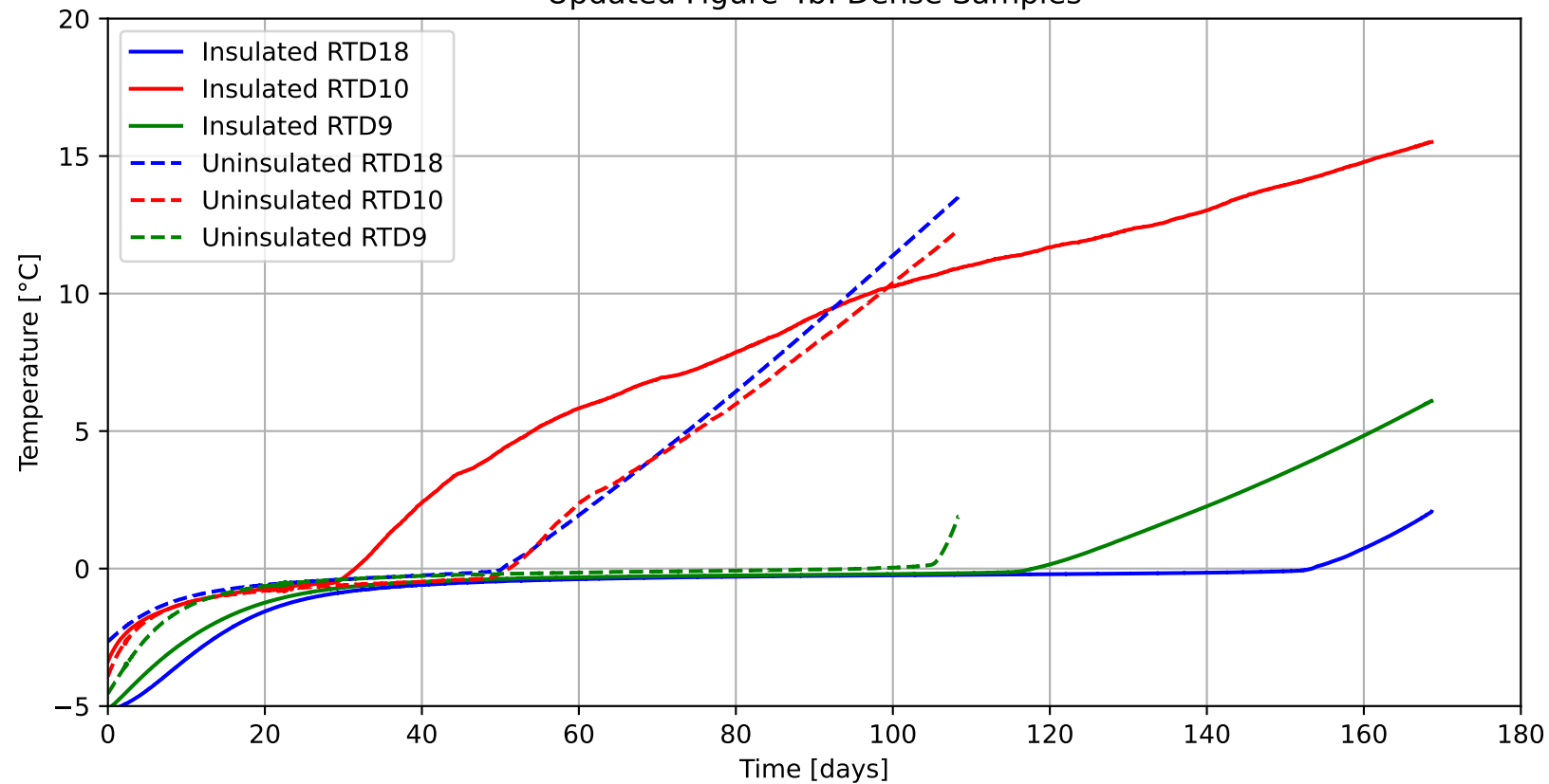
Updated Figure 4b: Dense Samples
