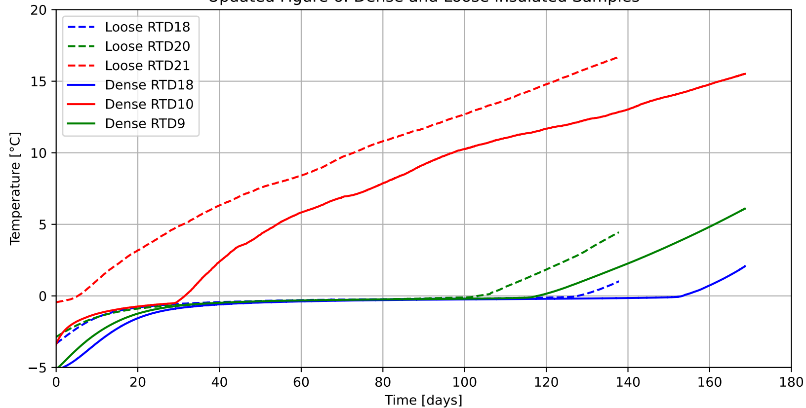
Updated Figure 6: Dense and Loose Insulated Samples
