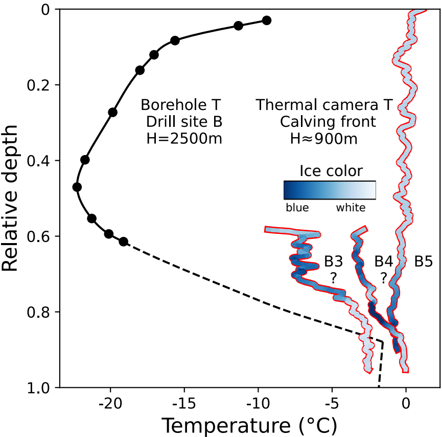
Figure 7. Temperature (T) and blue color index profiles scaled and located into the ice column. The icebergs B3, B4 and B5 from Fig. Figure 3 are scaled and situated in the ice column to be compared with the temperature profile at drill site B (black line) and its extrapolation (dashed line, Funk et al. (1994))(dashed line; Funk et al., 1994). Temperature is plotted on the horizontal axis as a function of relative depth. Ice color is represented by the color of the points (dark blue indicates blue ice). Vertical positions of B3 and B4 are uncertain.
