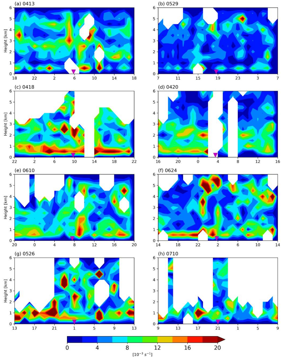
Figure S1: The time-height profiles of vertical wind shear for each individual case (unit: 10^{-3} \text{ s}^{-1} )
