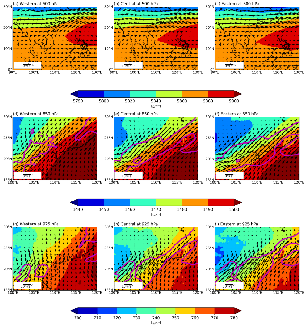
Figure 5 Composite mean geopotential heights and wind field at 500 hPa (a–c), 850 hPa (d–f) and 925 hPa (g–i) over WSHR events in Western (a, d, g), Central (b, e, h) and Eastern (c, f, i) GD. Geopotential heights in gpm, wind vectors (black arrows) in \text{m s}^{-1} with wind speed greater than 8 \text{ m s}^{-1} marked in magenta contours.
