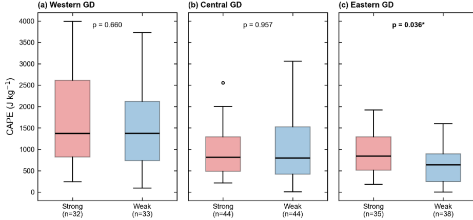
Figure 14 Pre-onset CAPE (ERA5, averaged over t = -6 to -2 h) for strong-rainfall (red) and weak-rainfall (blue) events in (a) western GD, (b) central GD, and (c) eastern GD. The box plots show the median, interquartile range, and whiskers extending to 1.5 \times \text{IQR} . The p value of the Mann-Whitney U-test is annotated; an asterisk denotes p < 0.05 .
