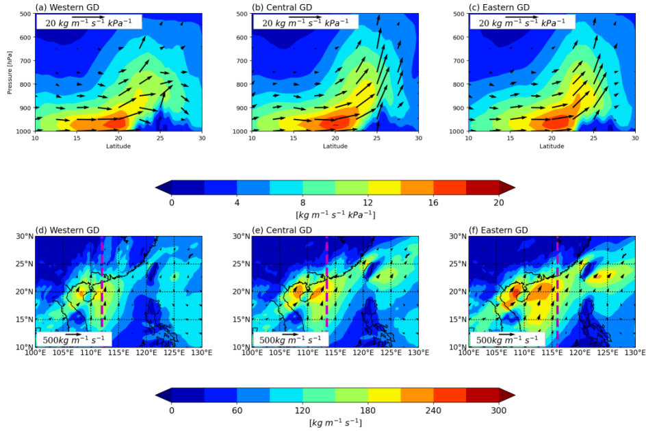
Figure 15 Composite mean moisture transport field of WSHR events in 2016–2020 for the Western (a, d), Central (b, e), and Eastern (c, f) regions. Upper panels (a–c): vertical cross-sections of moisture transport along the purple lines shown in (d–f); shading shows the horizontal component ( \text{kg m}^{-1} \text{s}^{-1} \text{kPa}^{-1} ), and arrows show the combined horizontal and vertical components, with the vertical component (VTw) magnified by a factor of 50 for visibility. Lower panels (d–f): spatial distribution of vertically integrated water vapour transport (IVT; \text{kg m}^{-1} \text{s}^{-1} ), with arrows showing IVT vectors and the purple line marking the transect location of the upper panels. IVT is integrated between 1000 and 850 hPa. Fields are averaged over t = -6 to -2 h before onset.
