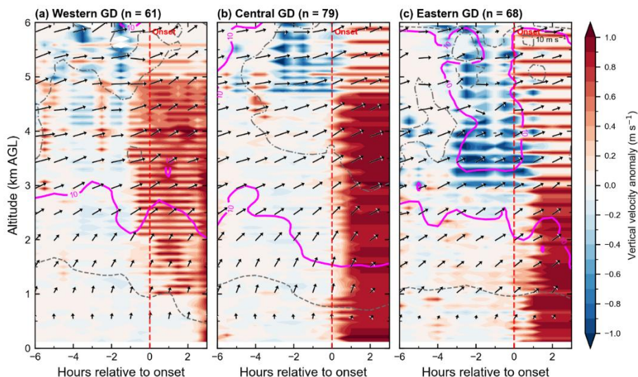
Figure 6 Composite time–height cross-sections of horizontal wind and vertical velocity anomalies for (a) western GD ( n = 61 ), (b) central GD ( n = 79 ), and (c) eastern GD ( n = 68 ) WSHR events. Arrows show composite wind vectors (reference: 10 \text{ m s}^{-1} ); shading shows the median vertical velocity anomaly relative to the t = -6 to -4 h baseline ( \text{m s}^{-1} ; red for ascent, blue for descent); magenta contours mark 10 \text{ m s}^{-1} wind speed. The gray contours with dashed and solid lines indicate 8 and 12 \text{ m s}^{-1} , respectively. The red dashed line indicates onset ( t = 0 ).
