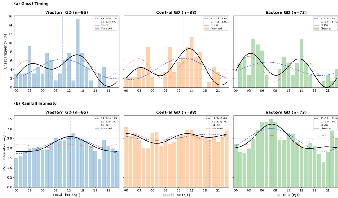
Figure 4 Diurnal variations of (a) WSHR onset frequency and (b) mean rainfall intensity for the western (blue), central (orange), and eastern (green) regions. The dashed and dotted curves show the first (S1, 24 h) and second (S2, 12 h) diurnal harmonics; solid black curves show S1 + S2. Percentages indicate explained variance.
