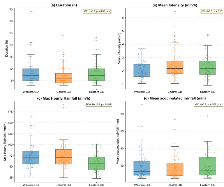
Figure 3 Statistical distributions of WSHR characteristics across three sub-regions: (a) event duration, (b) mean rainfall intensity, (c) maximum hourly rainfall, and (d) mean accumulated rainfall. The boxes show the median and interquartile range (IQR); whiskers extend to 1.5 \times \text{IQR} . The Kruskal–Wallis H statistic and the p -value are annotated in each panel.
