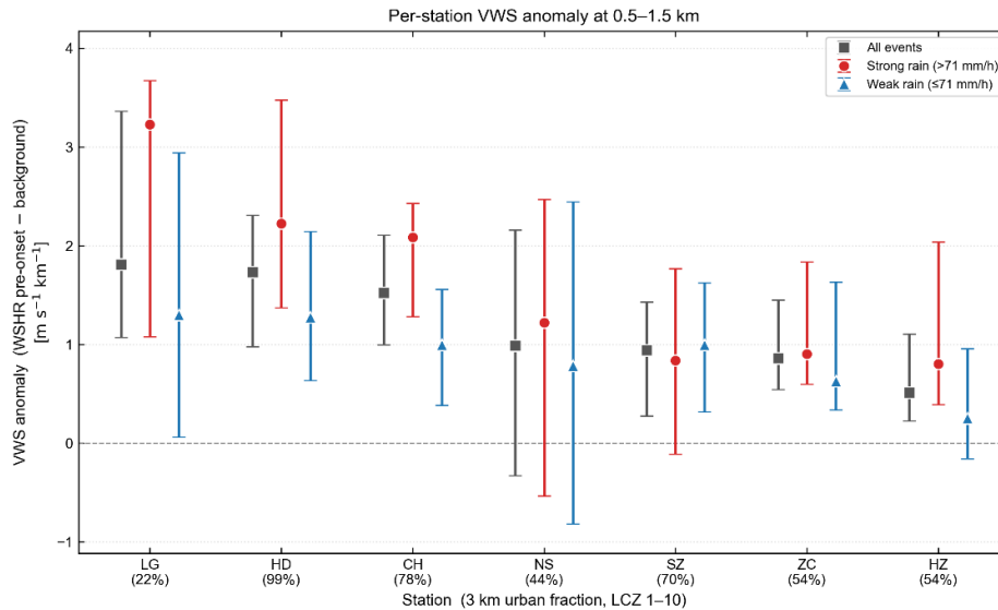
Figure 16 Per-station VWS anomaly composites at 0.5–1.5 km (3-h pre-onset mean) for the seven wind profiler stations in central GD, based on WSHR events during 2016–2020. Stations are ordered by the all-events median (grey squares); error bars denote bootstrap 95 % confidence intervals ( N = 2000 ). Red circles and blue triangles show medians for events with hourly peak rainfall above and below the 71 \text{ mm h}^{-1} split, respectively. x-axis labels include each station's 3-km urban fraction. Station codes: NS (Nansha), LG (Luogang), HD (Huadu), CH (Conghua), ZC (Zengcheng), SZ (Shenzhen), HZ (Huizhou Longmen).
