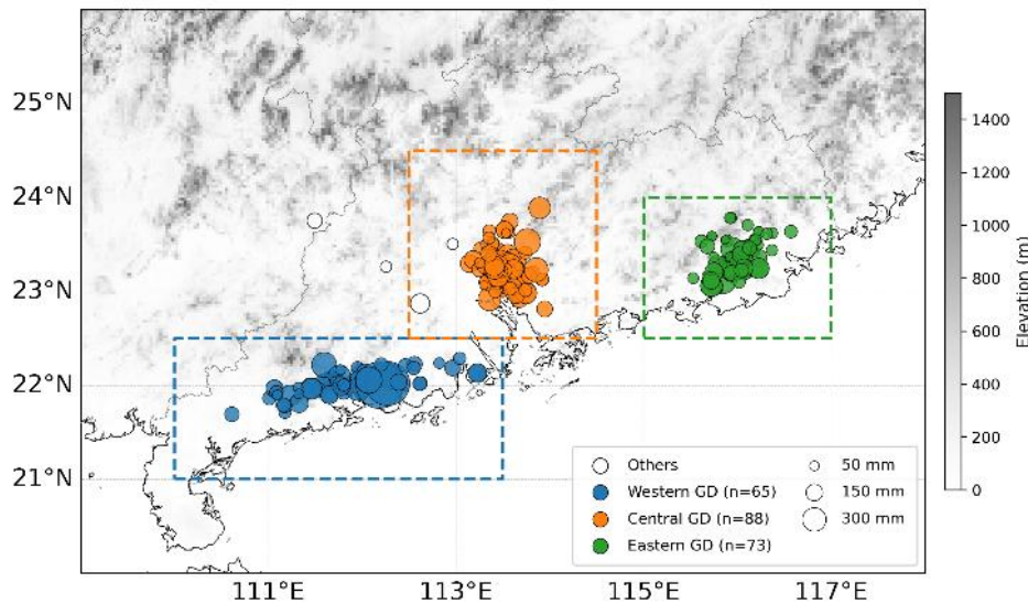
Figure 2 Spatial distribution of the WSHR precipitation centers in Guangdong Province during 2016–2020. The size of the marker is proportional to the maximum accumulated precipitation; white markers indicate invalid events. Dashed rectangles delineate the western (blue, n = 65 ), central (orange, n = 88 ), and eastern (green, n = 73 ) sub-regions. Gray shading shows the elevation of the terrain (m).
