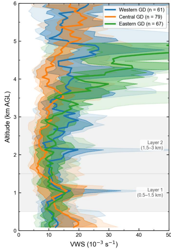
Figure 7 Composite VWS profiles averaged over t = -3 to 0 h for the western GD (blue, n = 61 ), central GD (orange, n = 79 ), and eastern GD (green, n = 67 ) regions. Lines show medians; dark and light shading show the 25-75 percentile range and 10th–90th percentile ranges. The gray bands mark the two layers used in Sect. 4.2: 0.5–1.5 km (Layer 1) and 1.5–3.0 km (Layer 2).
