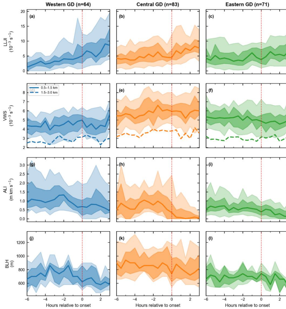
Figure 8 Composite temporal evolution of precursor indices for WSHR events over (a, d, g, j) western GD ( n = 64 ), (b, e, h, k) central GD ( n = 83 ), and (c, f, i, l) eastern GD ( n = 71 ): (a–c) LLJI, (d–f) VWS at 0.5–1.5 km (solid) and 1.5–3.0 km (dashed), (g–i) ALI, and (j–l) BLH. Lines show medians; dark shading shows the bootstrap 95 % CI of the median; light shading shows the interquartile range. The red dashed line marks onset ( t = 0 ).
