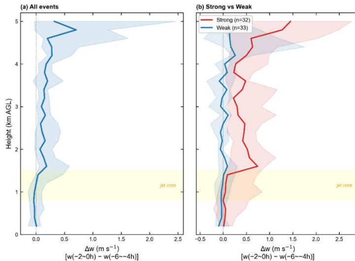
Figure 13 Vertical profiles of the pre-onset vertical velocity change ( \Delta w = \text{mean } w at t = -2 to 0 h minus mean w at t = -6 to -4 h) in western GD. (a) All events: solid line shows the composite median and shading shows the bootstrap 95 % confidence interval. (b) Strong-rainfall (red) and weak-rainfall (blue) events. The yellow band marks the jet core layer (0.8–1.5 km AGL) identified from Fig. 11a.
