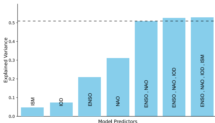
Figure 11. Explained variance by regression models of Gulf SST as a function of predictors. Summer (July-September) SST variance explained by different combinations of climate variability modes. Note that ENSO and NAO together account for more than 50% of the total SST variability. In contrast, the inclusion of IOD and ISM contributes only marginally to the explained variance.
