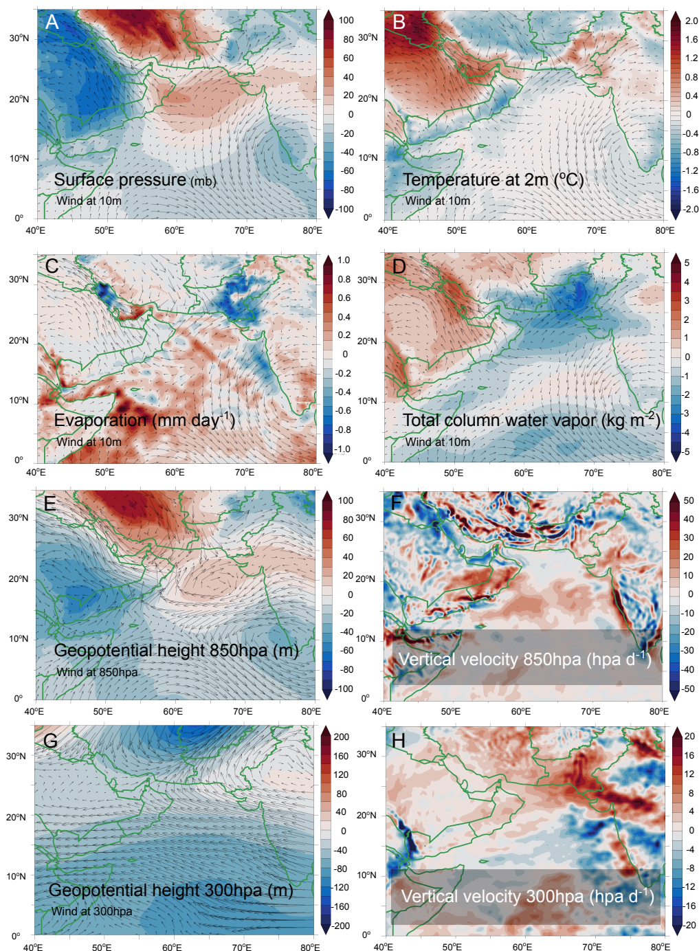
Figure 6. Atmospheric conditions favoring summer marine heatwaves in the Gulf. Composite of atmospheric conditions corresponding to SSTs 1.28 SD above the mean (90th percentile) over 75% of the Gulf. (A) Surface pressure, (B) air temperature at 2 m, (C) evaporation rate, (D) total column water vapor, (E) geopotential height and wind at 850 hPa, (F) vertical velocity at 850 hPa (negative values indicate upward motion), (G) geopotential height and wind at 300 hPa, and (H) vertical velocity at 300 hPa.
