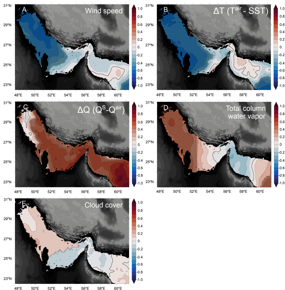
Figure 4. Correlations between SST and meteorological variables over the Gulf. Correlation between SST and wind speed (A), air-sea temperature gradient \Delta T = T^{\text{air}} - \text{SST} (B), air-sea humidity gradient \Delta Q = Q^{\text{S}} - Q^{\text{air}} (C), total column water vapor (D) and cloud cover (E). Hatching indicates statistical significance at 95% confidence interval. T^{\text{air}} and Q^{\text{air}} refer to air temperature and specific humidity at 2m. Q^{\text{S}} is the saturation specific humidity at sea surface.
