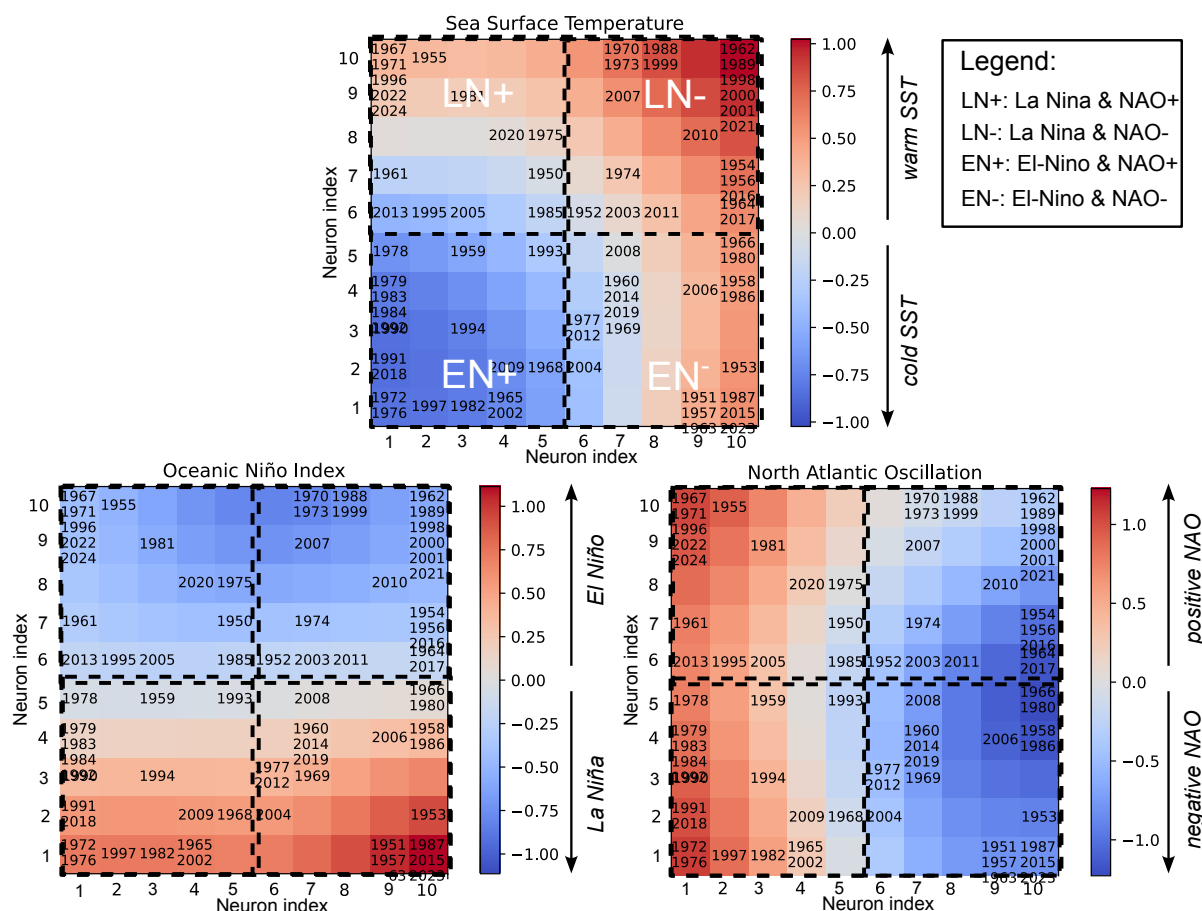
Figure 12. Visualization of Gulf SST links to ENSO and NAO using a Self-Organizing Map (SOM). Component planes of the SOM. Each plane shows the distribution of one variable across the map. Each neuron corresponds to a prototype of Gulf SST regime defined by a given combination of an SST anomaly and the corresponding phases of ENSO and NAO. Note that ENSO and NAO act mostly as two independent variables along which a large fraction of the SST can be explained. The map is divided into 4 quadrants that correspond to 4 regimes: (i) an upper right quadrant with the warmest summers where La Niña coincides with negative NAO, (ii) a lower-left quadrant with the coolest summers where El Niño coincides with positive NAO, and (iii) the upper-left quadrant and lower-right quadrant where La Niña coincides with positive NAO and El Niño coincides with negative NAO, respectively. Individual years are shown associated with their best-matching neurons.
