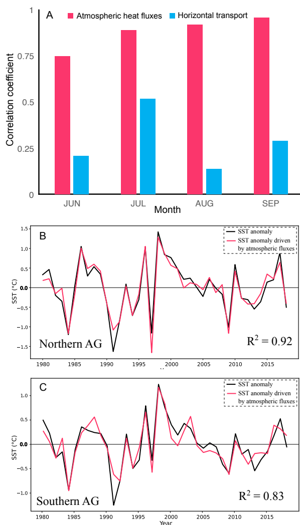
Figure 2. Impact of atmospheric heat fluxes on the Gulf temperature. (A) Pearson correlation coefficients between Gulf SST anomalies and anomalies in atmospheric heat fluxes (red) and heat transport from the Sea of Oman (blue) during summer. Inter-annual summer SST anomaly (black) as a function of time, along with the contribution of atmospheric heat fluxes to the SST anomaly (red), in the northern (B) and southern (C) Gulf. The contribution of heat fluxes is estimated from a linear regression of SST anomalies onto anomalies in the four heat flux components: solar shortwave radiation, downward longwave radiation, latent heat flux, and sensible heat flux.
