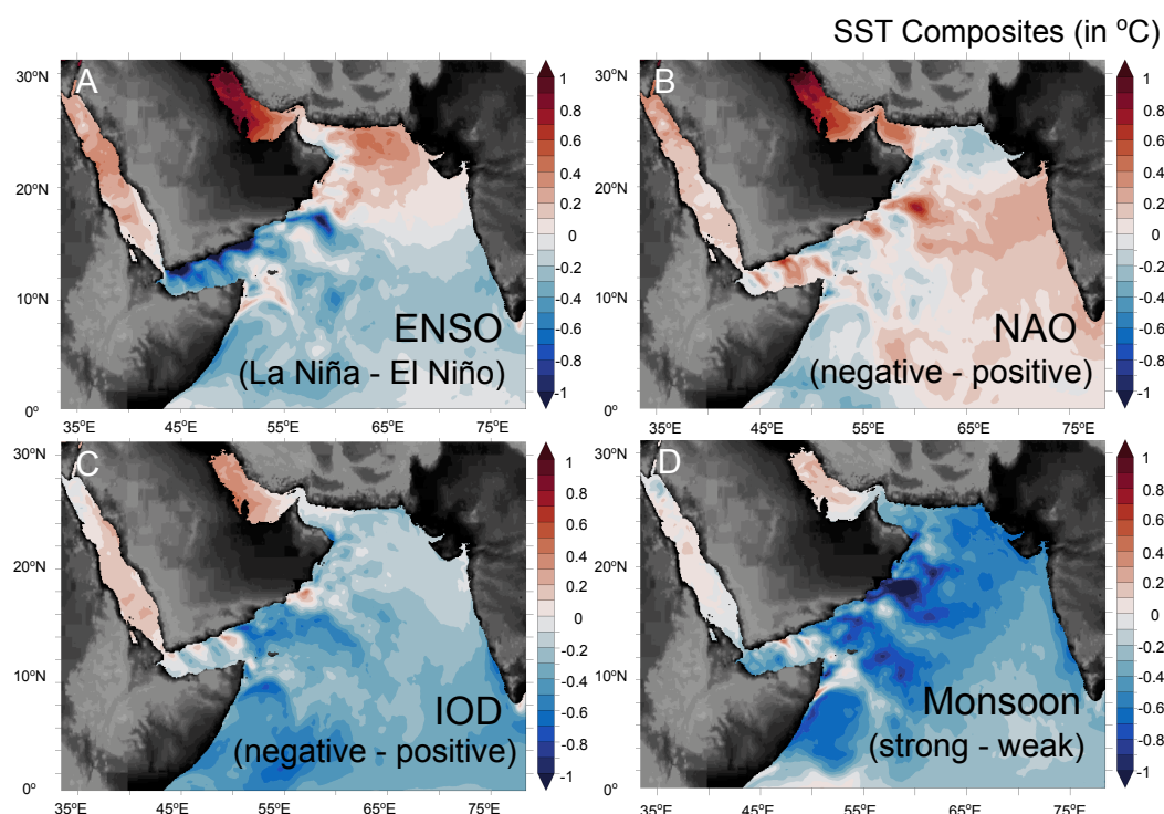
Figure 13. Contrasting impacts of climate teleconnections on SSTs in the Gulf and Arabian Sea. Composite SST anomalies showing the difference between opposite phases of major climate oscillation modes during summer (from left to right and top to bottom: ENSO, NAO, IOD, ISM).
