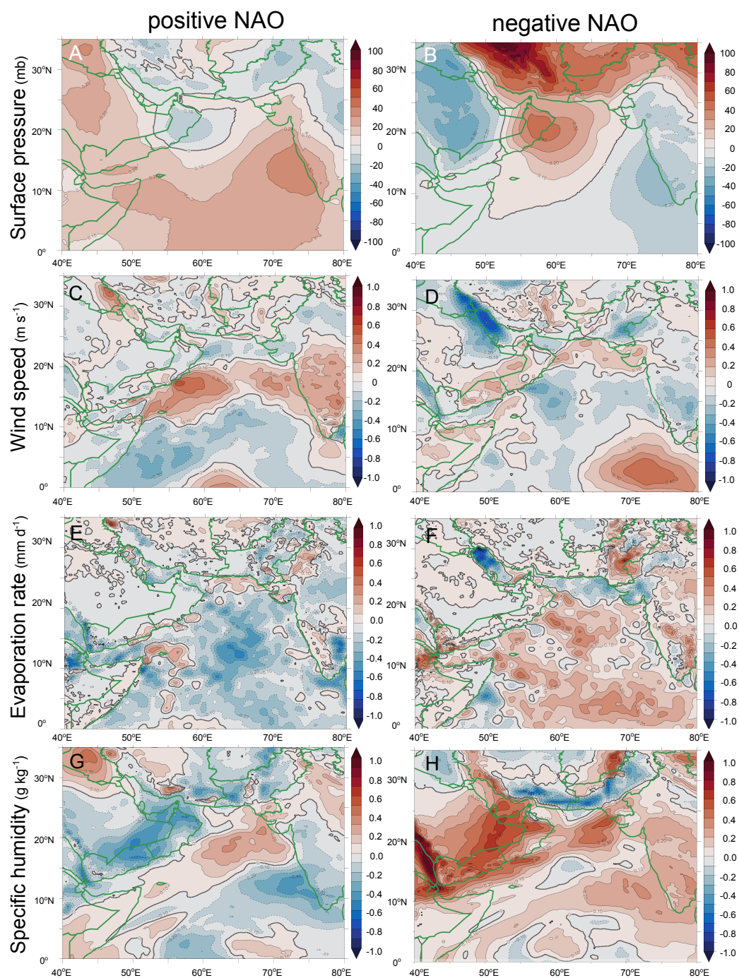
Figure 10. Composite anomalies during NAO. Anomalies in summer atmospheric conditions during positive (left) and negative (right) NAO over the Arabian Peninsula and Arabian Sea region. (A-B) sea level pressure, (C-D) wind speed, (E-F) evaporation rate, (G-H) specific humidity at 850 hpa.
