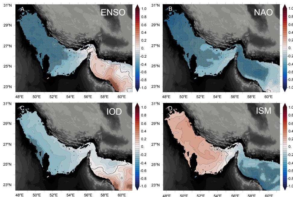
Figure 7. Gulf SSTs and large-scale teleconnections. Zero-lag correlations between Gulf SSTs and major climate oscillation modes in summer (from left to right and top to bottom: ENSO, NAO, IOD, ISM). Hatching indicates statistical significance at 95% confidence interval.
