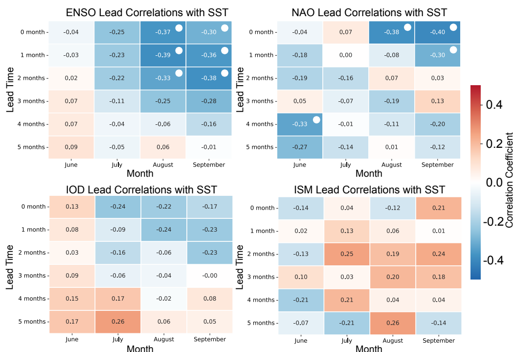
Figure 8. Lead-lag correlations between major climate variability modes and Gulf SST. Lead-lag correlations between ENSO (top-left), NAO (top-right), IOD (bottom-left) and ISM (bottom-right) and Gulf SST during summer months. Statistically significant correlations at 95% confidence interval are marked with white filled circles.
