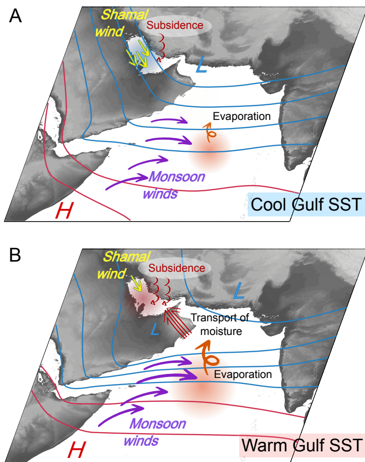
Figure 14. Illustration of atmospheric conditions causing cool and warm SSTs in the Gulf during summer. Schematic illustration of atmospheric conditions favoring cool (A) and warm (B) SSTs in the Gulf. Lower (higher) pressure over the Arabian Peninsula and higher (lower) pressure over Iran/Pakistan are associated with stronger (weaker) monsoon winds over the Arabian Sea, weaker (stronger) Shamal winds over the Gulf and stronger subsidence in the higher troposphere. These conditions lead to enhanced (reduced) evaporation over the Arabian Sea, increased (reduced) air moisture transport to the Gulf region, reduced (enhanced) evaporation over the Gulf and increased (reduced) retention of air moisture near the surface. Consequently, these changes enhance (reduce) heat trapping near the surface and weaken (increase) evaporative cooling at the surface.
