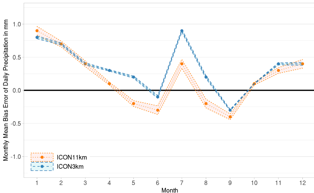
Fig. S4: Monthly mean bias error of daily precipitation of ICON3km and ICON11km during the period 2005 to 2014, as well as the 95%-confidence intervals from the station means
