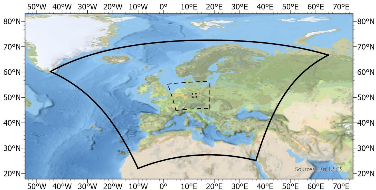
Fig. S3: RCM EURO-domain (solid) and CPRCM CEU-domain (dashed), together with the edges of the study area (points) (sources: ESRI, USGS)
