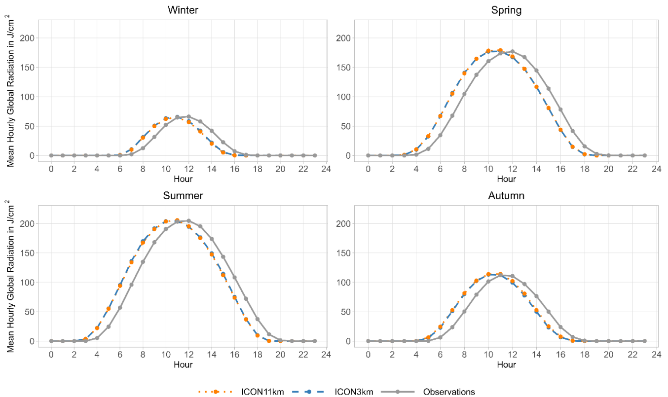
Fig. 3: Seasonal diurnal cycles of mean hourly global radiation computed by ICON11km and ICON3km, as well as the observations for the study area for the period from 2005 to 2014
