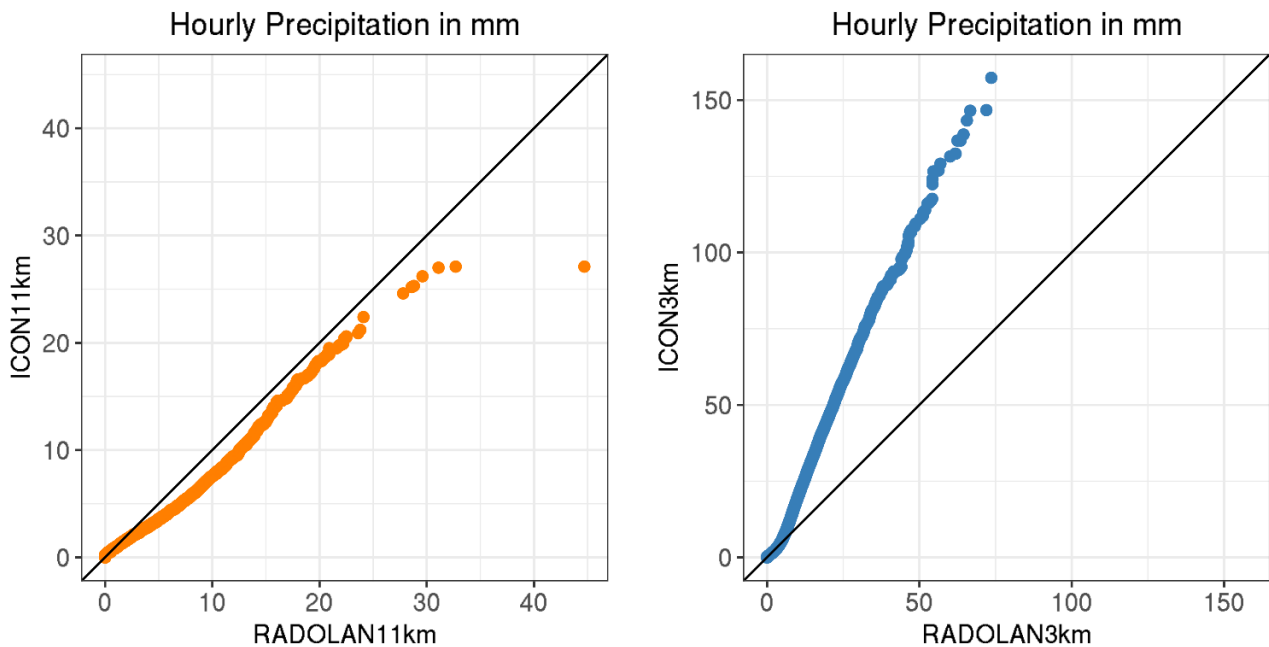
310 Fig. 6: QQ-plots for hourly precipitation for the period from 2005 to 2014 for ICON11km to RADOLAN11km (left) and ICON3km to RADOLAN3km (right)
