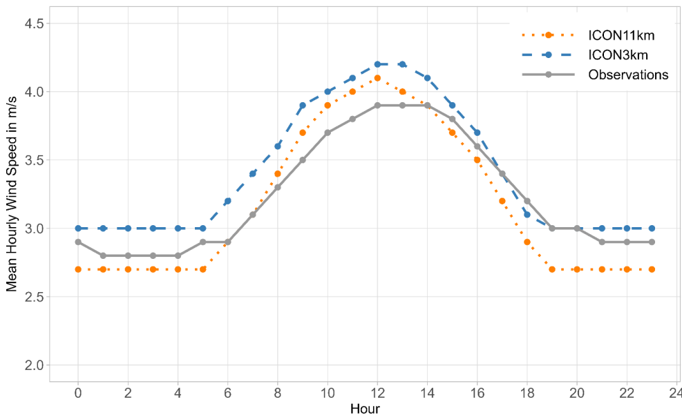
Fig. 5: Diurnal cycle of mean hourly wind speed computed by ICON11km and ICON3km, as well as the observations for the study area for the period from 2005 to 2014
