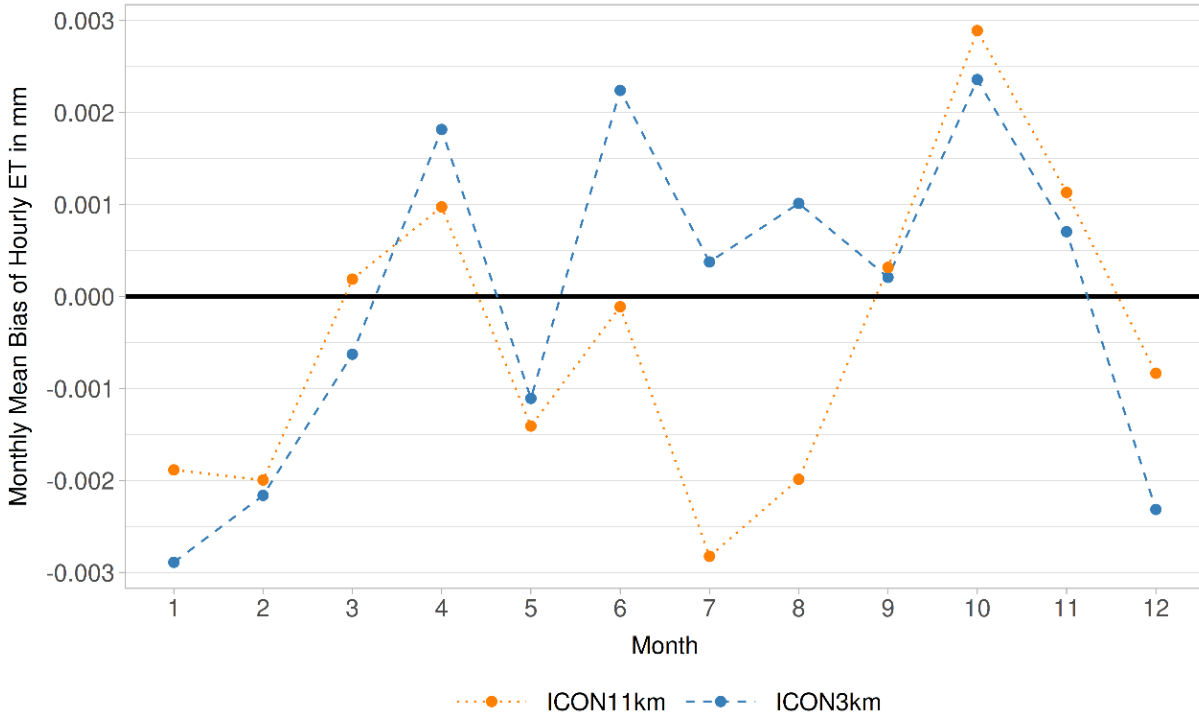
Fig. 11: Monthly mean bias of hourly total evapotranspiration, as calculated by the hydrological model driven with ICON3km and ICON11km for the period from 2006 to 2014
