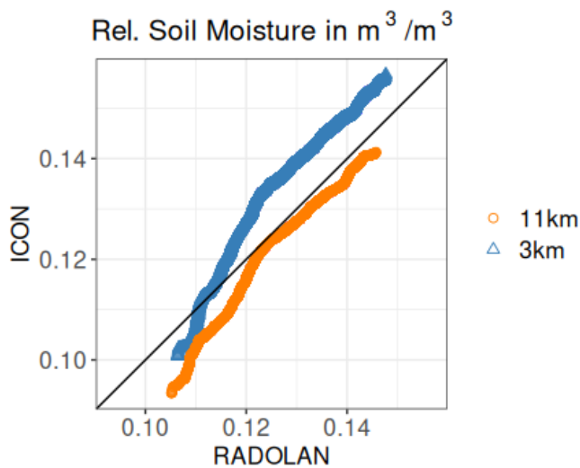
Fig. 10: QQ-plots for hourly soil moisture for the period from 2006 to 2014 for ICON11km to RADOLAN11km and ICON3km to RADOLAN3km
