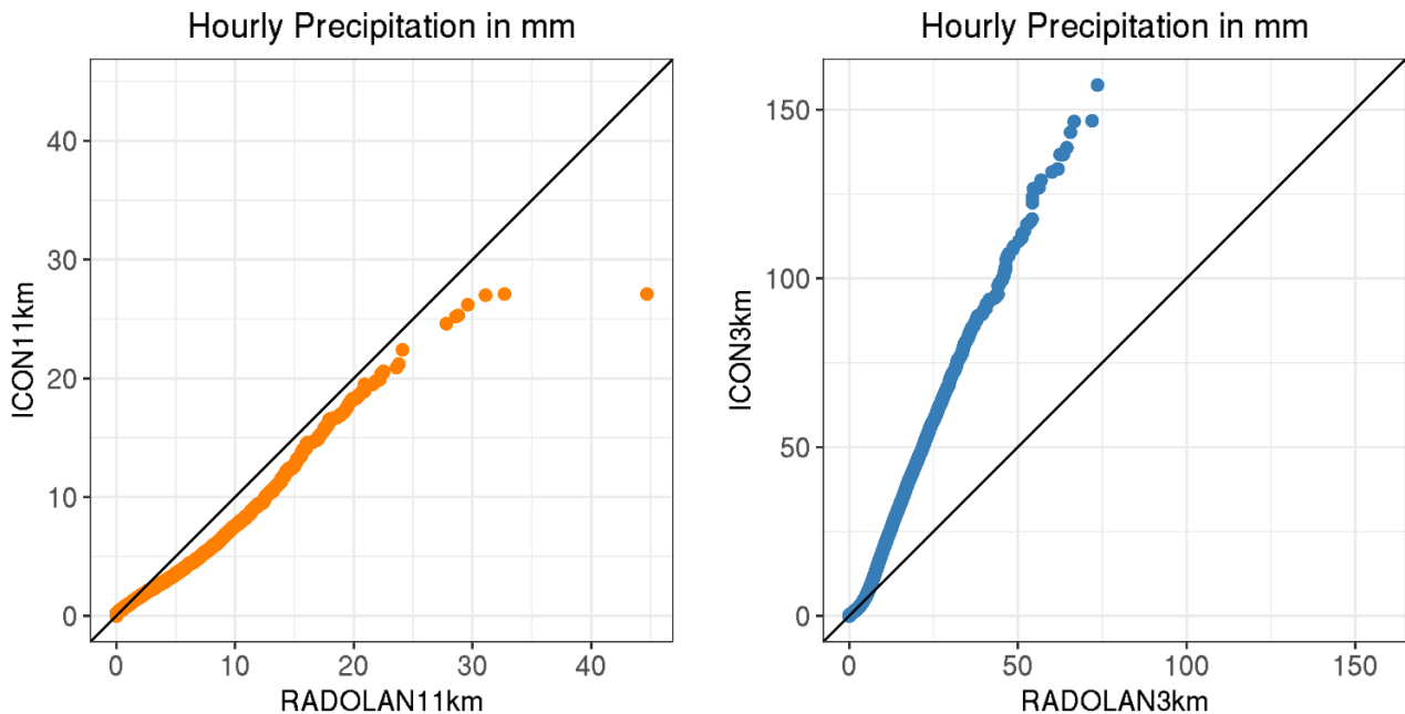
Fig. 6: QQ-plots for hourly precipitation for the period from 2005 to 2014 for ICON11km to RADOLAN11km (left) and ICON3km to RADOLAN3km (right)
