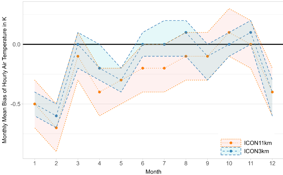
225 Fig. 2: Monthly mean bias of hourly air temperature of ICON3km and ICON11km for the period from 2005 to 2014, as well as the 95%-confidence intervals from the station means
