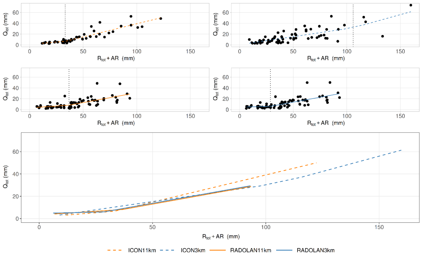
Fig. 14: Upper half: Scatter plots of total runoff ( Q_{tot} ) to the sum of total rainfall ( R_{tot} ) and 8-h antecedent rainfall (AR) over the catchment of Kleindalzig and those upstream, fitted with a piecewise linear regression model. The thresholds are indicated with a dotted vertical line. Lower half: Combined piecewise linear regression model results of Q_{tot} to R_{tot} + AR
