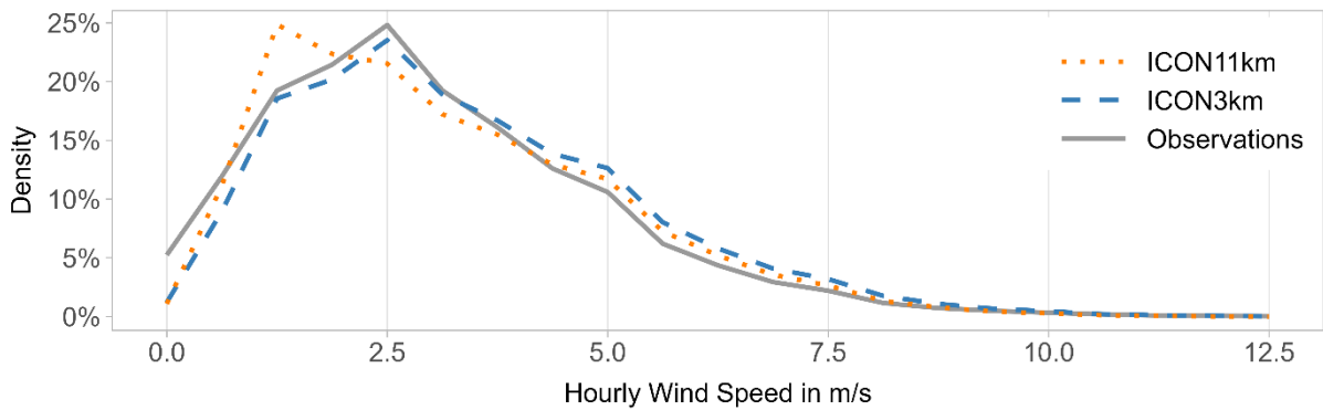
280 Fig. 4: Frequency polygons for hourly wind speed as observed, and calculated by ICON3km and ICON11km over the study area for the period from 2005 to 2014
