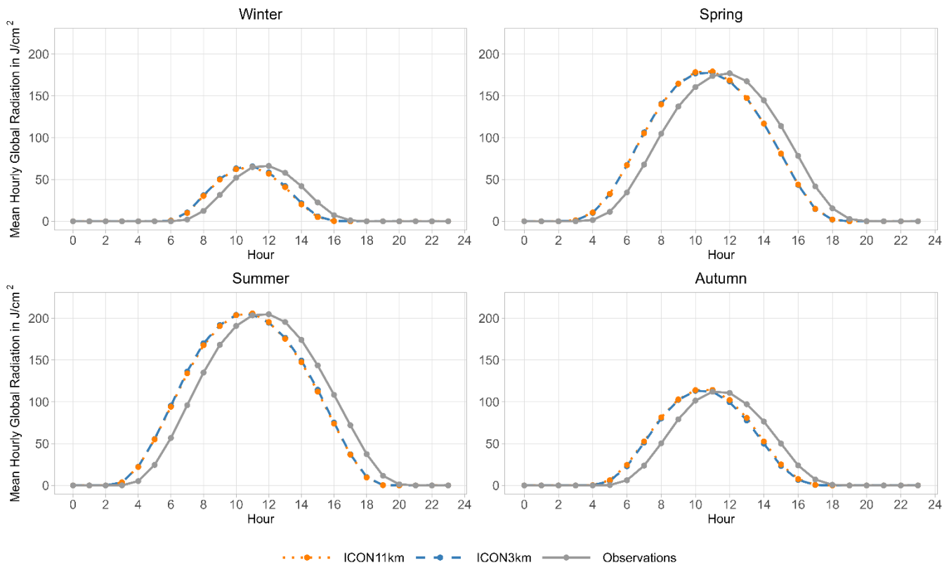
250 Fig. 3: Seasonal diurnal cycles of mean hourly global radiation computed by ICON11km and ICON3km, as well as the observations for the study area for the period from 2005 to 2014
