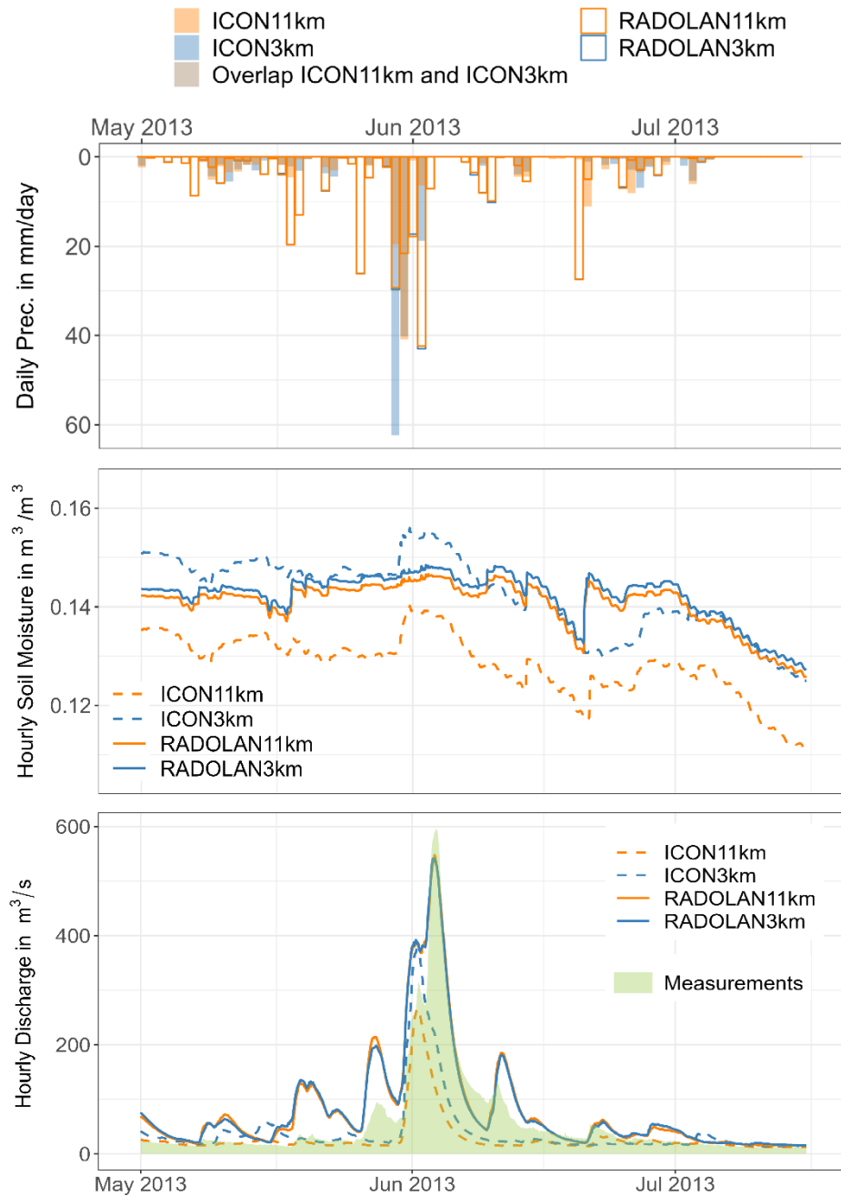
465 Fig. 15: Top: Daily spatial average precipitation estimates over the catchment of Zeitz and those upstream for the period of the 2013 flood for ICON11km, ICON3km, RADOLAN11km and RADOLAN3km, Centre: the respective hourly relative soil moisture spatial averages gained from continuous simulation, Bottom: the resulting hydrographs (using hourly data) for the catchment of Zeitz together with the discharge measurements
