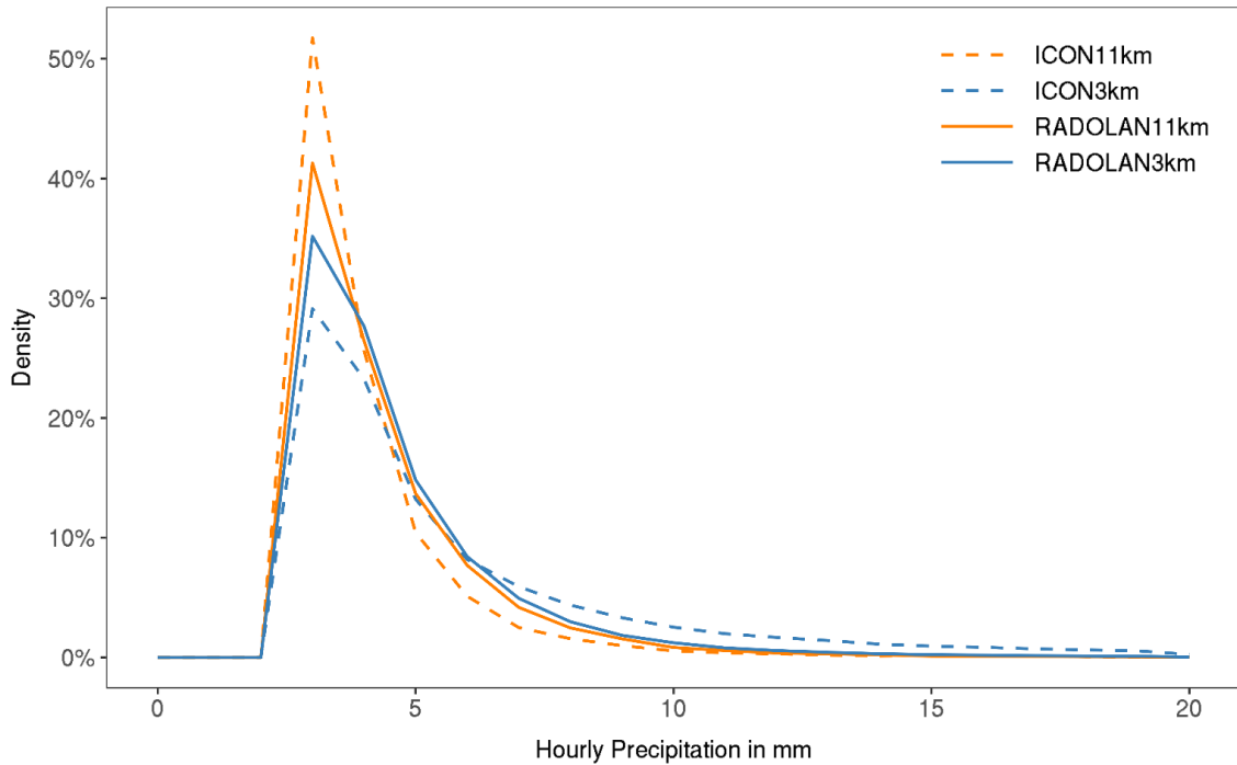
Fig. 7: Frequency polygons for ICON11km, ICON3km, RADOLAN11km and RADOLAN3km for the 99.5th-percentile of hourly precipitation for the period from 2005 to 2014
