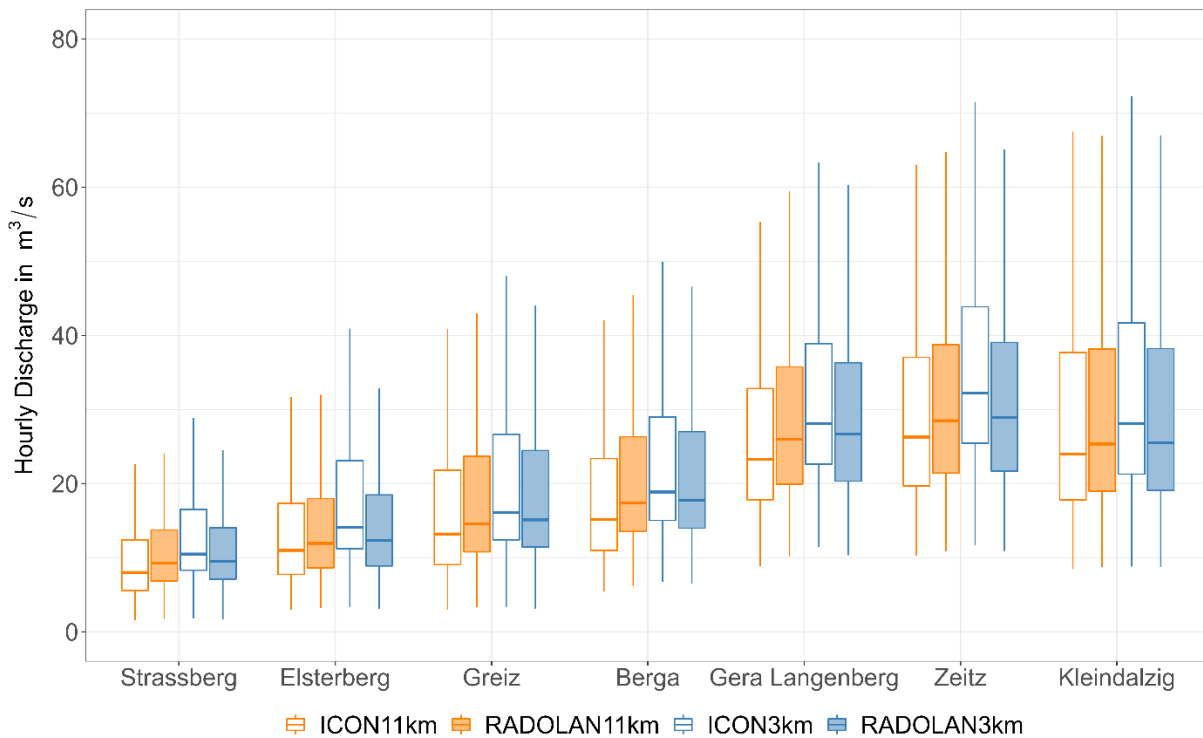
420 Fig. 12: Boxplots of hourly discharge (period from 2006 to 2014) computed by the WaSiM hydrological model driven with meteorological data from ICON11km and ICON3km, as well as with adjusted radar data of respective equal resolution (RADOLAN11km and RADOLAN3km) for catchments of the main stem of the Weiße Elster river within the study area. Values beyond the whiskers are not represented.
