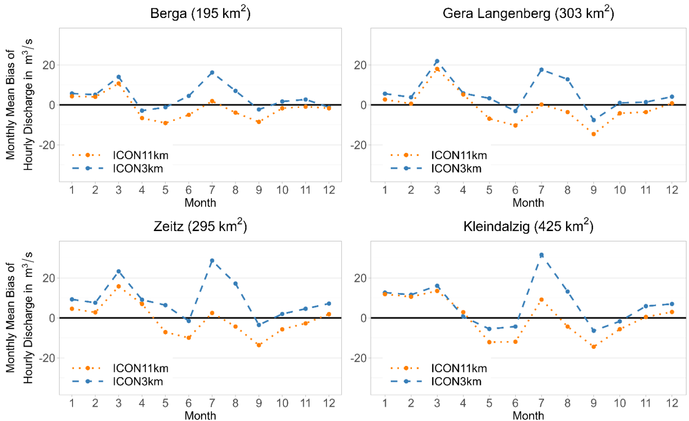
435 Fig. 13: Monthly mean bias of hourly discharge from the hydrological model driven with ICON11km/ ICON3km meteorological data compared to when driven with adjusted radar data of equal resolution (RADOLAN11km/ RADOLAN3km) for the four most downstream catchments on the main stem of the Weiße Elster river within the study area for the period from 2006 to 2014
