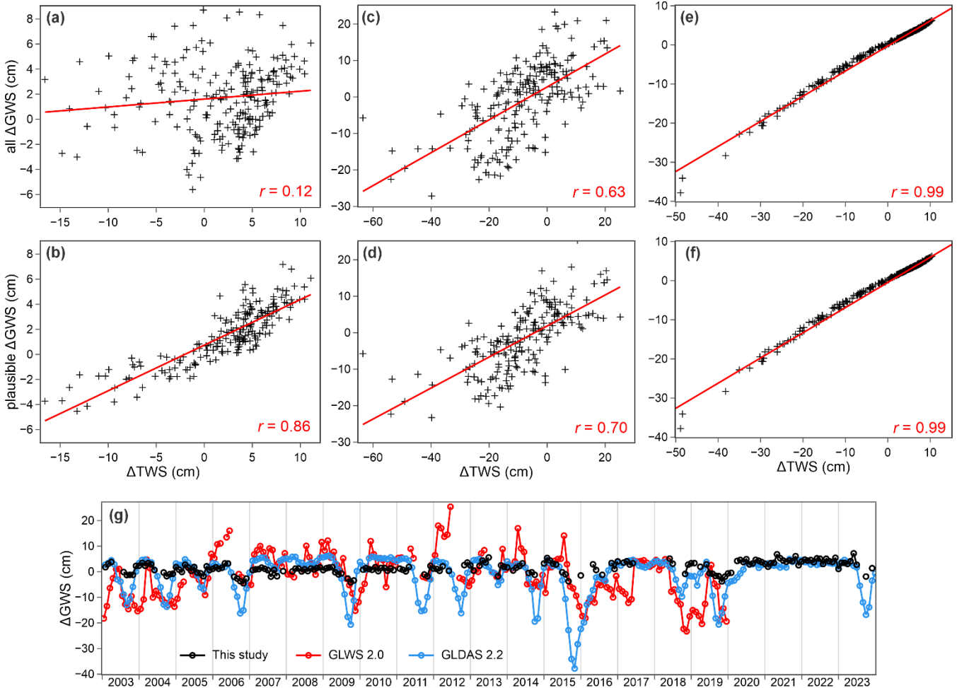
Figure 6: Cross-correlations between ensemble mean \Delta TWS and \Delta GWS from (a, b) this study, (c, d) the GLWS dataset, and (e, f) the GLDAS dataset with and without implausible estimates; (g) comparison of \Delta GWS from this study and GLWS.
