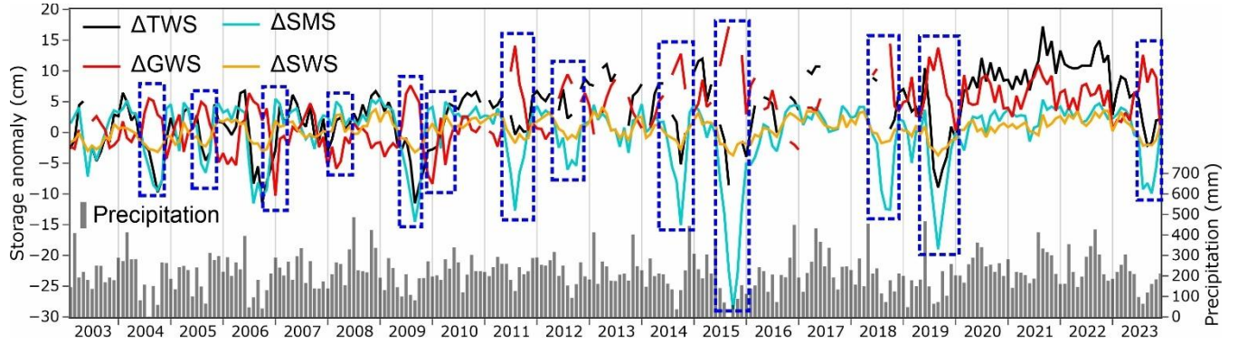
Figure 4: Comparison between mean \Delta TWS (GRACE JPL 0.5°), \Delta SMS (Noah LSM), \Delta SWS (WGHM), and computed \Delta GWS . Blue dashed polygons indicate arithmetic problems resulting from \Delta SMS values being significantly lower than \Delta TWS .
