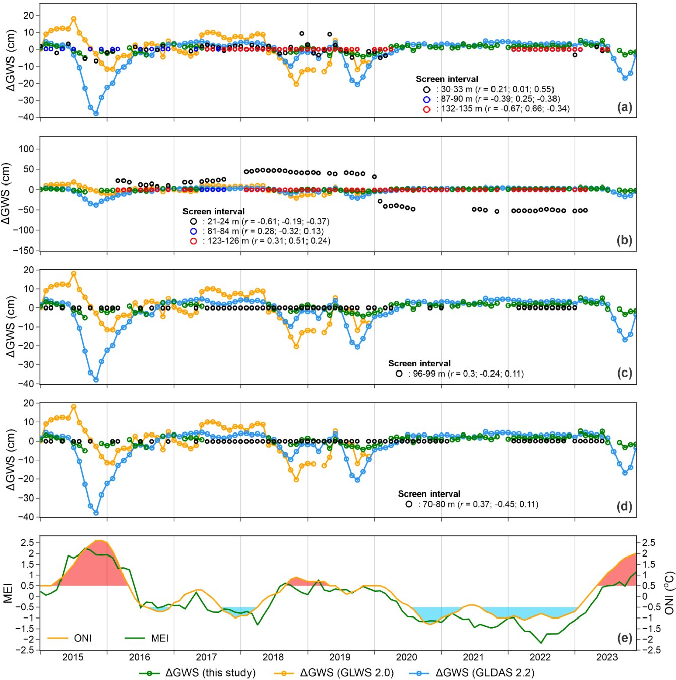
540 Figure 8: Comparison between \Delta GWS from piezometers (black, dark blue, and red circles) at (a) MG, (b) MM, (c) GM, and (d) TS sites with GRACE-derived \Delta GWS (green, orange, and light blue circle-line); (e) MEI (green line) and ONI (orange line) indices. All
