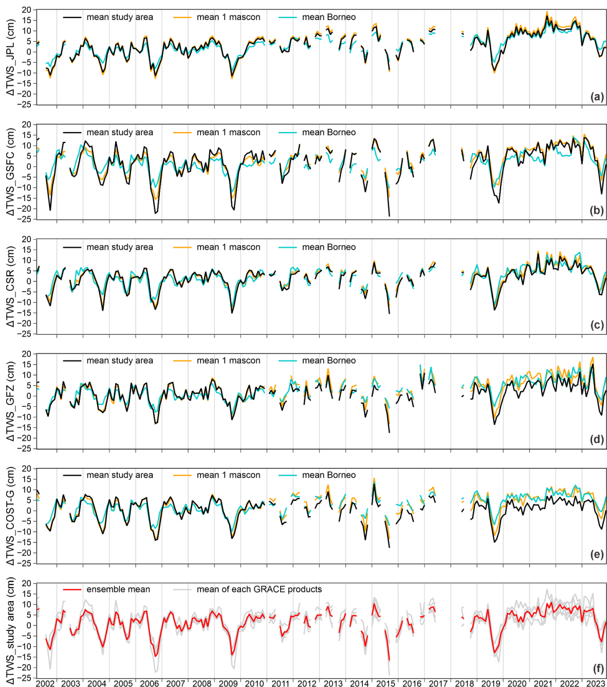
Figure 2: Comparison of mean \Delta TWS values from different GRACE datasets: (a) JPL, (b) GSFC, (c) CSR, (d) GFZ, and (e) COST-G. In (a) to (e), the black, orange, and blue lines represent \Delta TWS for the study area, a single 3 rd mascon, and the entire Borneo, respectively. Plot (f) shows the ensemble mean \Delta TWS of the study area (red line) derived from the five GRACE datasets (gray lines). Missing \Delta TWS data are indicated by gaps in the dataset.
