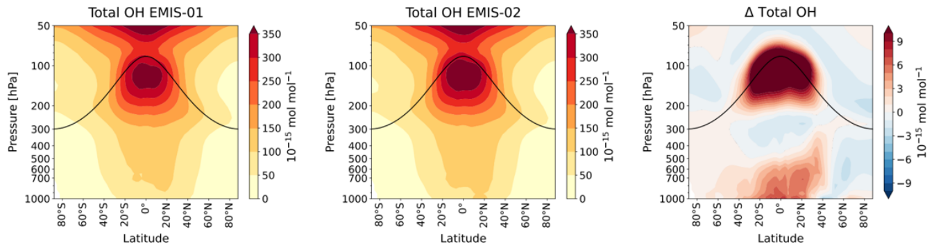
Figure 5. Multi-annual (2000–2010), zonally averaged OH volume mixing ratio [ 10^{-15} mol mol ^{-1} ] and the absolute differences between EMIS-01 and EMIS-02 simulation results.
