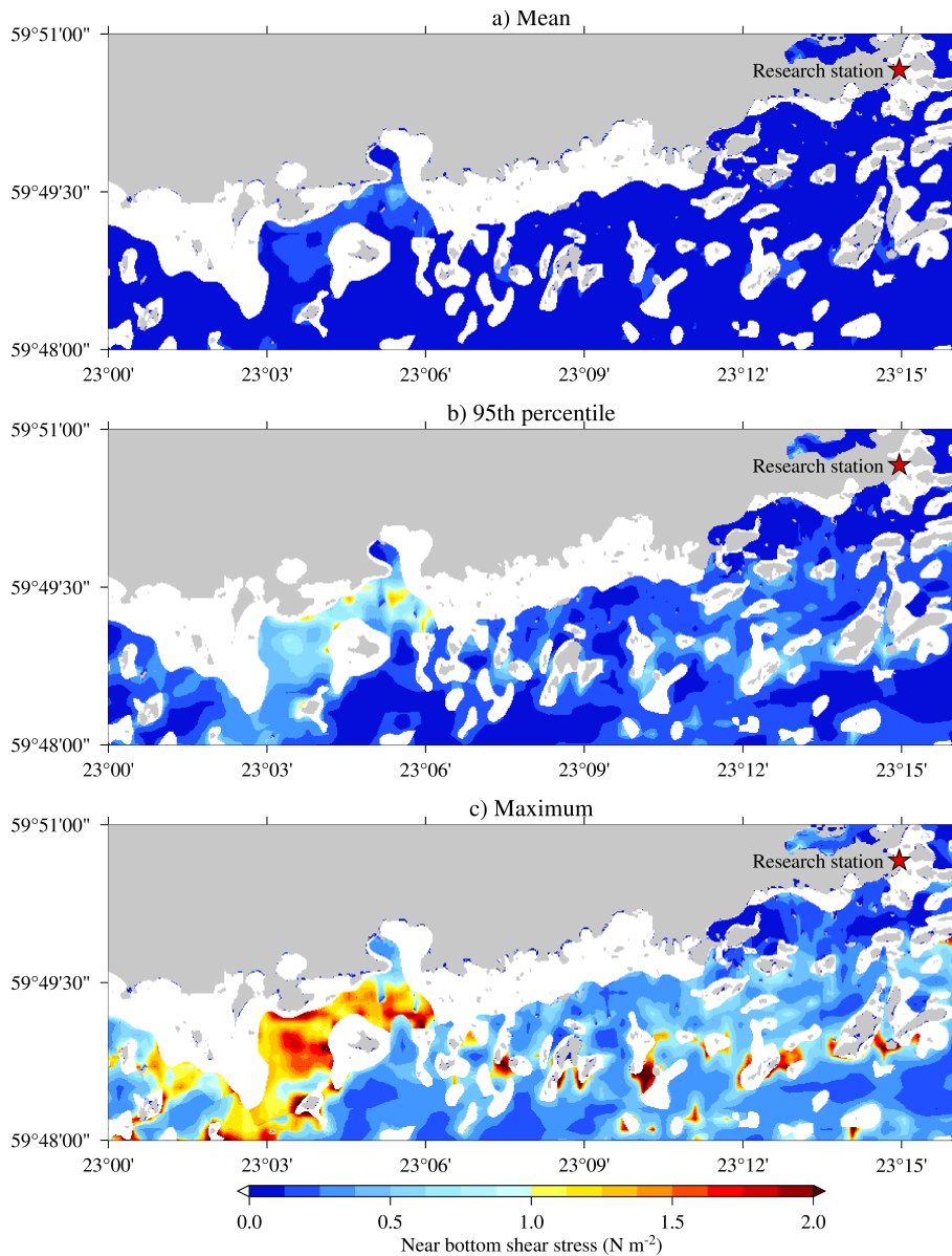
Figure 6. The mean (a), 95 th percentile (b), and maximum values (c) of the modelled near-bottom shear stress for all covering the available model data—modelled time periods in 2014, 2015 and 2017. No results are available for classes Boulders and Coarse sediments (white), since no measurements were available from those classes to determine representative grain sizes. The red star marks the Tvärminne research station for reference.
