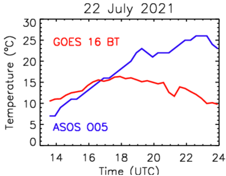
Figure 4. ASOS station O05 temperature and GOES 16 window BT time series, daytime 22 July. The ASOS data (blue line) are the same as in S24’s Figure 6. Red line, BT for the GOES pixel (at 40.282°N, 121.241°W) closest to O05 (40.2824°N, 121.241°W) location..
