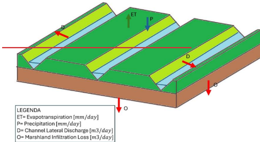
Figure 3: WetMAT model scheme for the Doñana case study, with evapotranspiration (ET) and precipitation (P) as main fluxes, small losses due to infiltration (O) and the Channel Lateral Discharge (D) affecting the marshland flooding process.
