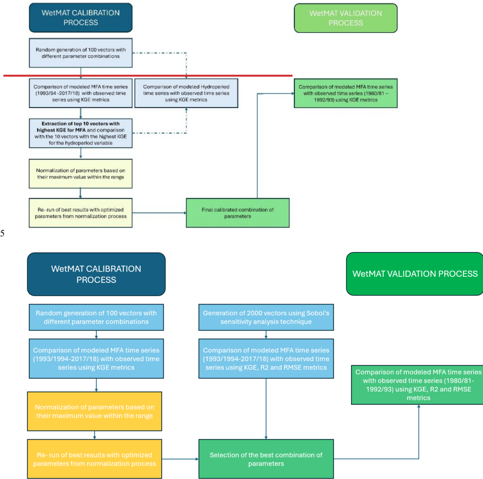
Figure 5: Main steps involved in the calibration and validation processes of the WetMAT model.
