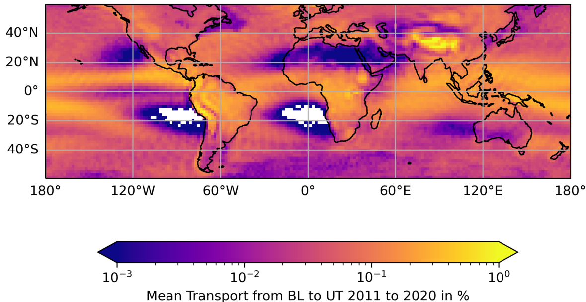
Figure 8. Ten-year (2011 to 2020) mean convective mean transport from the planetary boundary layer height to upper-troposphere-UT within 12 min. The upper-troposphere-UT is defined as the vertical region between the tropopause and the height of tropopause in hPa plus 150 hPa.
