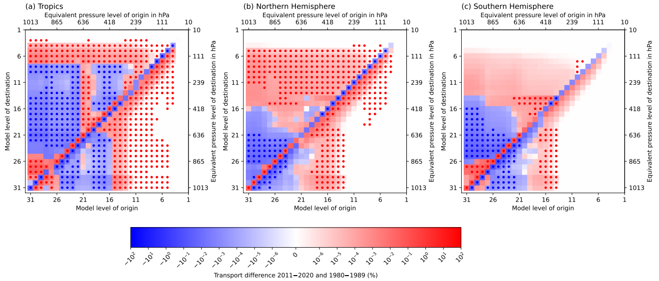
Figure 7. Changes in the convective mean transport in different regions. Same as Fig. ?? but (a) for 30°S and to 30°N, (b) for 60°N to 30°N and (c) for 60°S to 30°S.
