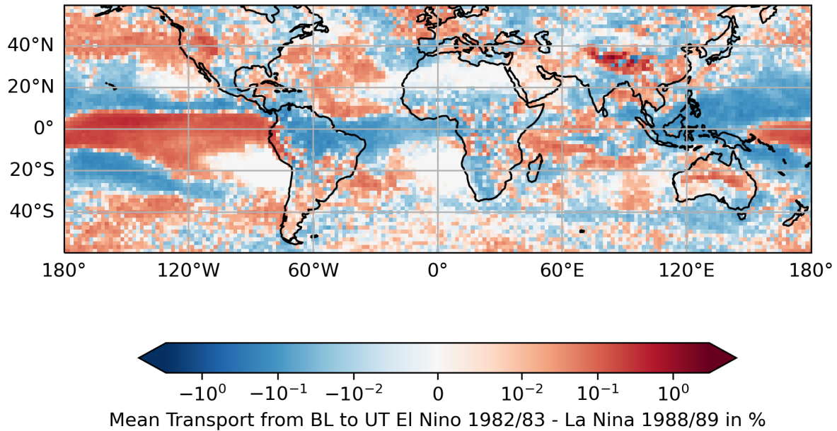
Figure 10. As Fig. ?? but for the difference between the El Niño event 1982/83 and the La Niña event 1988/89.
