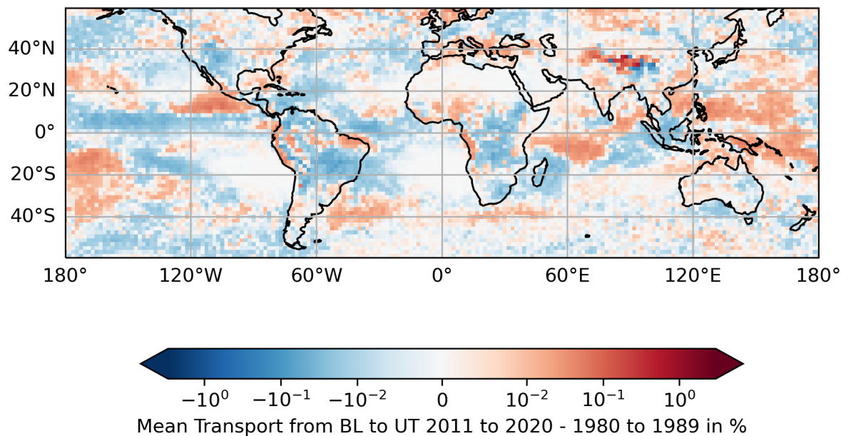
Figure 9. As Fig. ?? but for the difference of the mean values of 2011 to 2020 and 1980 to 1989.
