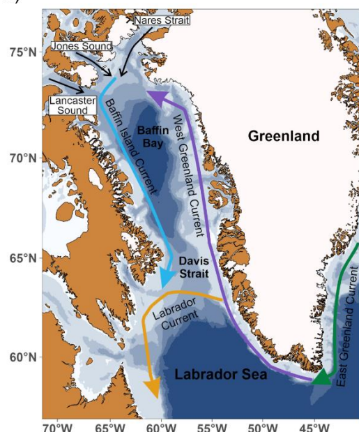
Figure 1: a) Schematic overview of the ocean currents and bathymetry in Baffin Bay and Davis Strait. Colored lines with arrows indicate the direction of different ocean currents. Bathymetry data from the GEBCO 2023 grid (GEBCO Bathymetric Compilation Group 2023). b) Map of the study area during DANA 6/21 with red points indicating the sampling locations and their affiliation to a certain transect (1-5).
