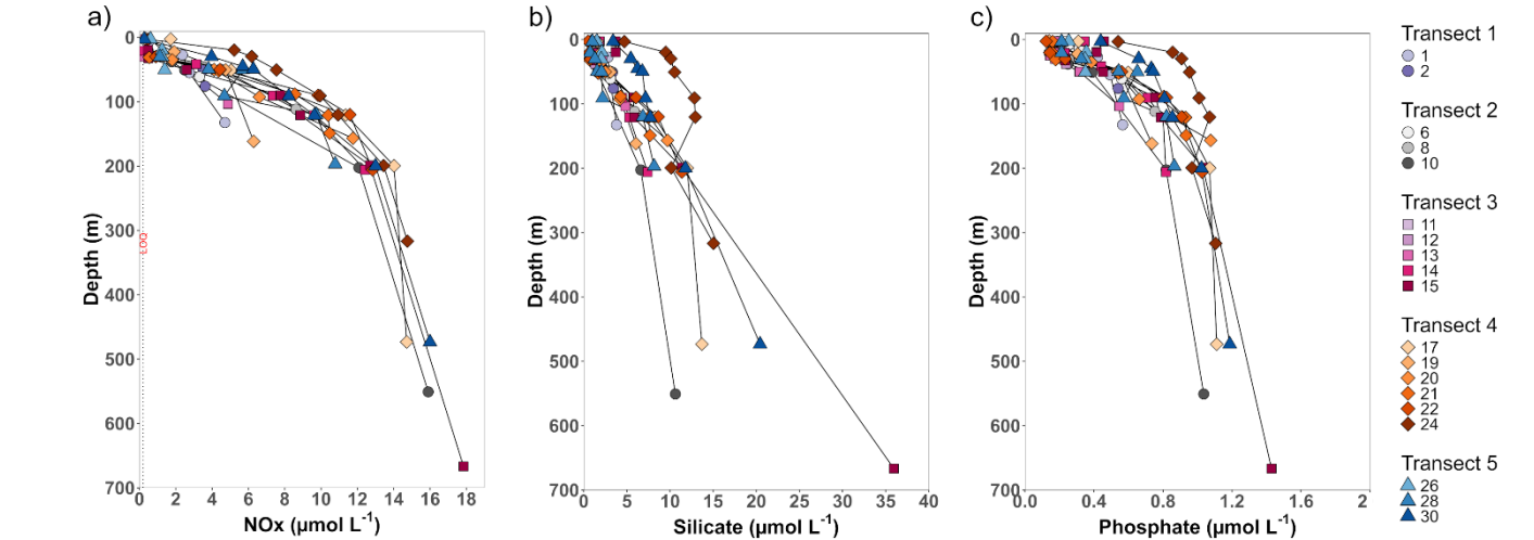
250 Figure 3 Vertical profiles of nutrient concentrations across the study area. Each data point is identified by shape (transect number) and color (station number).
