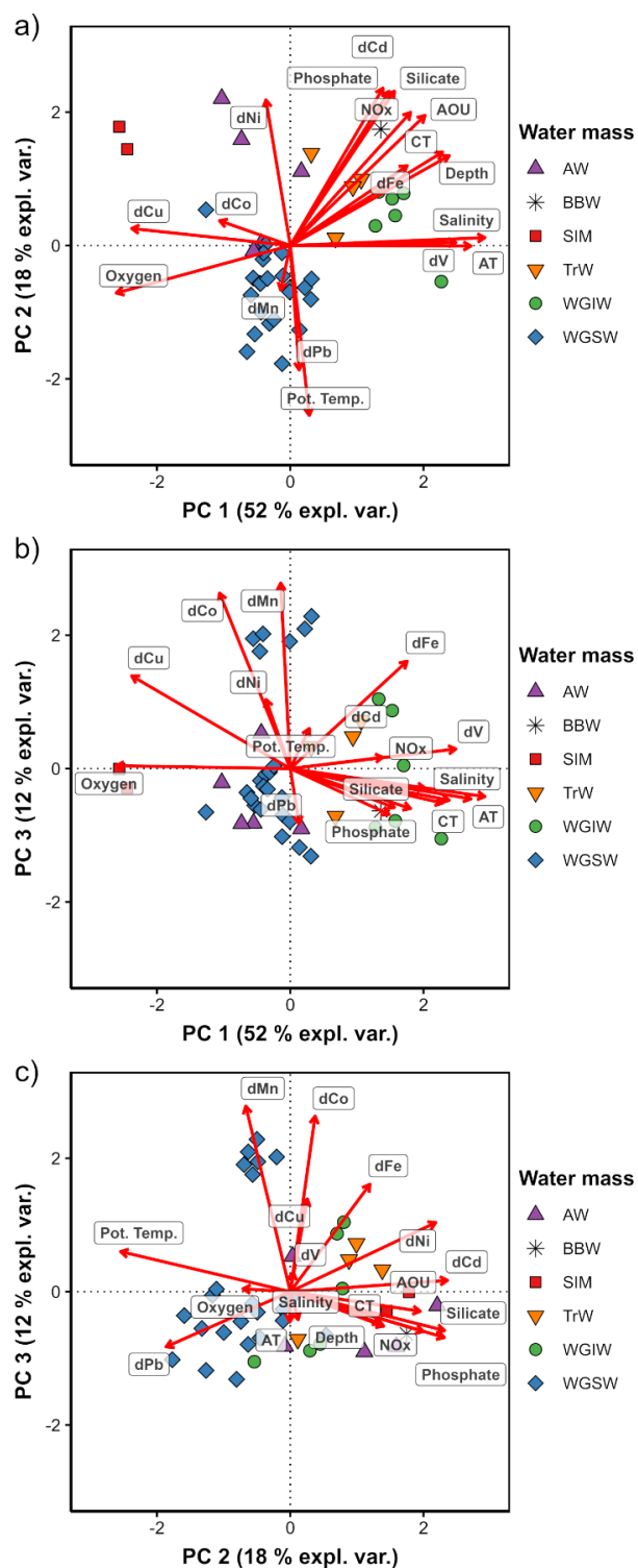
355 Figure 7: Biplots according to PCA results for a) PC 1 score vs PC 2 score; b) PC 1 score vs PC 3 score; and c) PC 2 score vs PC 3 score, with colors indicating the water mass affiliation of each sample. The loading of each parameter is indicated by a red arrow.
