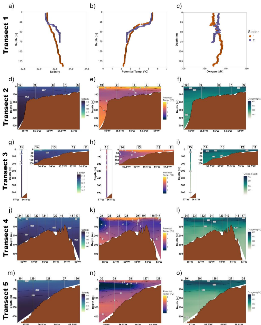
210 Figure 2: Water depth profiles illustrating the spatial distribution of salinity, potential temperature, and oxygen along transect 1 (a-c), transect 2 (d-f), transect 3 (g-i), transect 4 (j-l), and transect 5 (m-o). For transect 1, data are not shown as interpolated profiles due to limited data availability. For transect 3, station 15 is displayed separately because of its southerly location (refer to Fig. 1 b).
