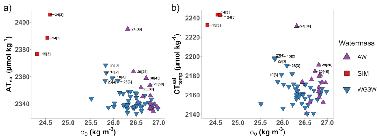
585 Figure 10: First 50 m of the water column for a) salinity-normalized AT values against pot. density and b) temperature-salinity-normalized CT values against pot. density. Different water mass categories are given in the legend. SIM affected stations (14, 15, 24) and stations adjacent to those (10, 13, 23, 28, 29, 30) are labeled. The number in brackets corresponds to the sampling depth.
