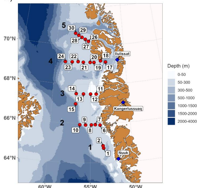
Figure 1: a) Schematic overview of the ocean currents and bathymetry in Baffin Bay and Davis Strait. Colored lines with arrows indicate the direction of different ocean currents. Bathymetry data from the GEBCO 2023 grid (GEBCO Bathymetric Compilation Group 2023). b) Map of the study area during DANA 6/21 with red points indicating the sampling locations and their affiliation to a certain transect (1-5).
