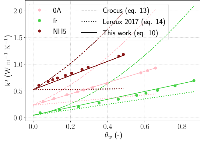
Figure 13. Comparison of the proposed regression of thermal conductivity of dry and wet snow with the regression of Crocus adapted from Yen (1981) extended for wet snow and the one proposed by Leroux and Pomeroy (2017), for three different snow samples.
