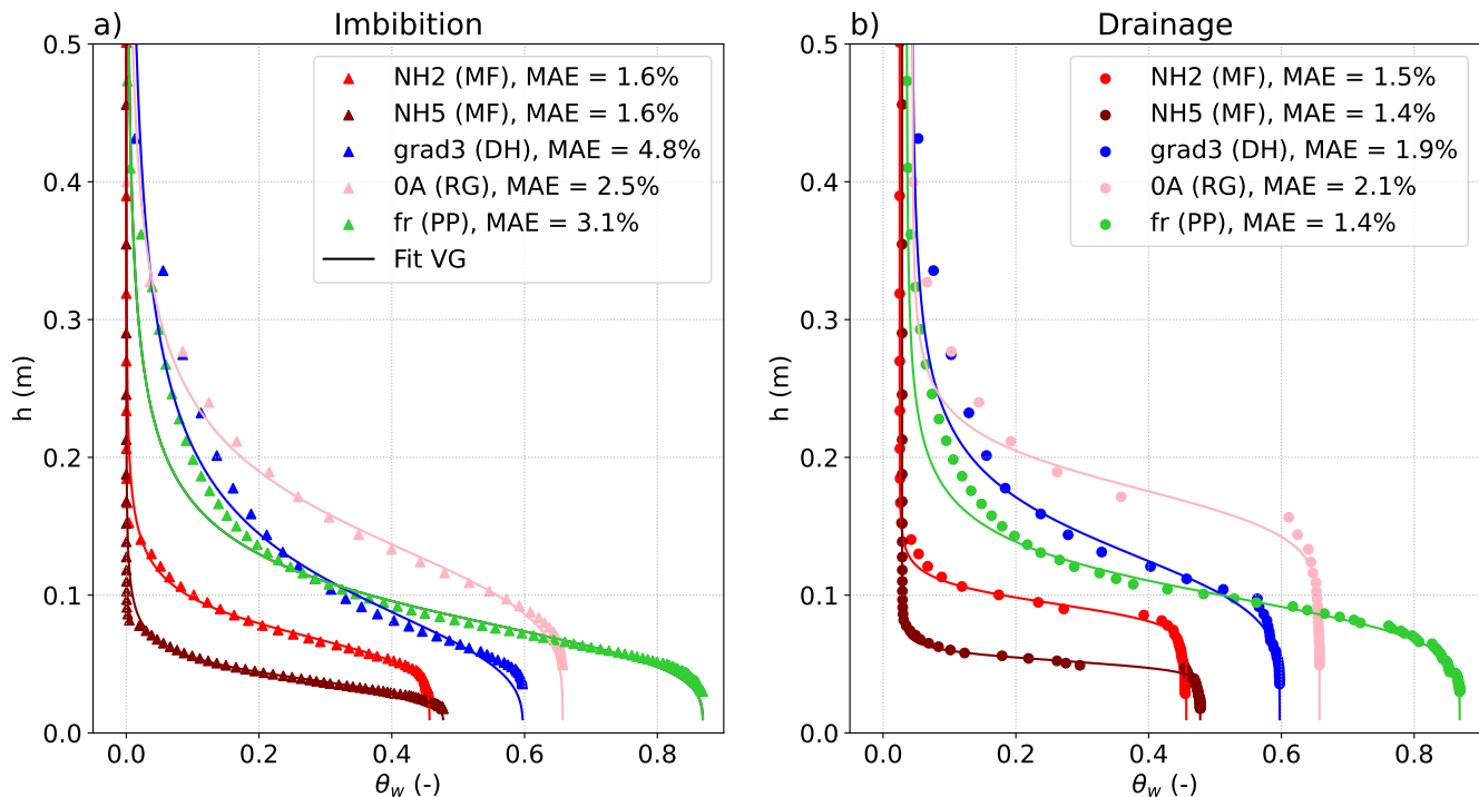
Figure 6. Numerical imbibition and drainage WRCs for different types of snow samples with the corresponding VG fits. The curve colors represent the different snow types, the MAE . The MAEs on \theta_w of the fits are expressed in percent.
