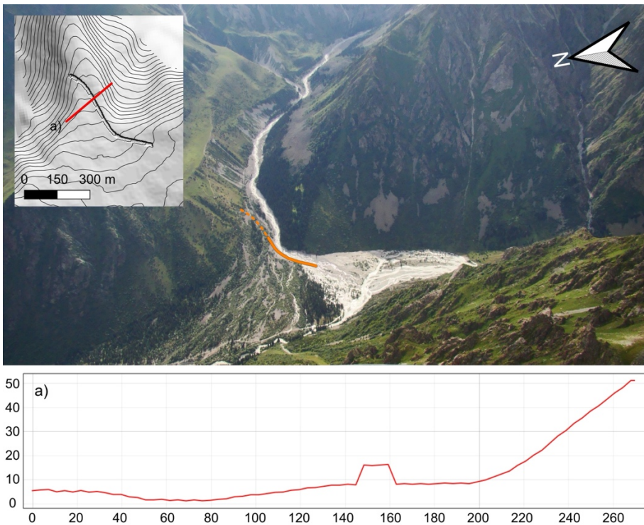
Figure 4: Photograph of the Aksay fan with the position of the existing deflection dam as of 2024 (solid orange line) and the enhanced deflection dam (dashed orange line). Top left box: Hillshade of the artificially modified DEM produced for the RAMMS simulation of the DRM measure. Bottom box: Profile across the river bed and the artificially enhanced deflection dam. Photograph: V. Zaginaev, 2015.
