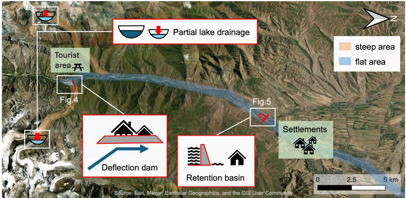
120 Figure 3: Schematic overview of the Ala-Archa valley with the location of the different DRM measures consisting of i) lake level lowering, ii) a deflection dam (reference to Fig. 4), and iii) a retention basin (reference to Fig. 5).
